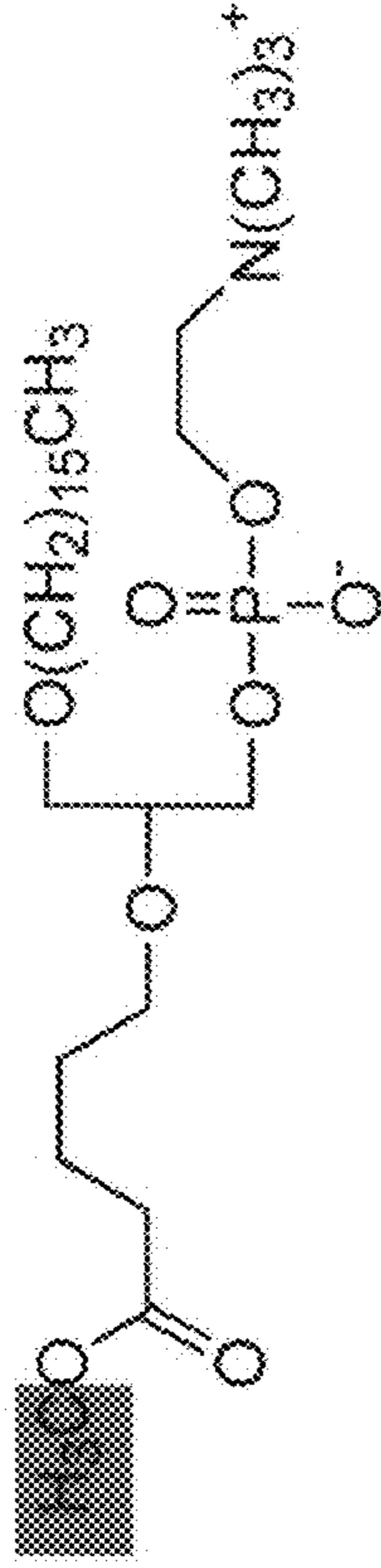
1-O-hexadecyl-2-(4'-carboxymethylester)-butyl-sn-glycero-3-phosphocholine (Methyl ester of Cl-201)
