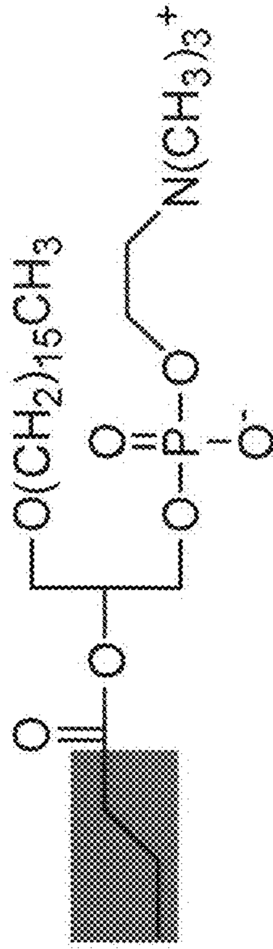
1-O-Hexadecyl-2-O-Butyroyl-sn-Glycero-3-Phosphocholine (PAF-2C)
