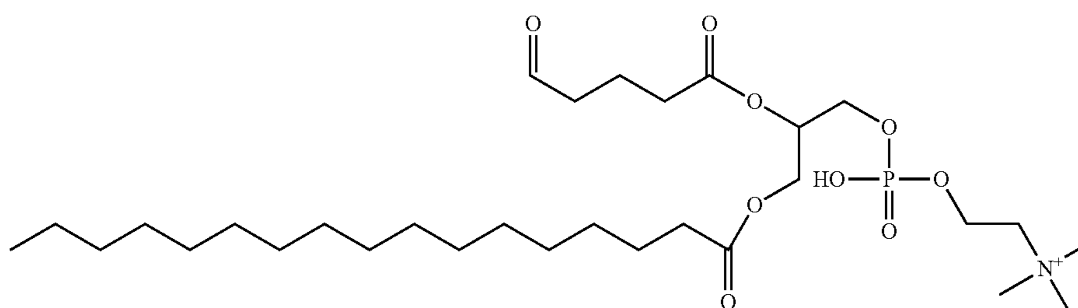
1-hexadecyl-2-(5'-oxo-pentanyl)-sn-glycero-3-phosphocholine
