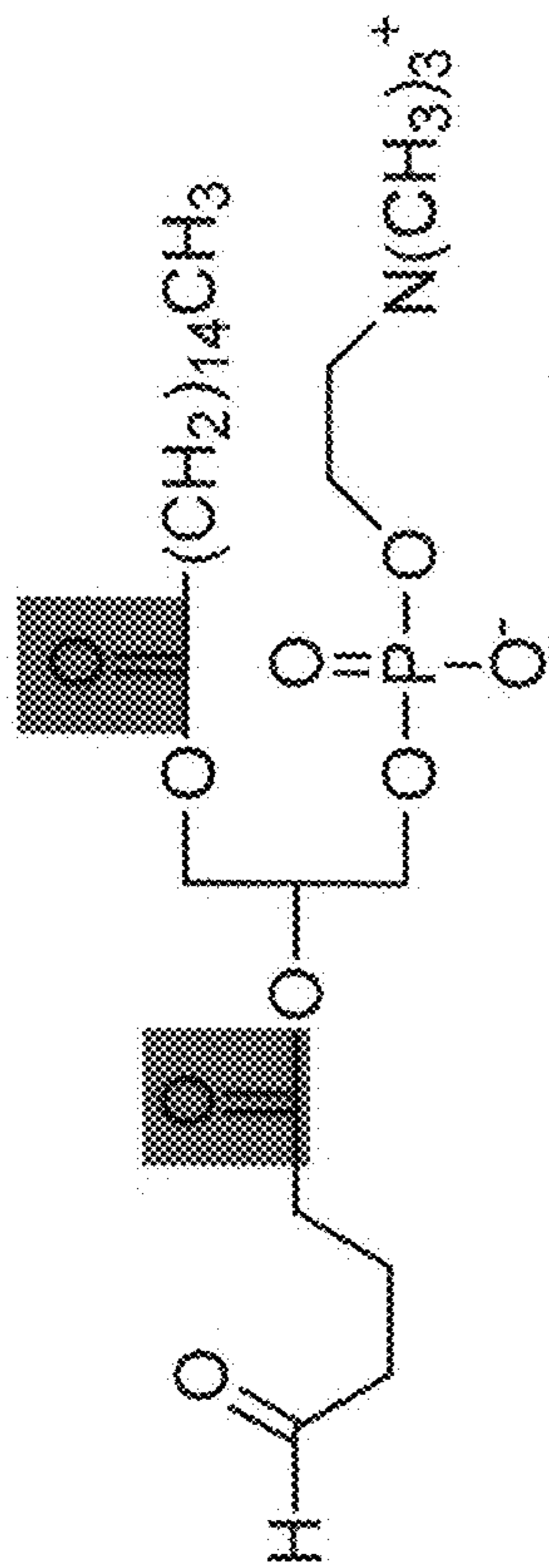
1-Palmitoyl-2-(5'-oxo-Valeroyl)-sn-Glycero-3-Phosphocholine (POVPC)
