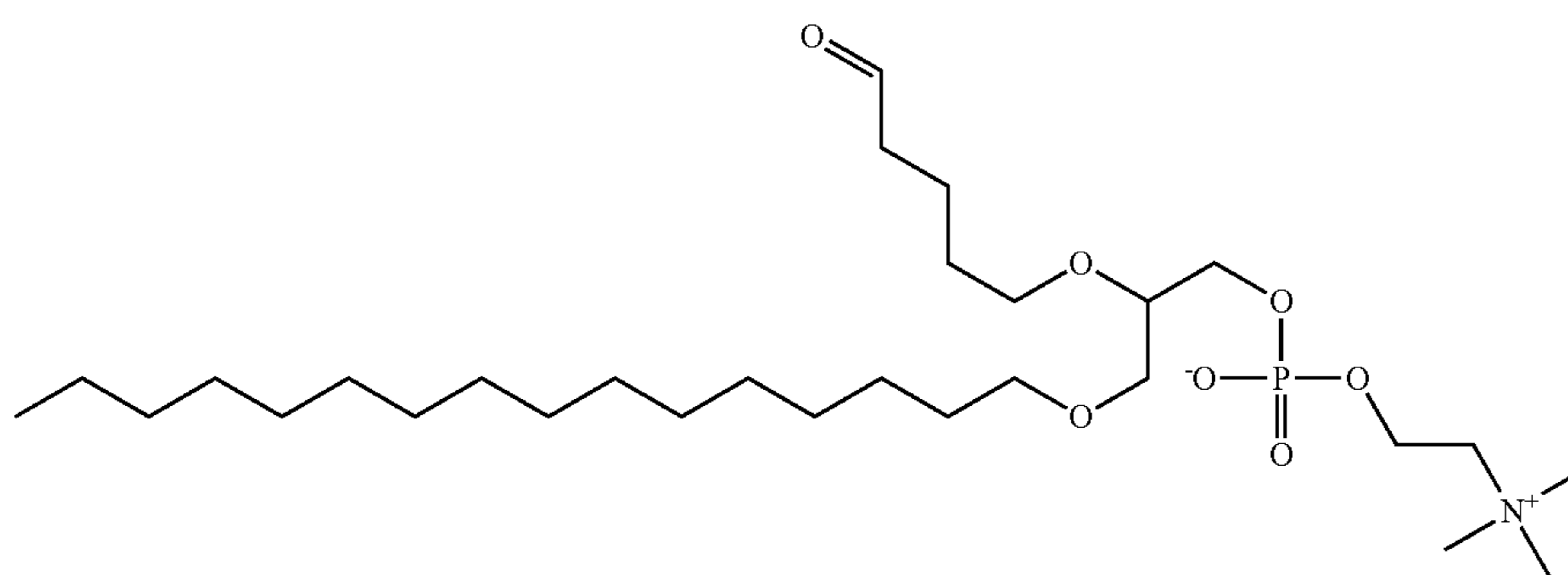
1-hexadecyl-2-(5'-oxo-pentanyl)-sn-glycero-3-phosphocholine
