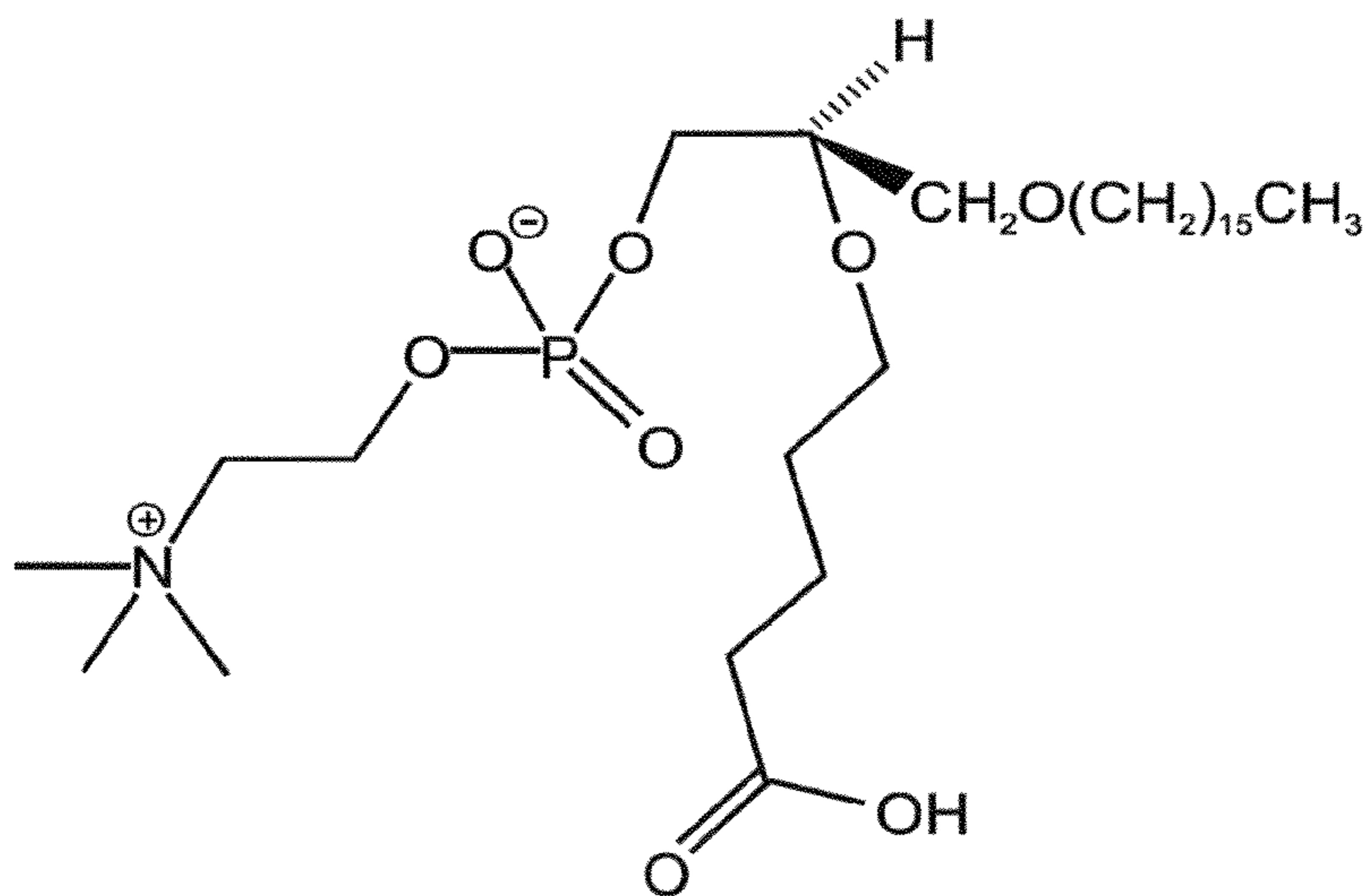
Compound VII (CI-201)
