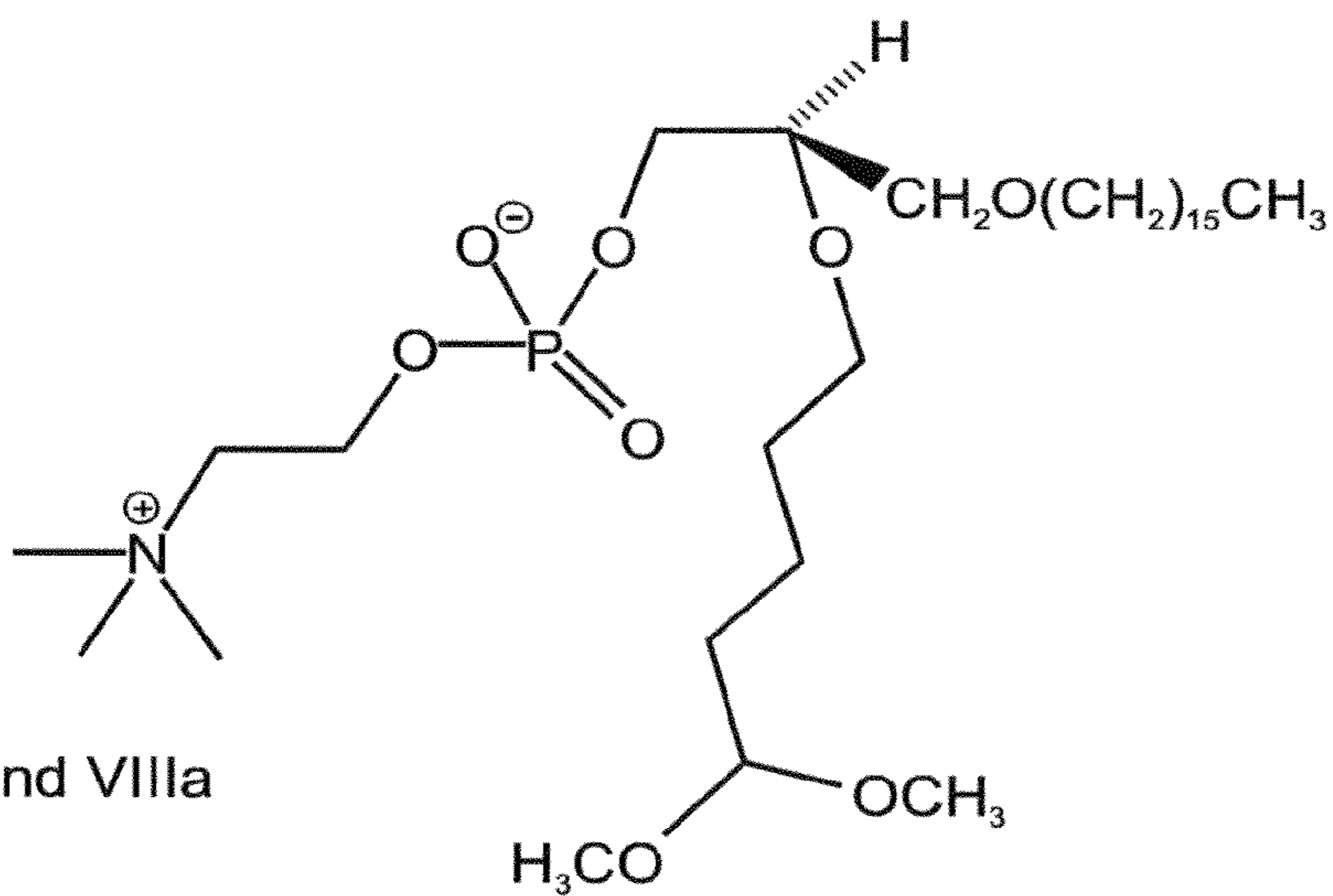
Compound VII (CI-201)
