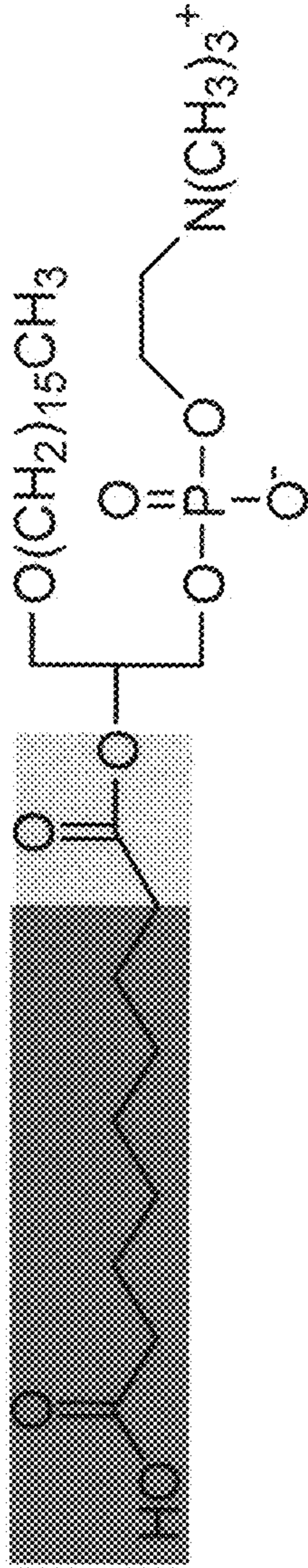
1-O-Hexadecyl-2-Azelaoyl-sn-Glycero-3-Phosphocholine (azPC)
