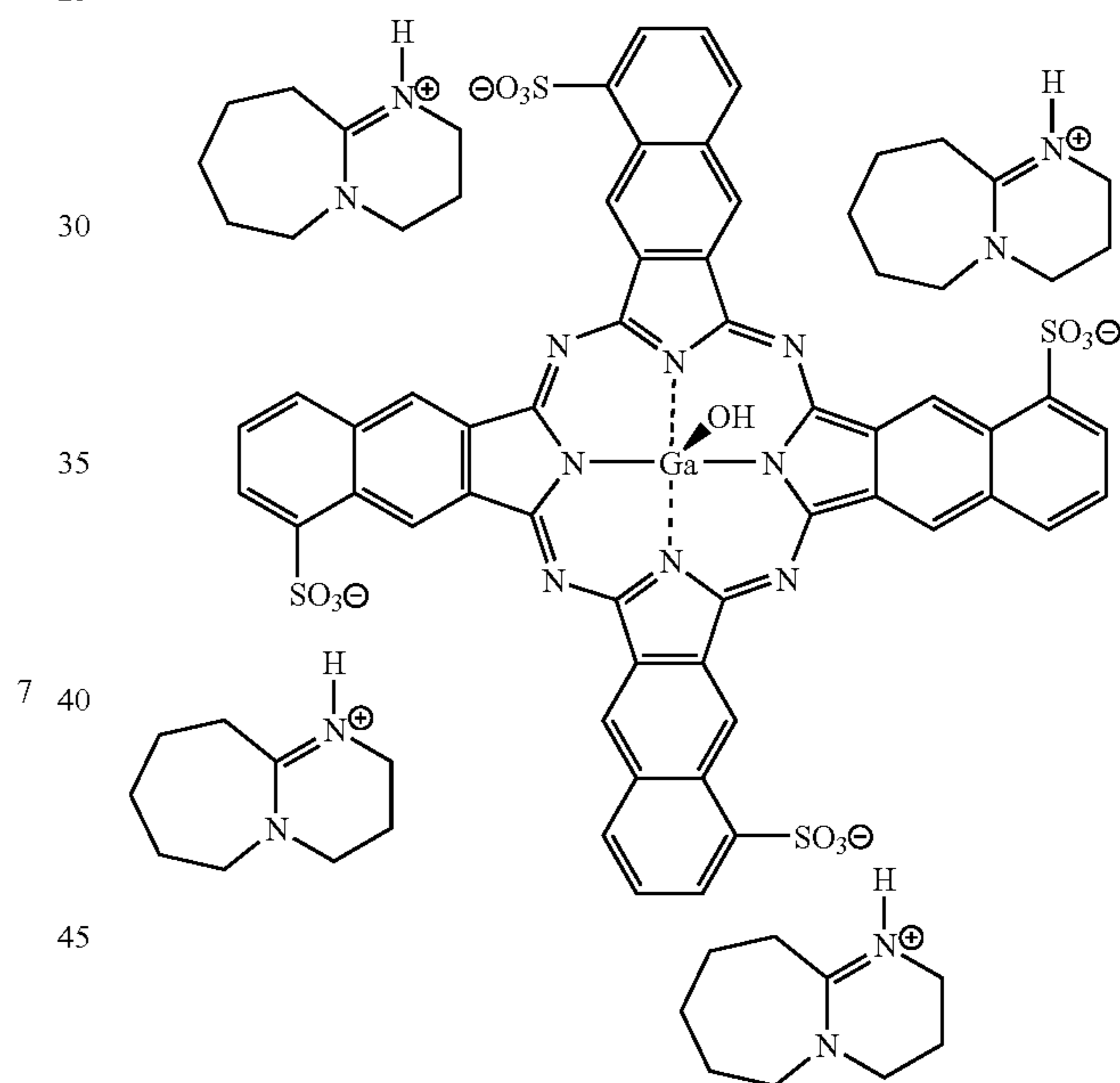
(a) Tetrapyrrolium 5
