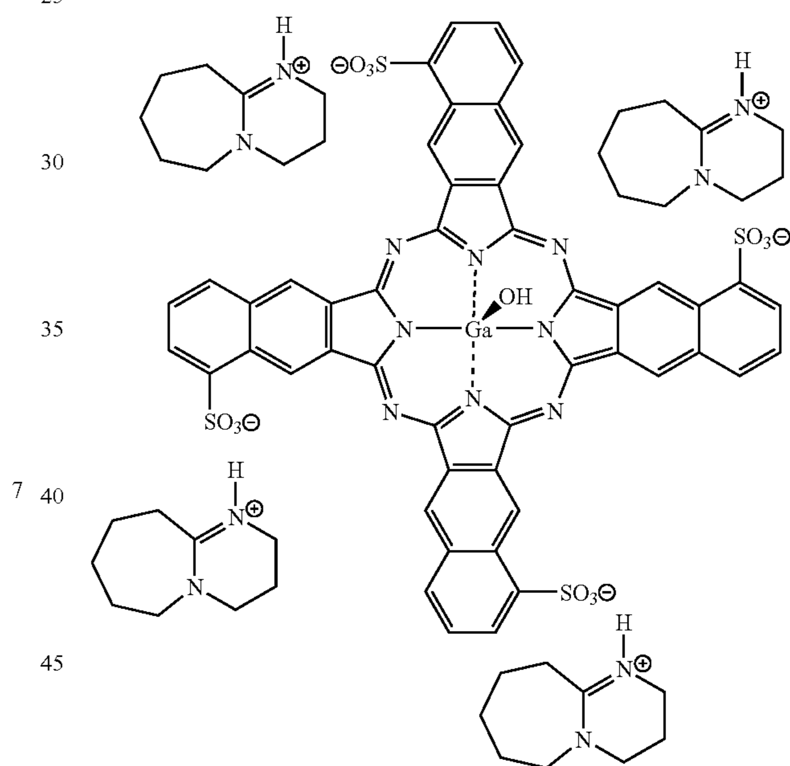
(a) Tetrapyrrolium 5
