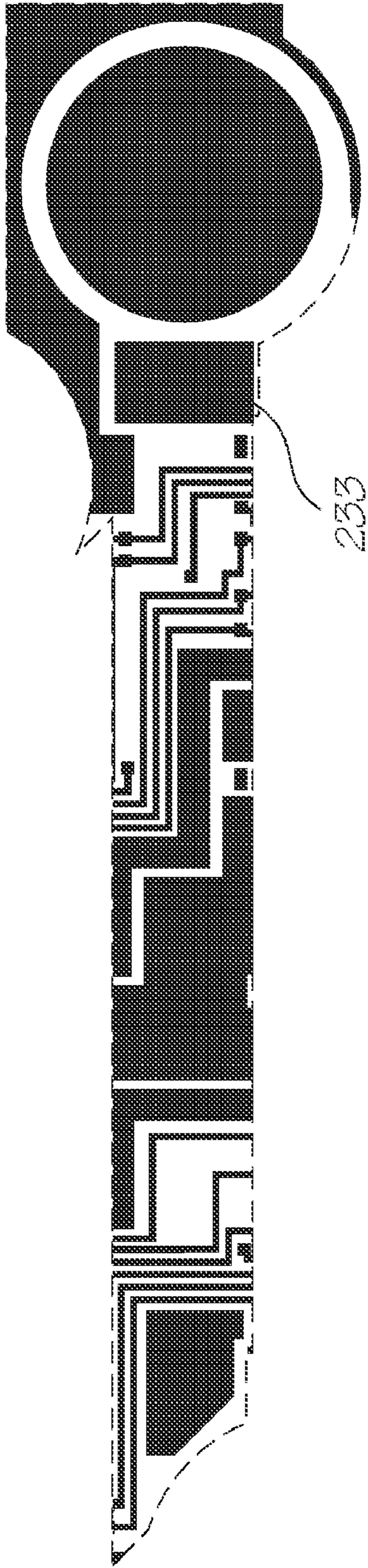
Metal 2 mask
