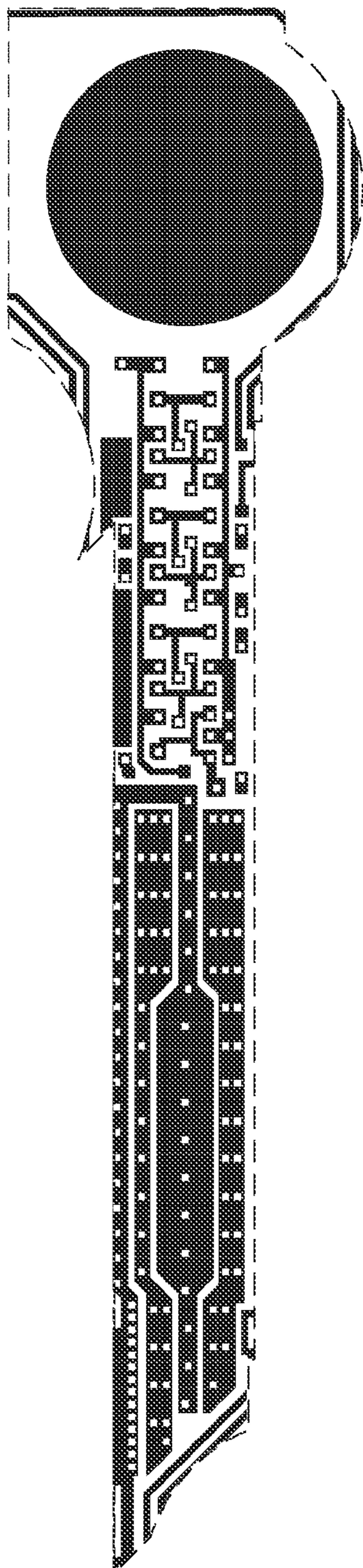
Metal 1 mask
