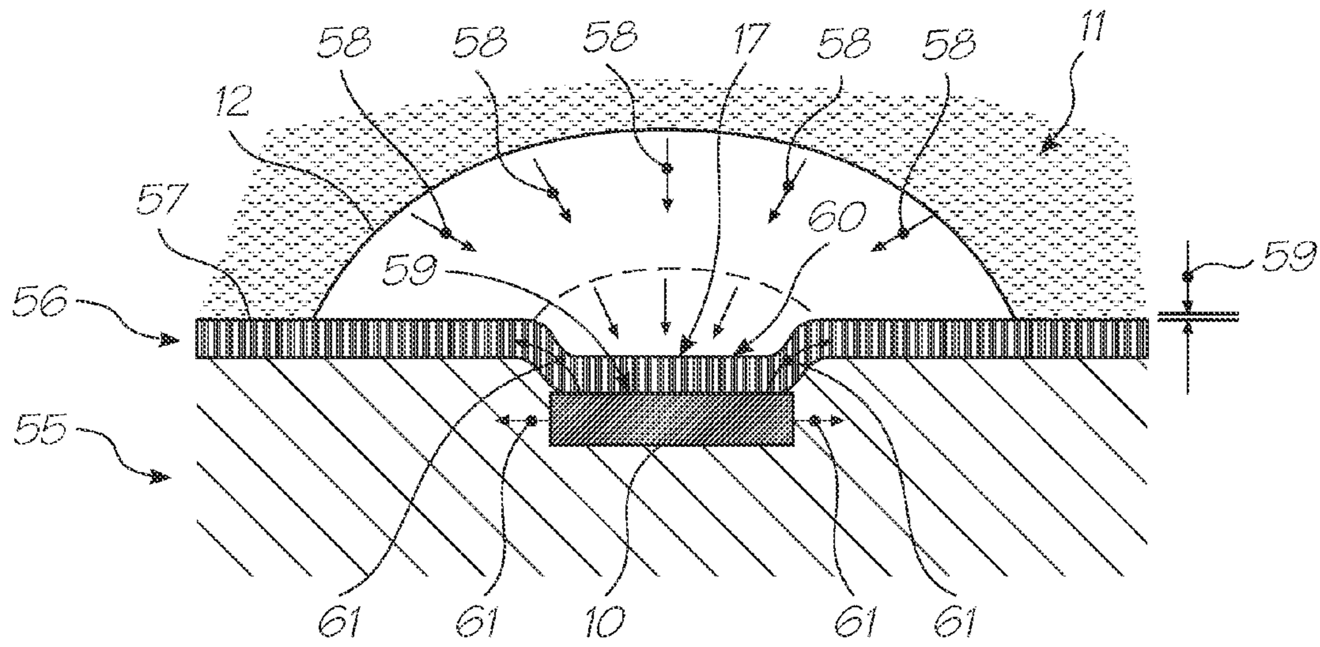
FIG. 47 (PRIOR ART)
