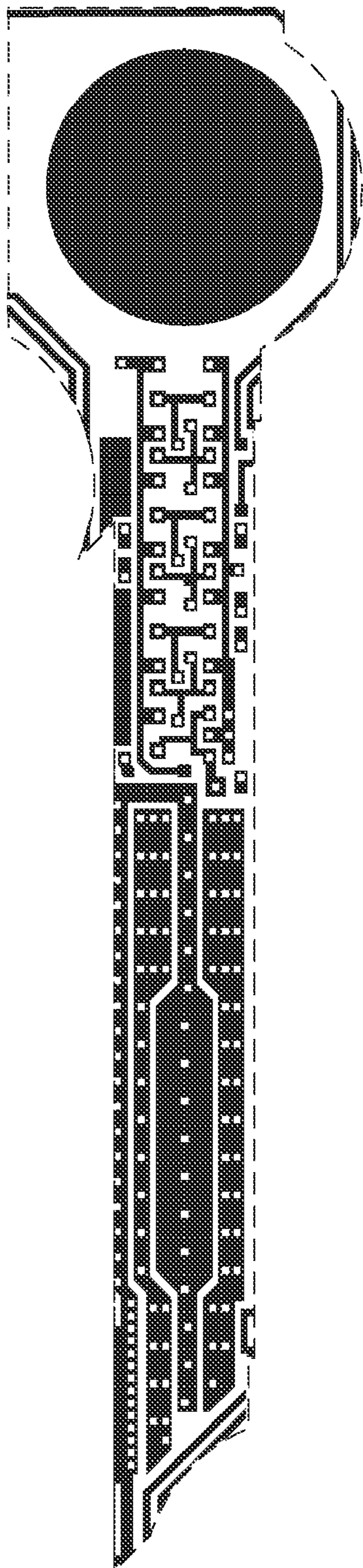
Metal 1 mask
