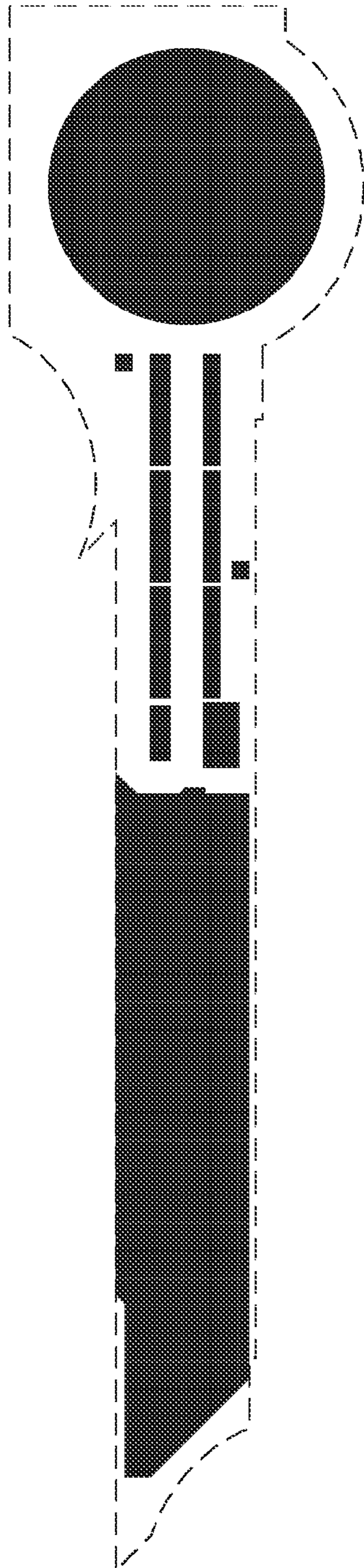
Active mask
