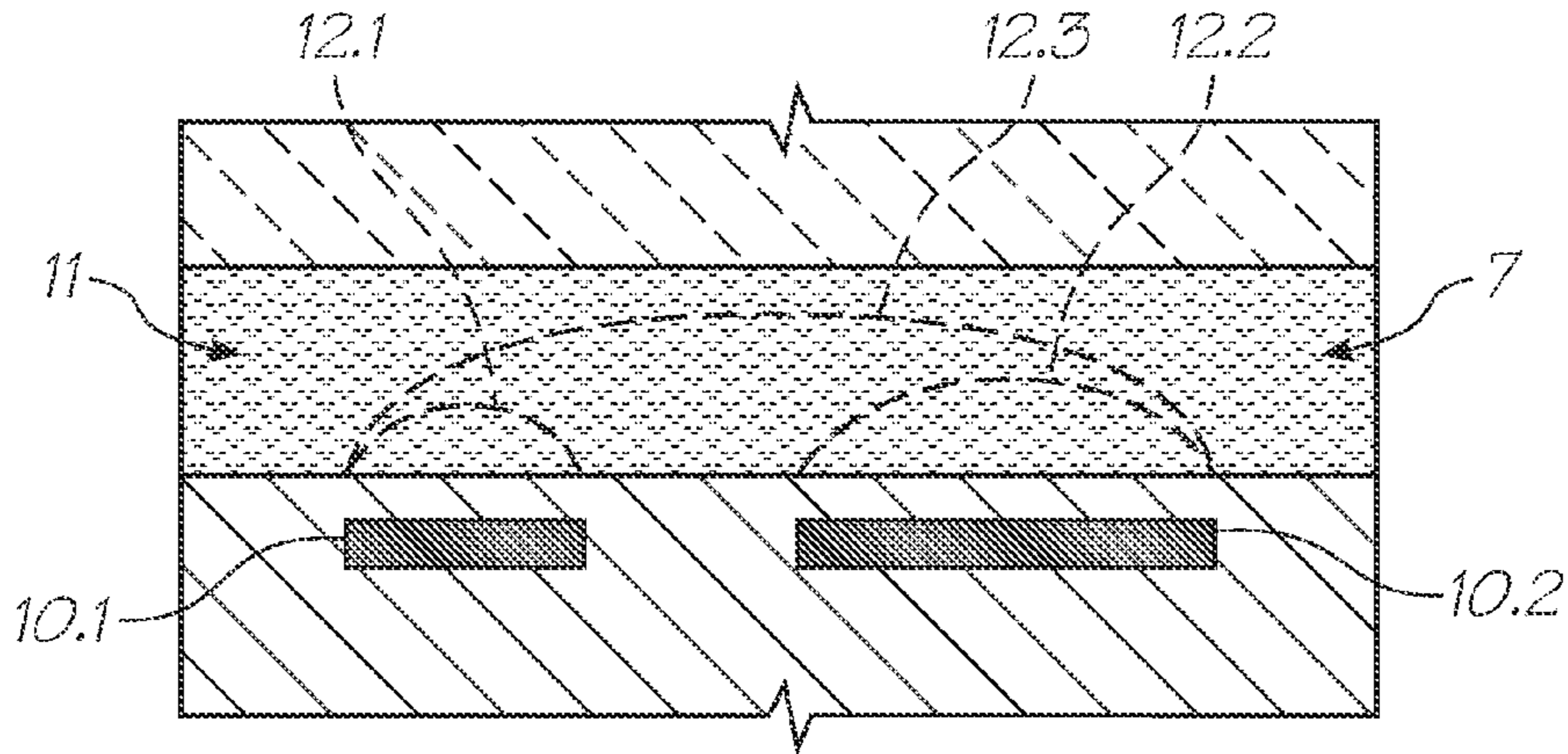
FIG. 52 (PRIOR ART)
