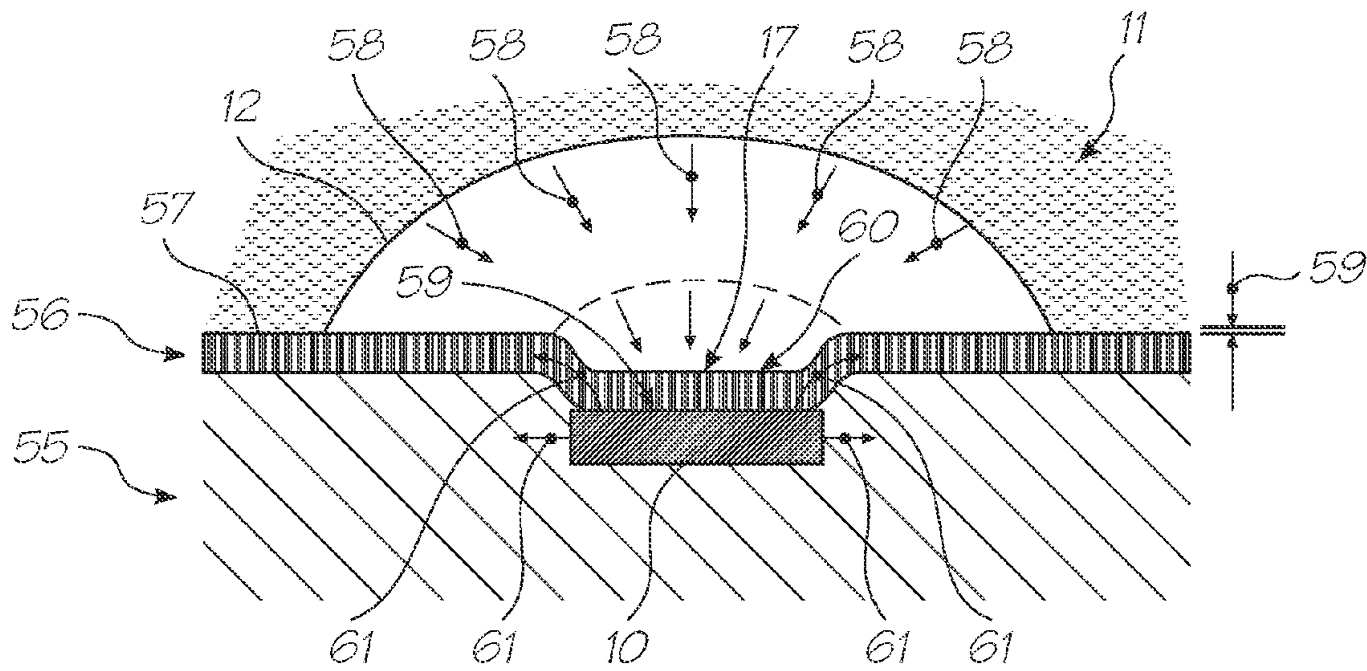
FIG. 47 (PRIOR ART)
