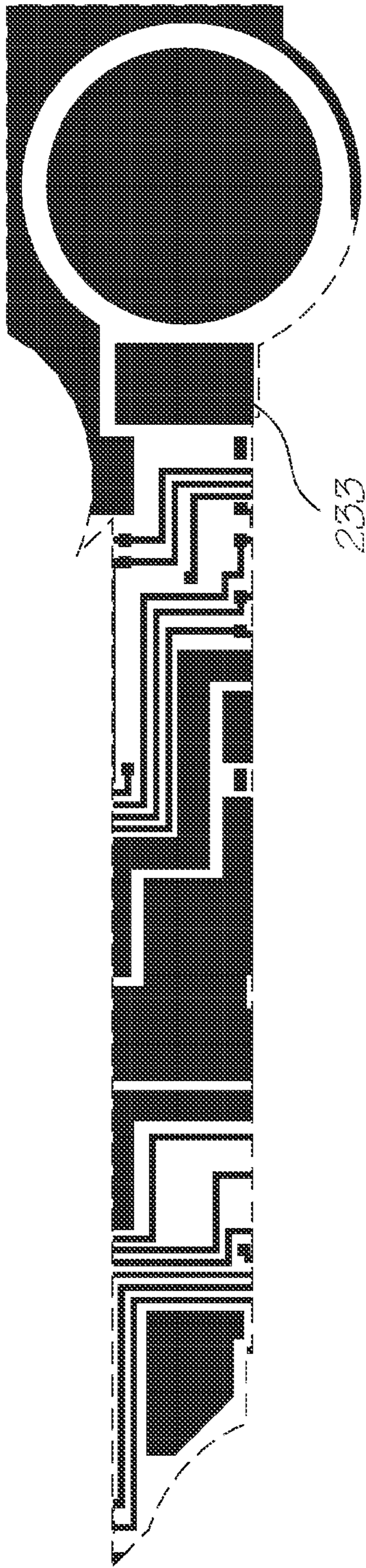
Metal 2 mask
