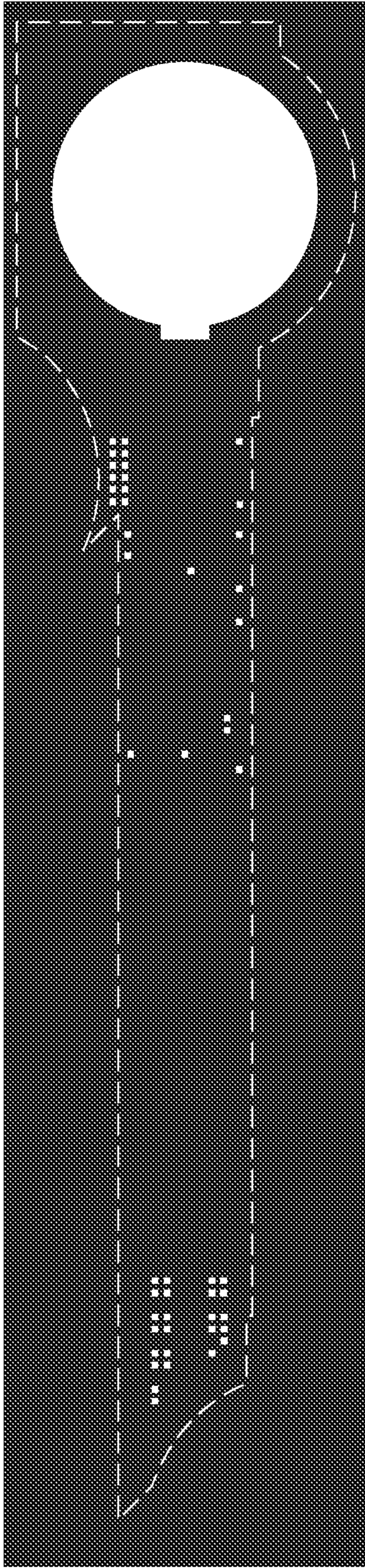
Via 1 mask
