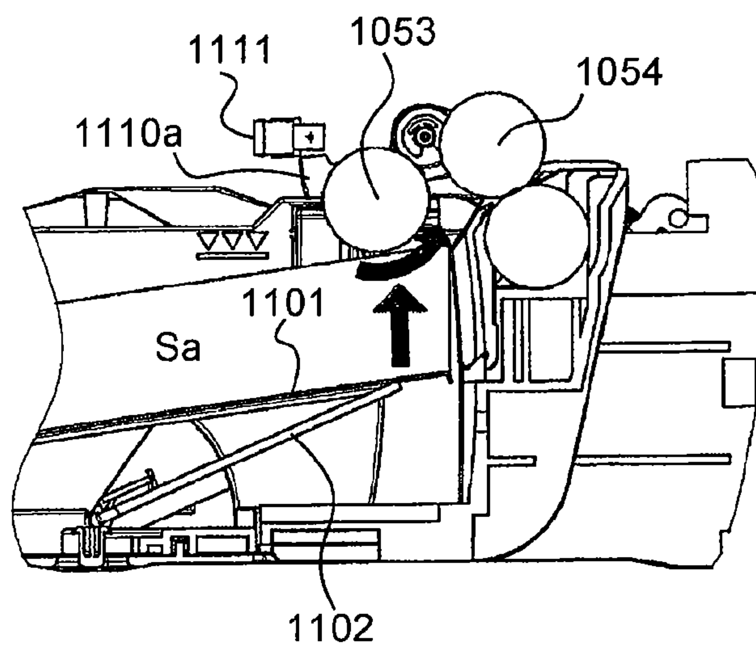
FIG. 9C PRIOR ART
