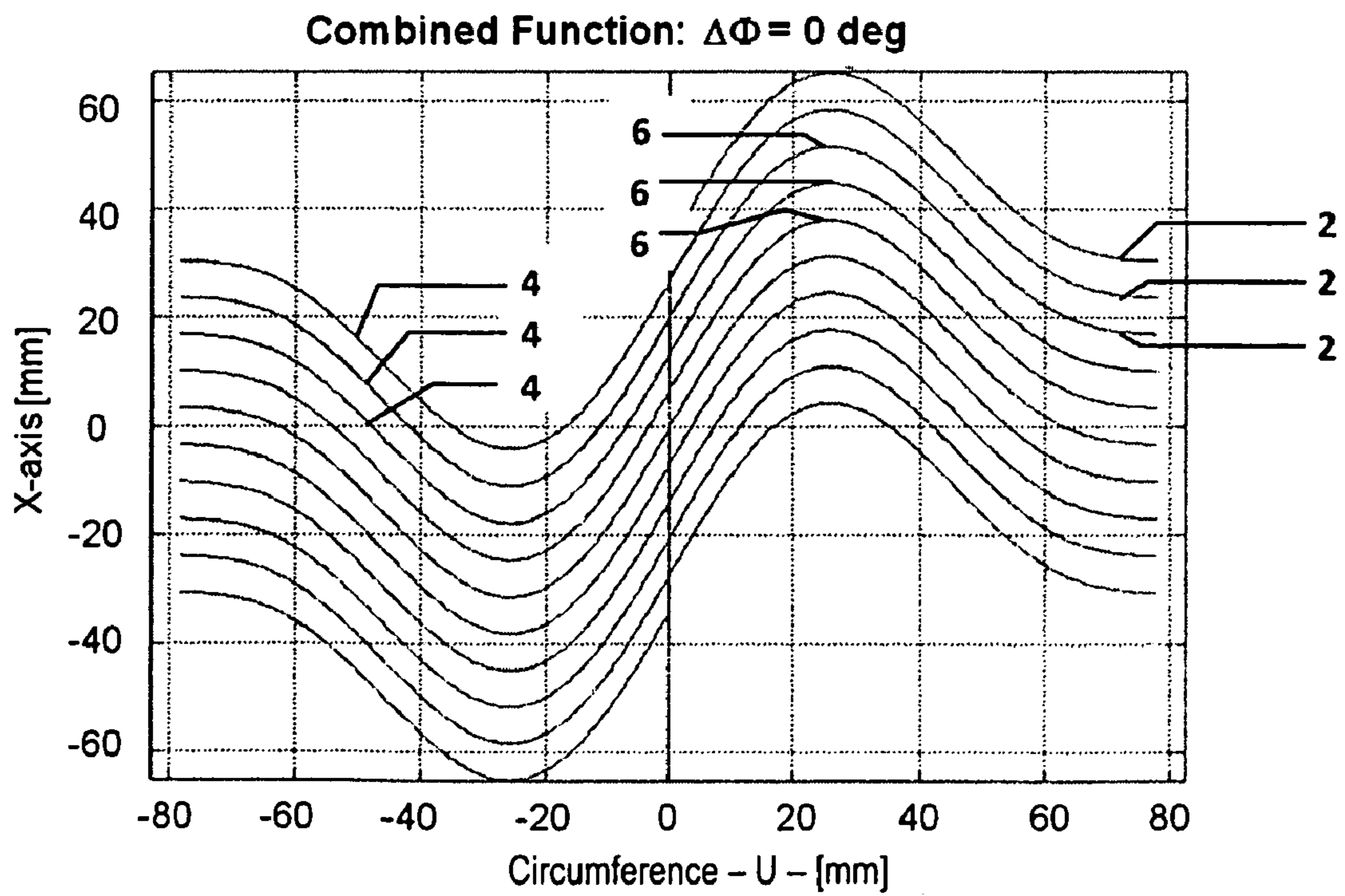
Figure 6: (Prior Art)
