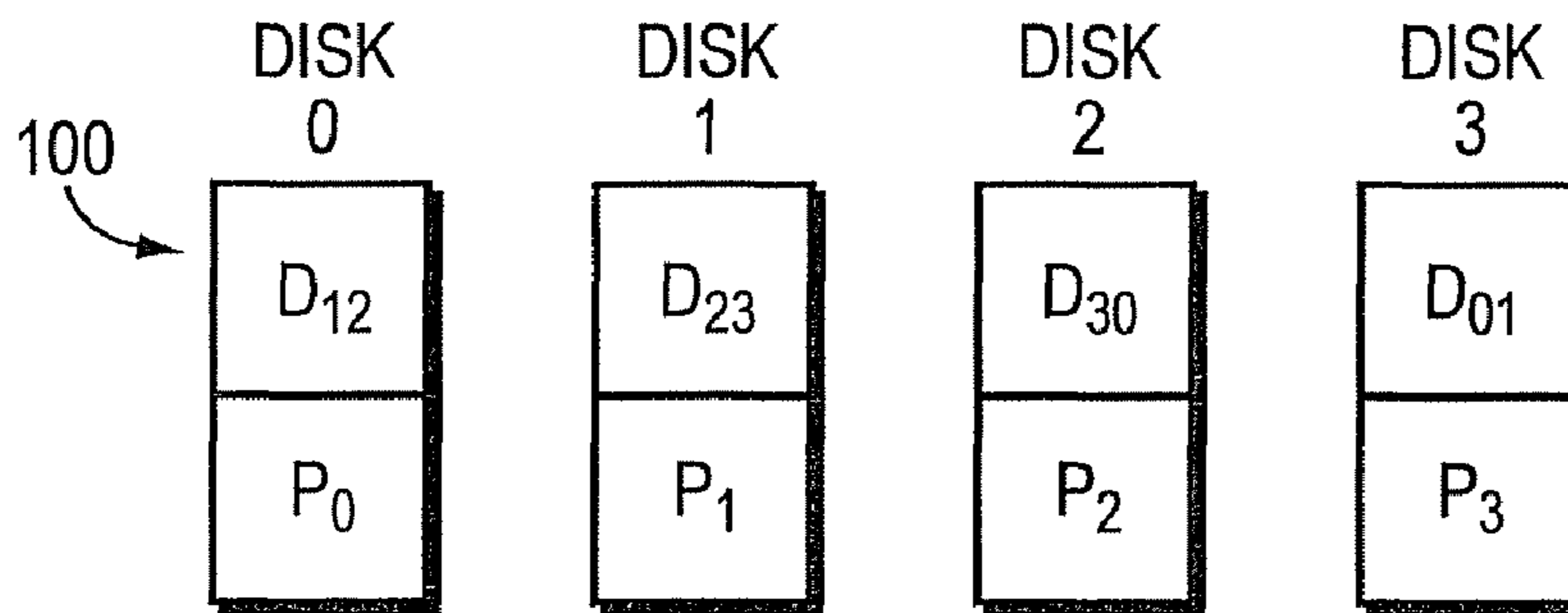
FIG. 1 (PRIOR ART)
