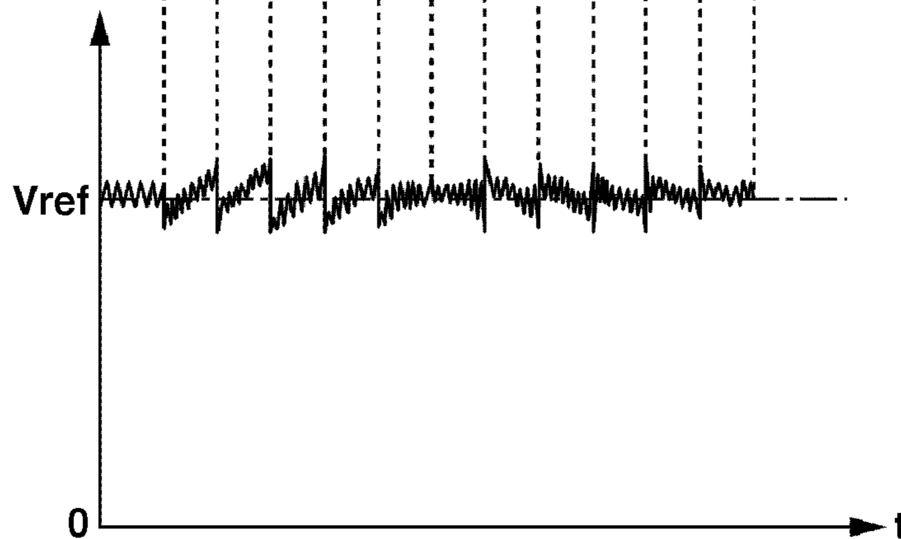
FIG.7C PRIOR ART VELOCITY DETECTION DATA AFTER CONTROL
