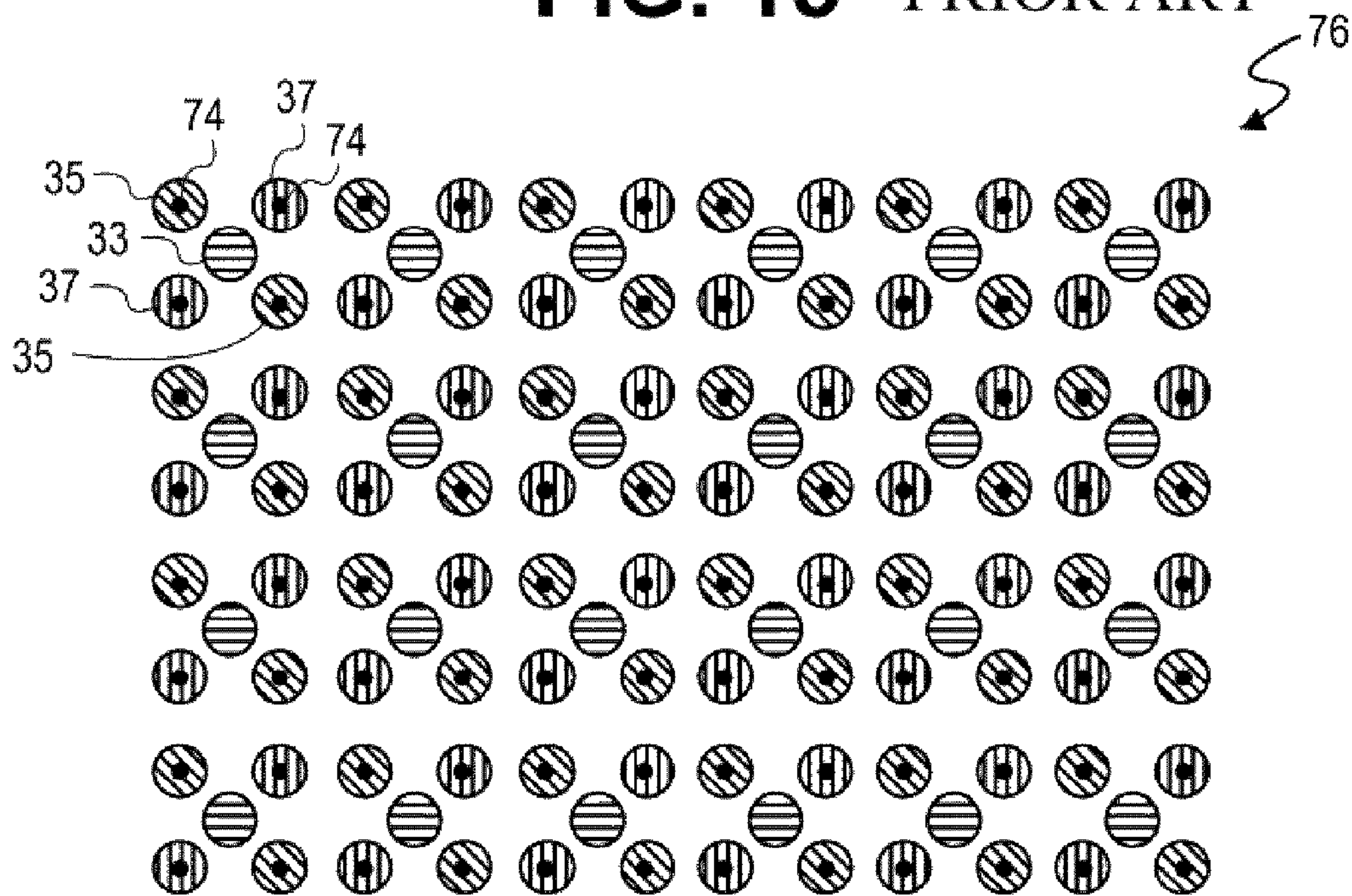
FIG. 15 PRIOR ART
