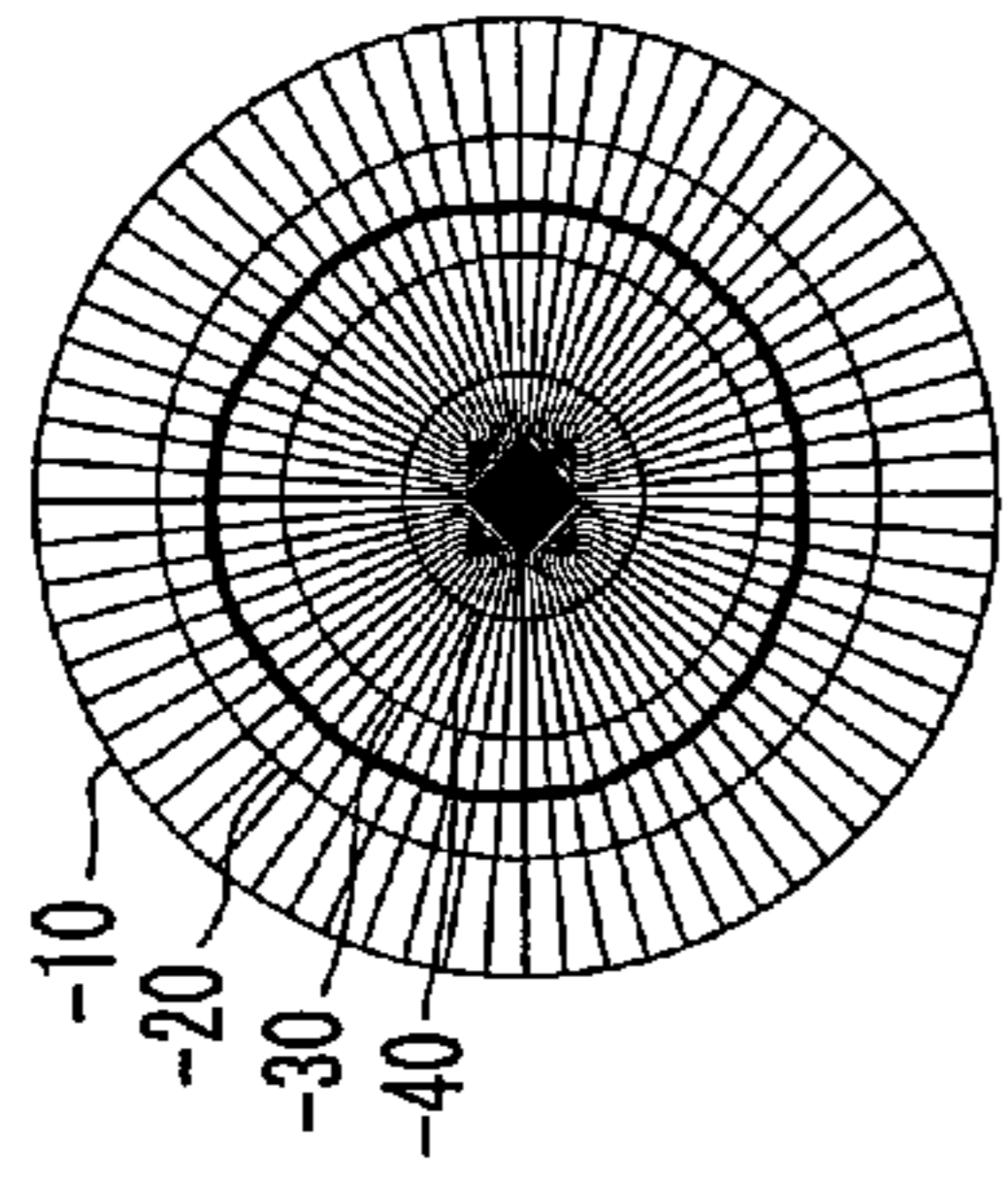
Fig. 32(b) A_d = -9\text{dB}
