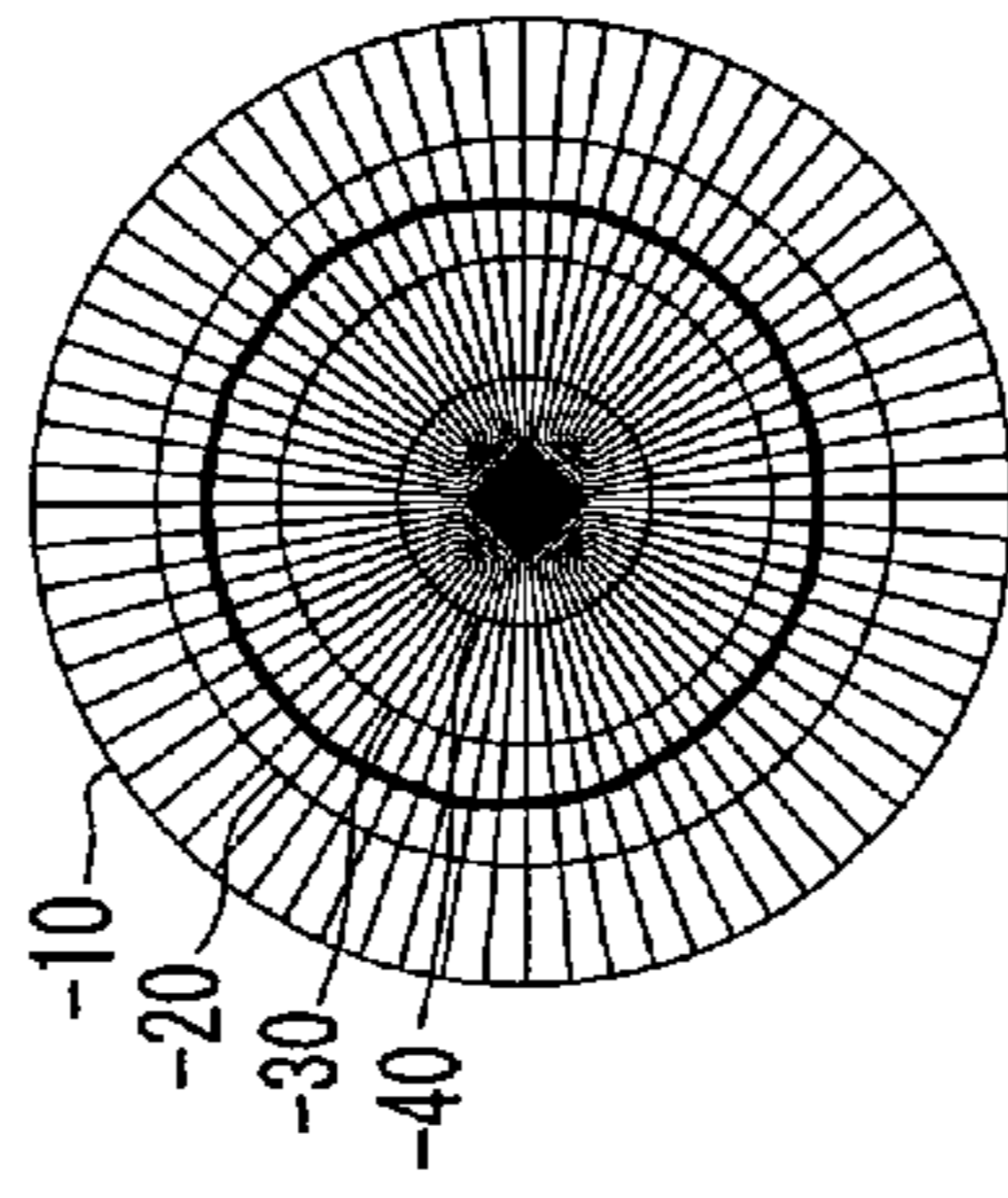
Fig. 32(e) A_d = -6\text{dB}
