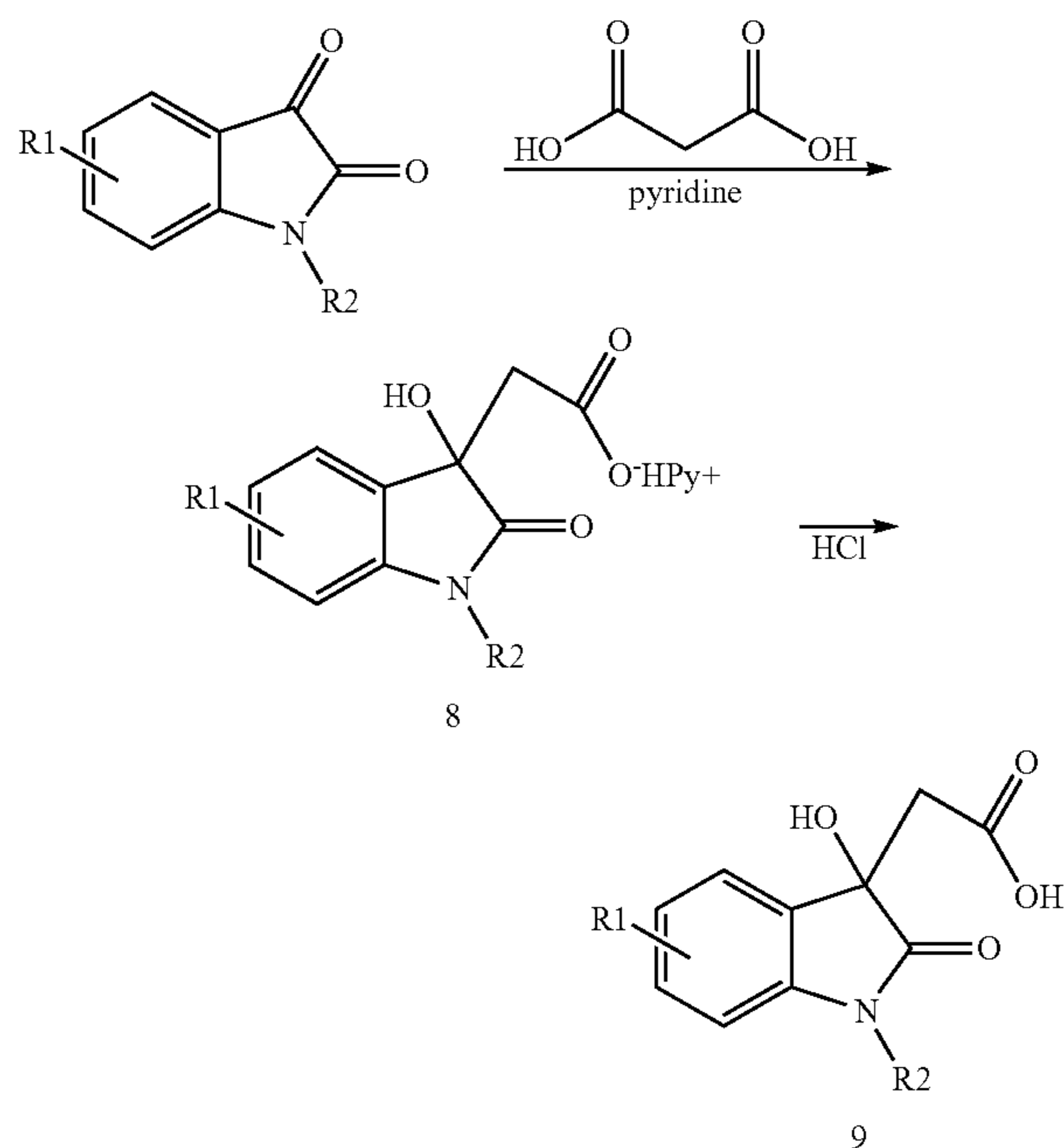
Scheme 6: Condensation of isatin with malonic acid in pyridine
