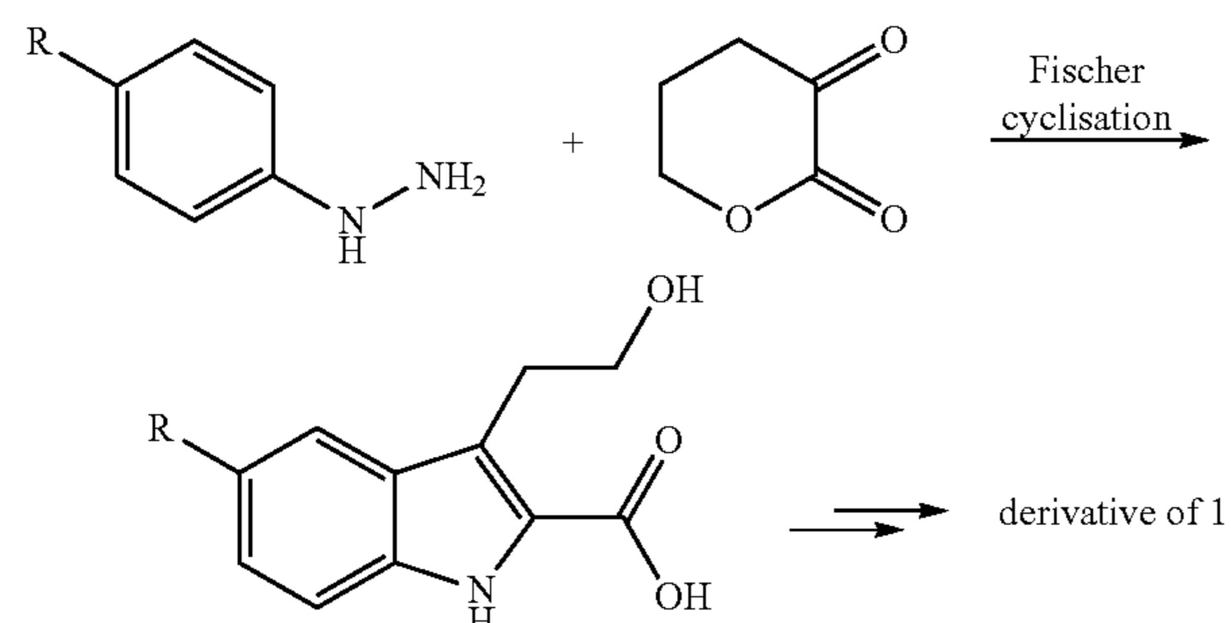
Scheme 3: Alternative Carbonyl compounds for the Fischer cyclisation
