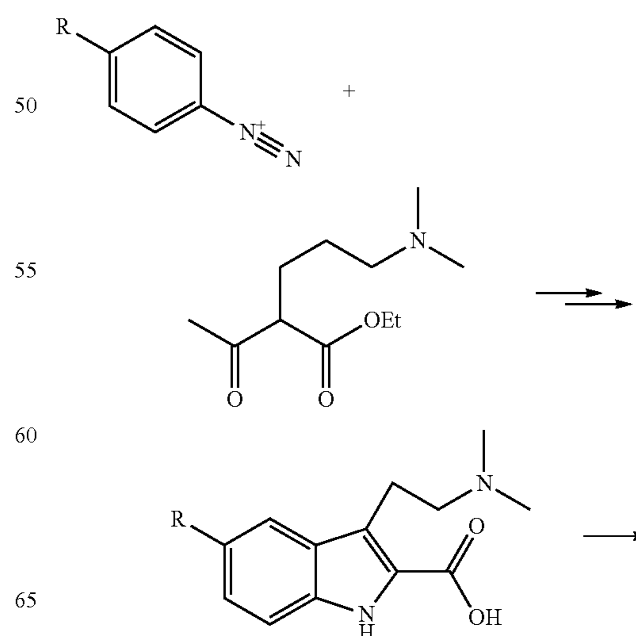
Scheme 3: Alternative Carbonyl compounds for the Fischer cyclisation
