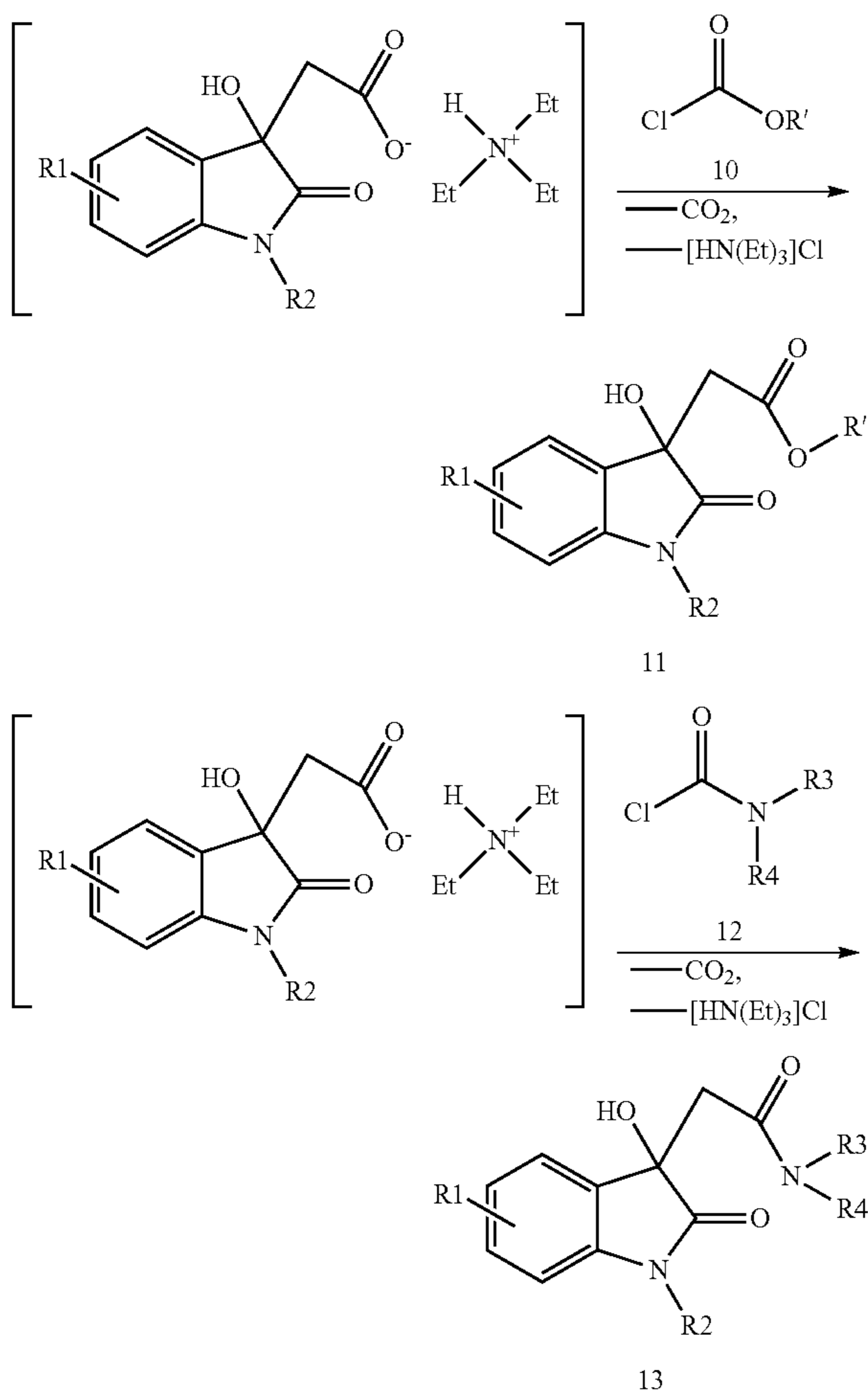
Scheme 7: Synthesis of esters 11 and amides 13 of 9
