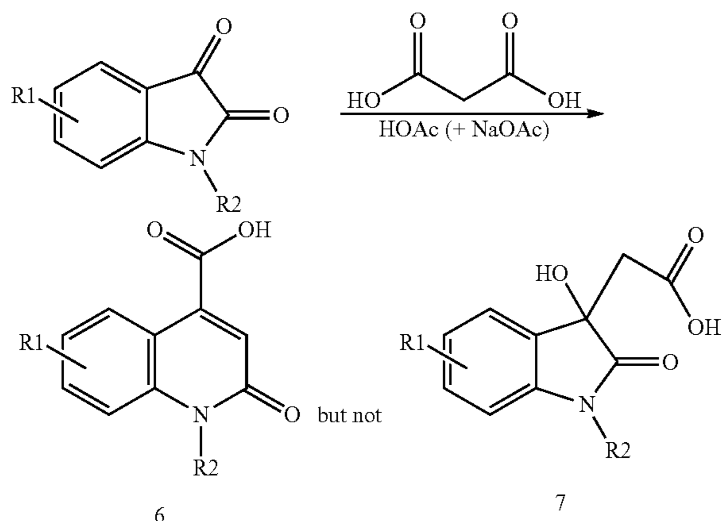
Scheme 5: Condensation of isatin with malonic acid in acetic acid
