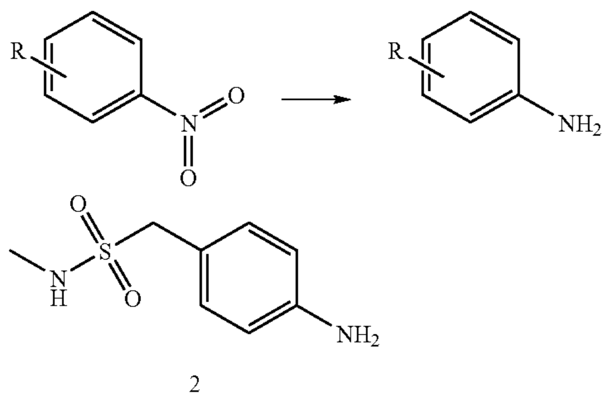
Scheme 1 Synthesis of aniline precursors for tryptamine derivatives
