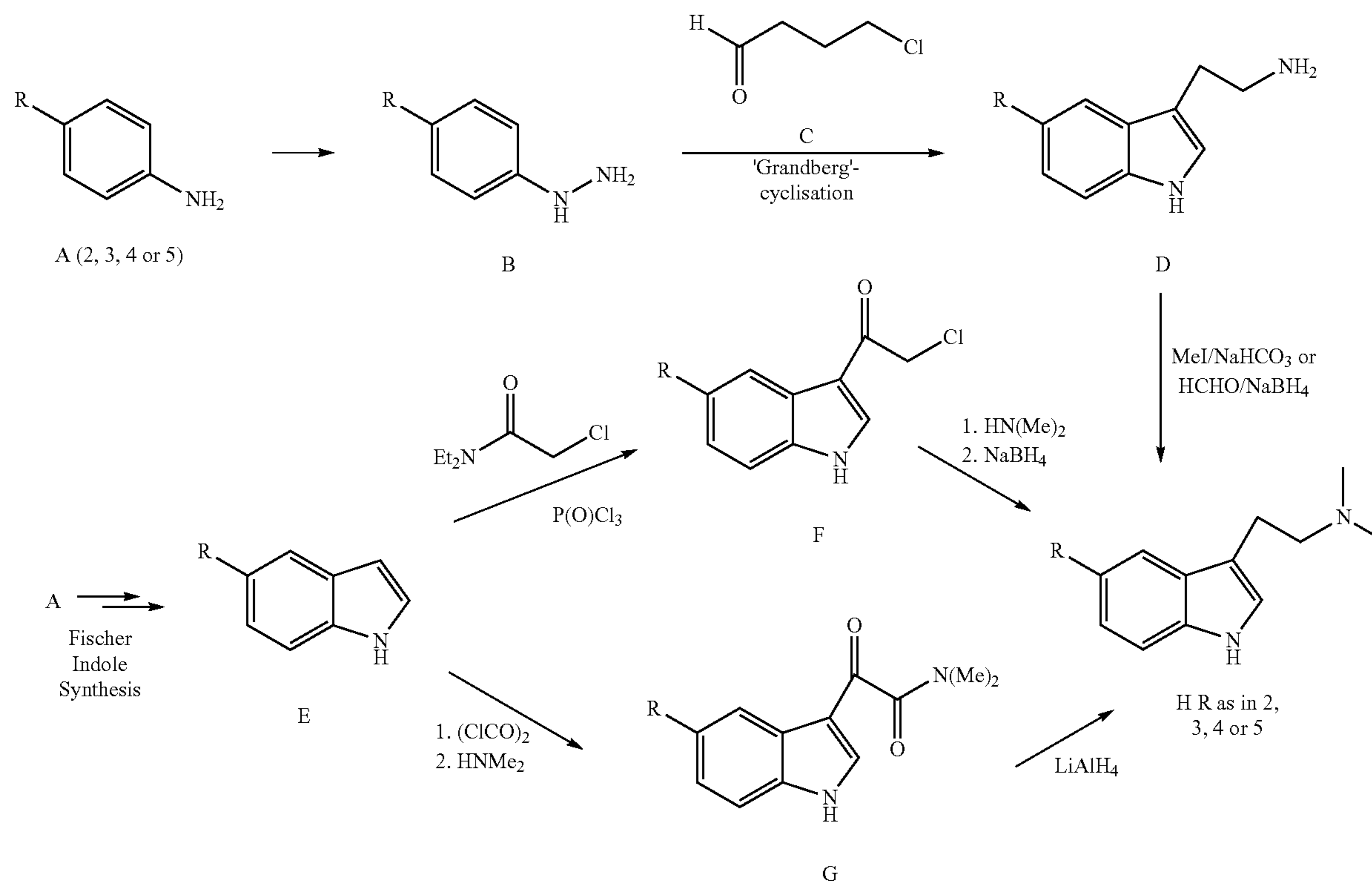
Scheme 2. Synthesis of tryptanes from their aniline precursors
