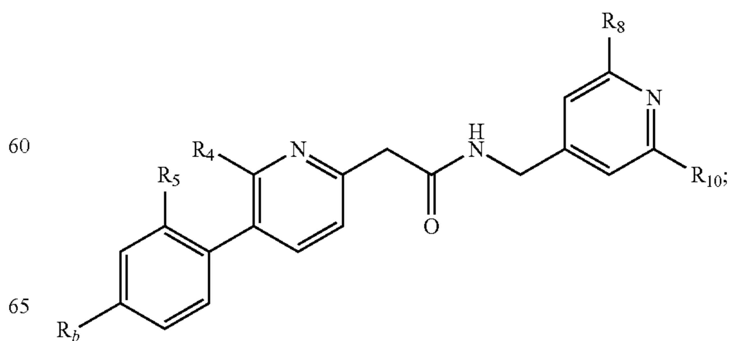
Formula XI:
