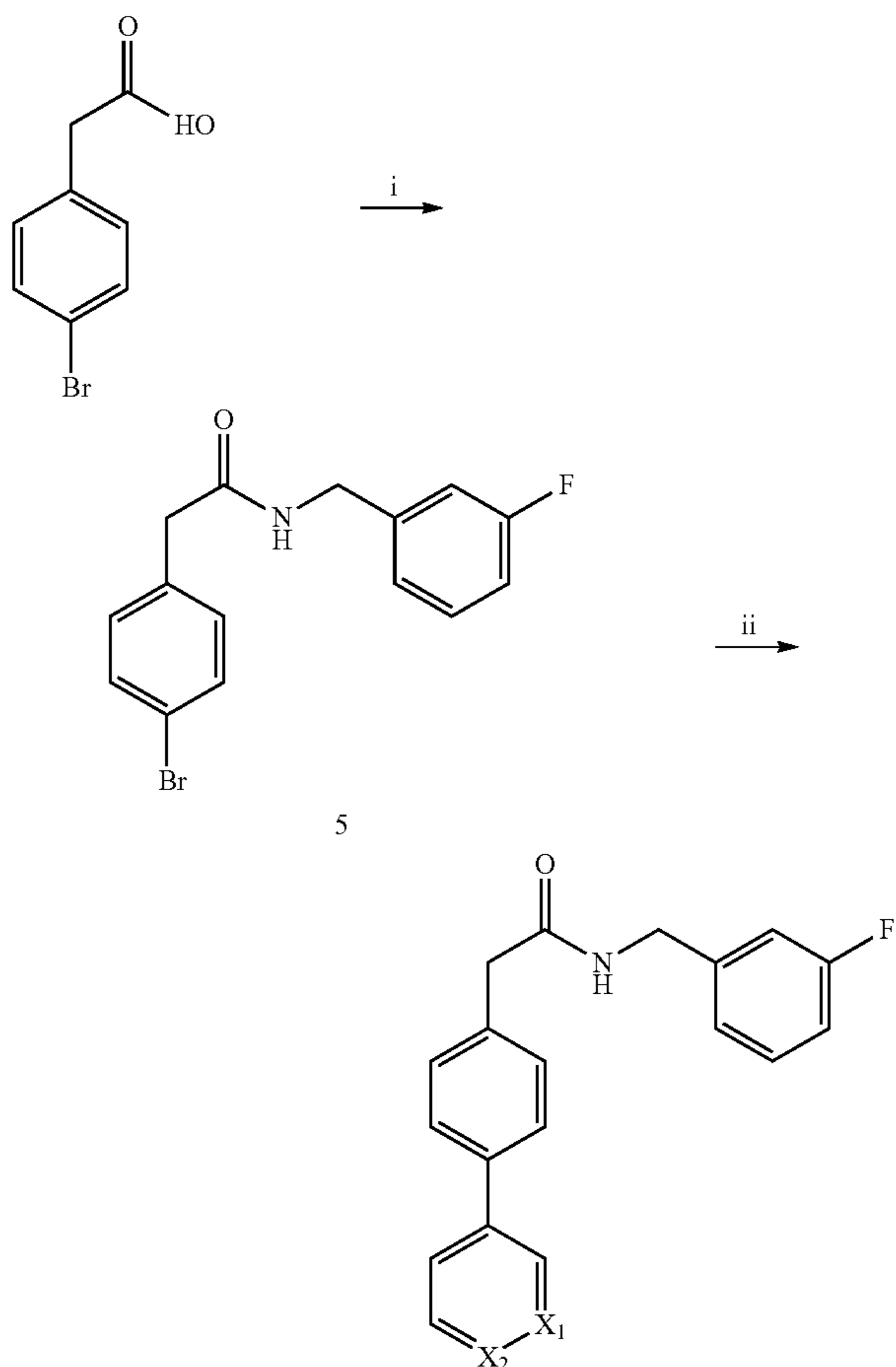
Scheme 4
