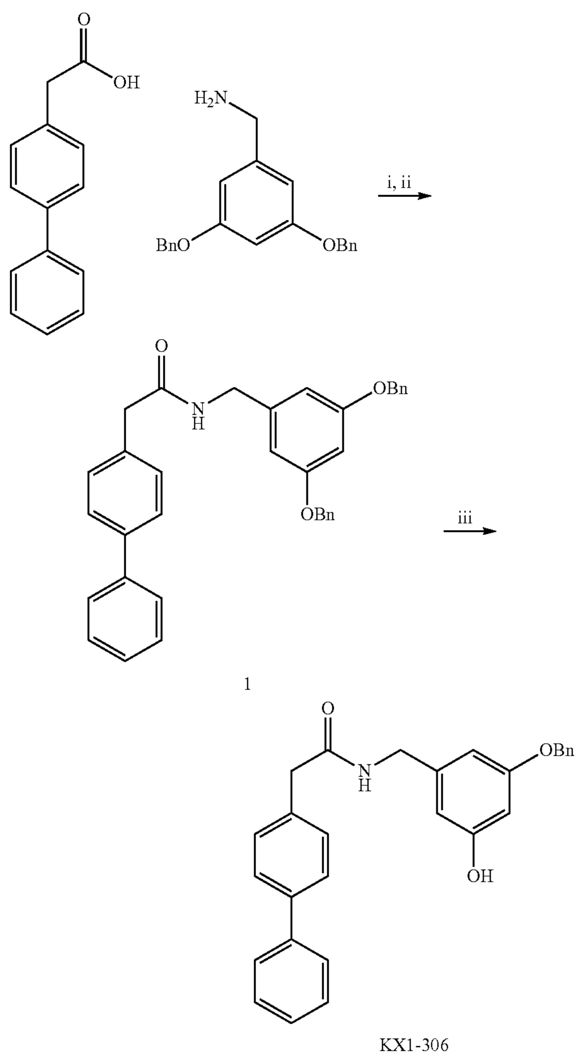
Scheme 1
