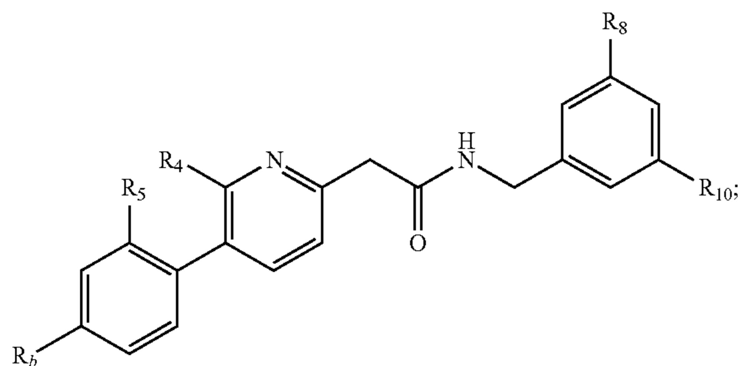
Formula III:
