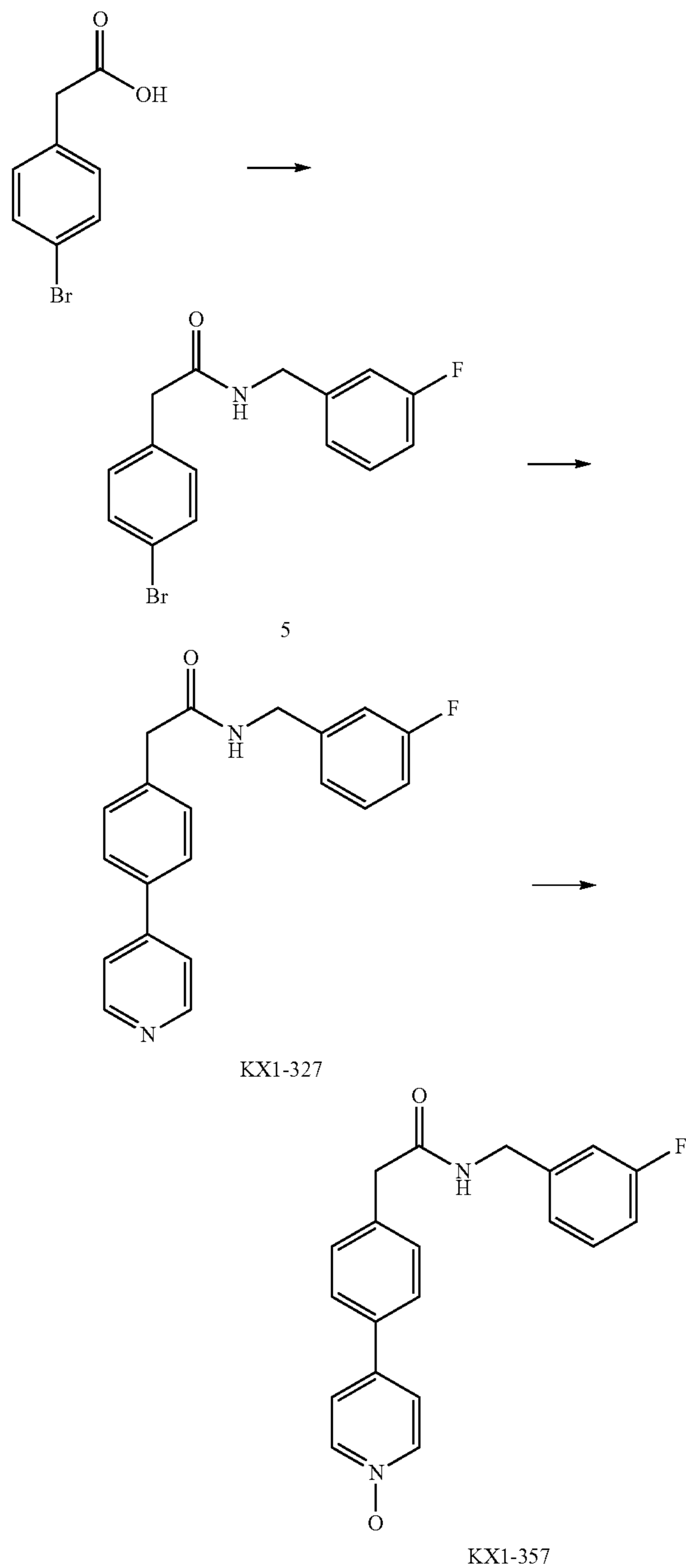
Scheme 5
