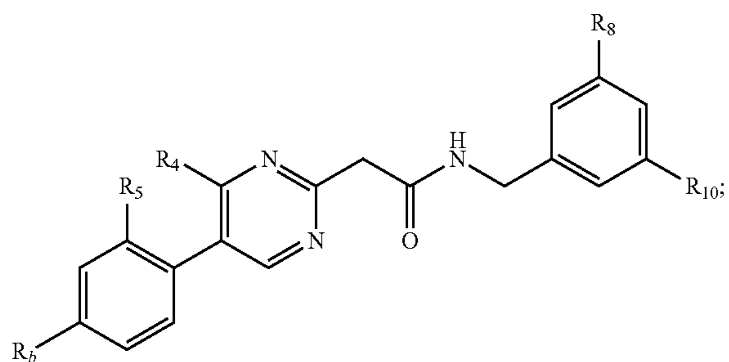
Formula III:
