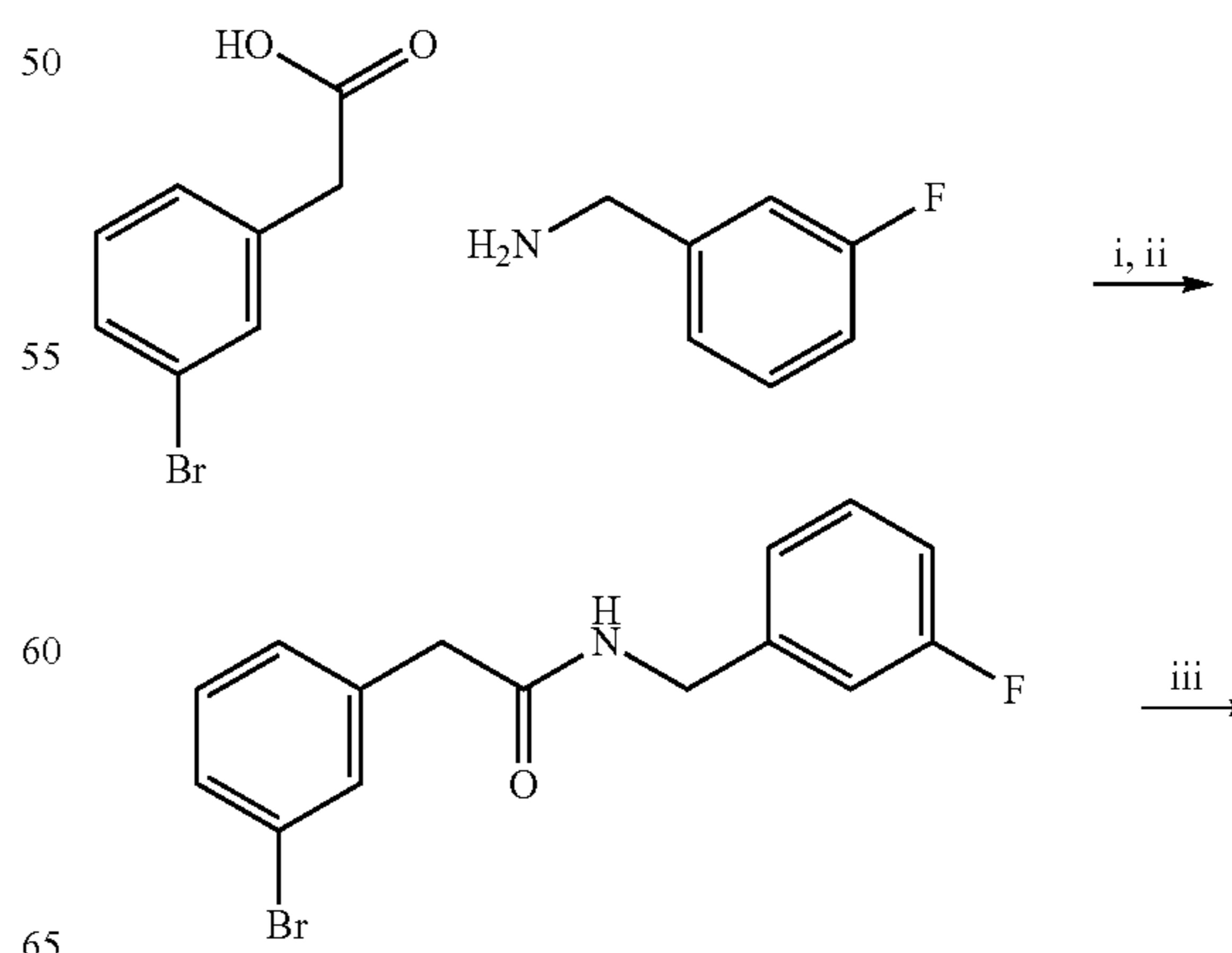
Scheme 2
