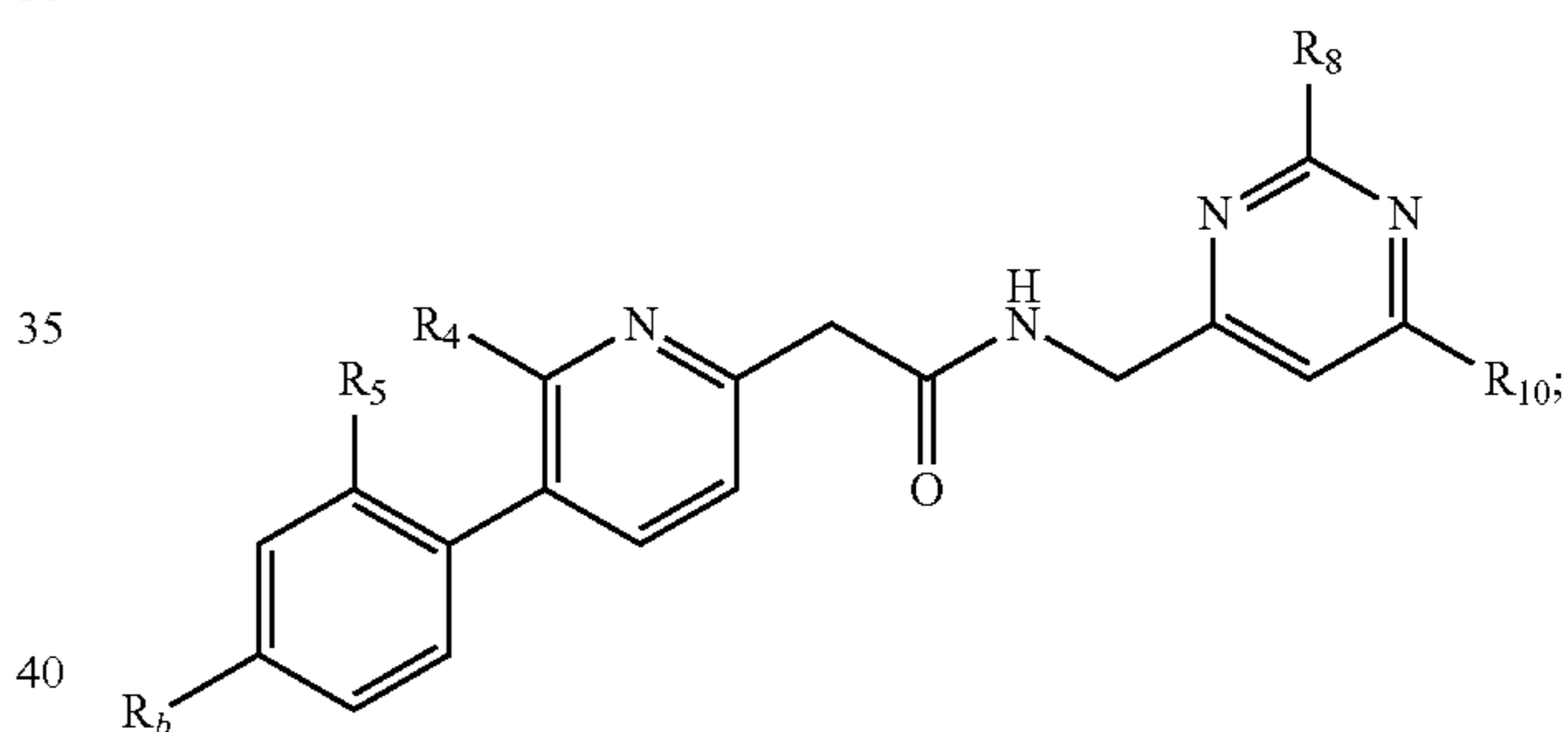
Formula X:
