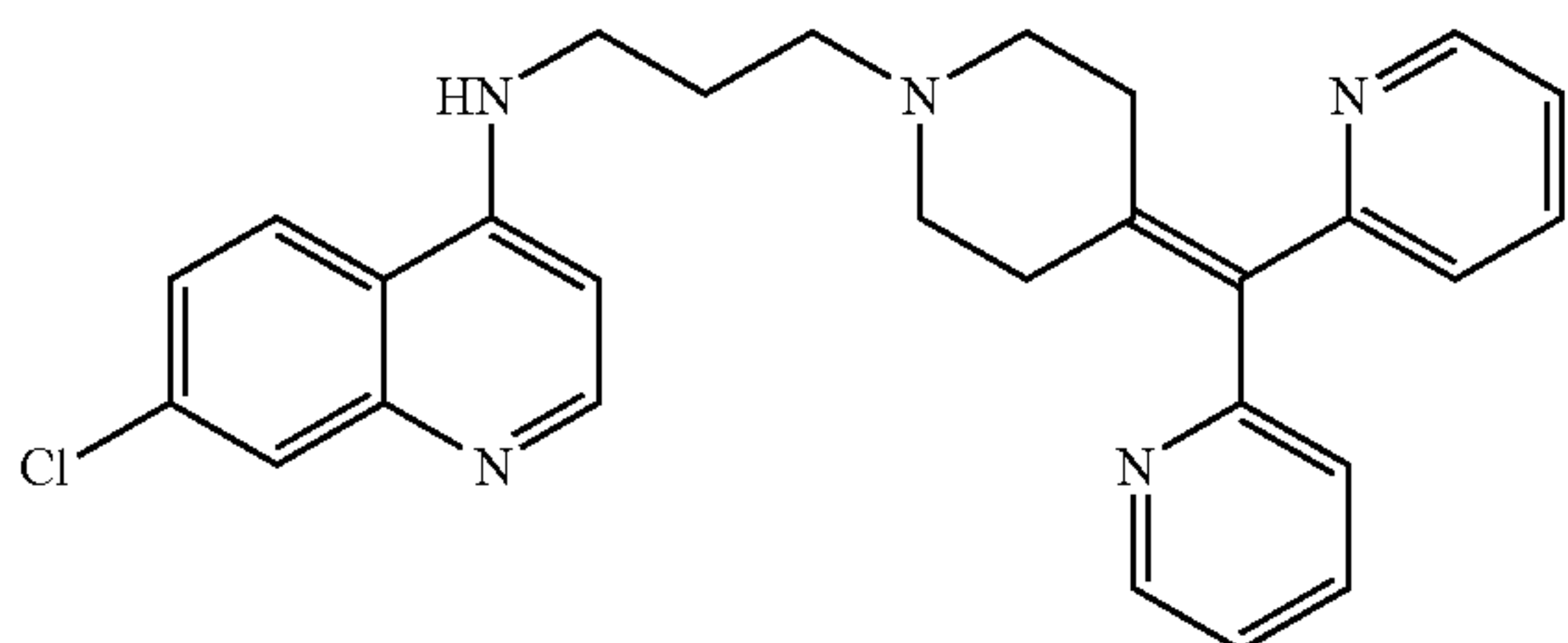
RCQ_117 Dipyrindin-2-yl-methylene derivative
