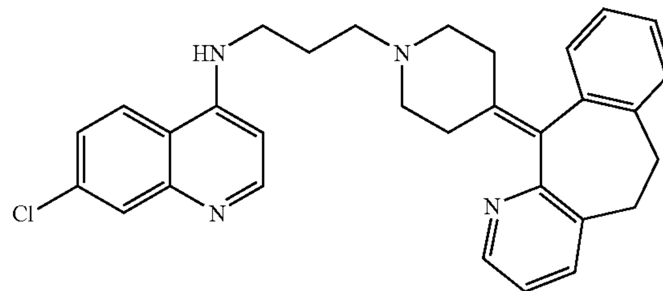
RCQ_112 (an azatadine derivative)
