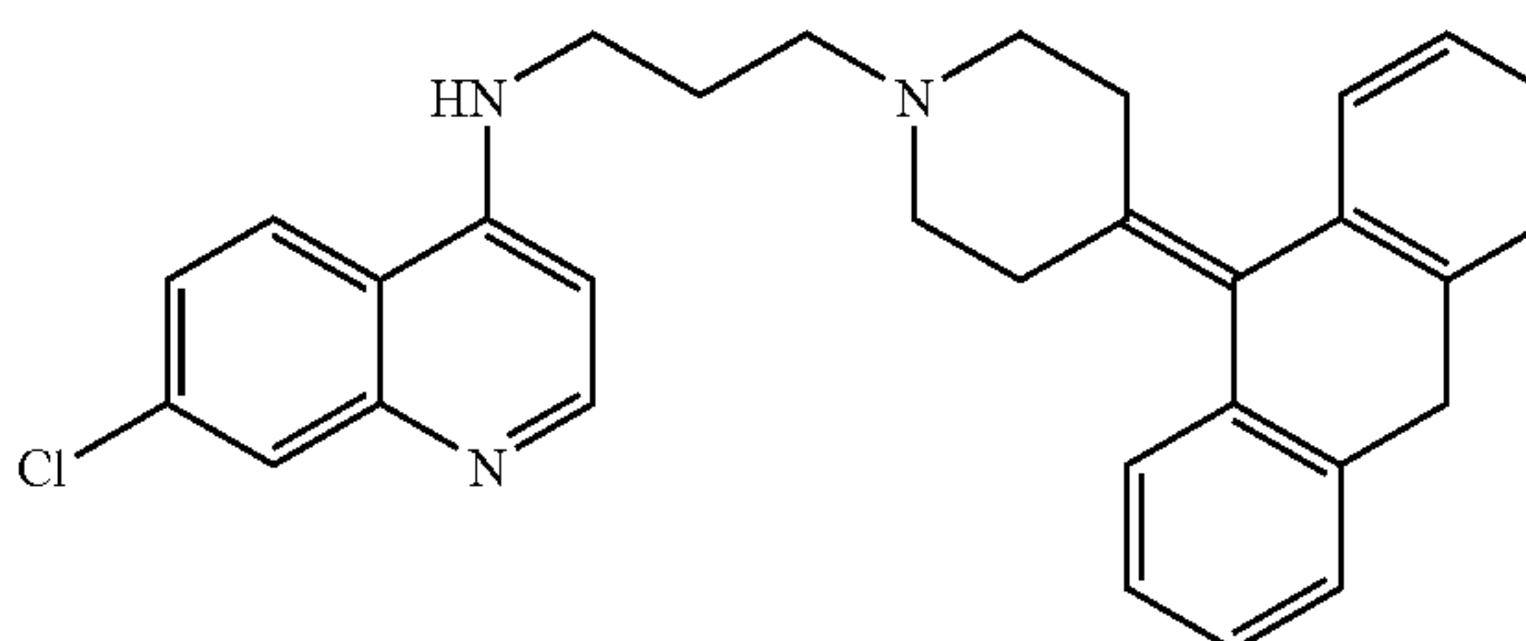
RCQ_114 10H-Anthracen-9-ylidene derivative
