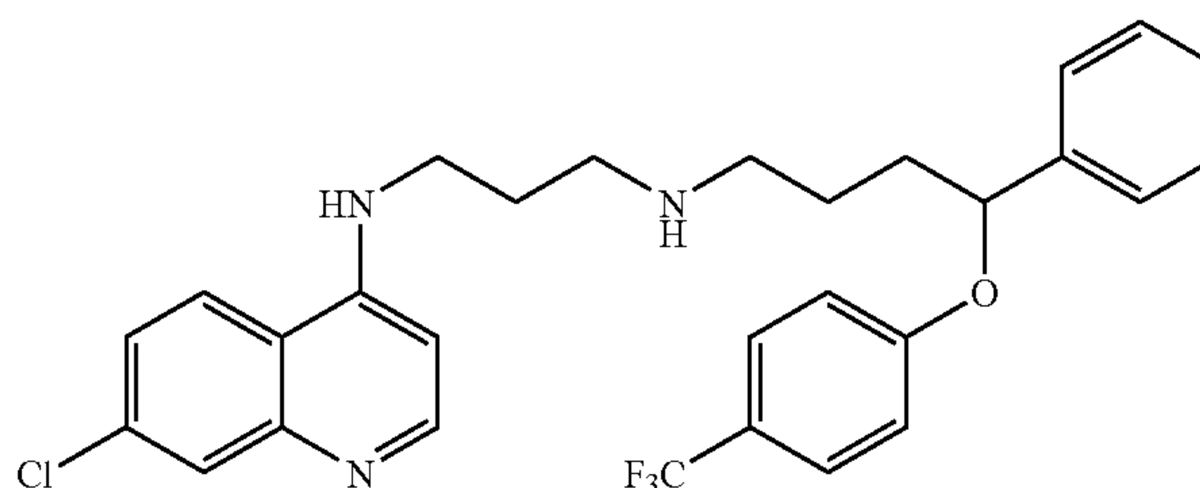
RCQ_103 (a fluoxetine derivative)
