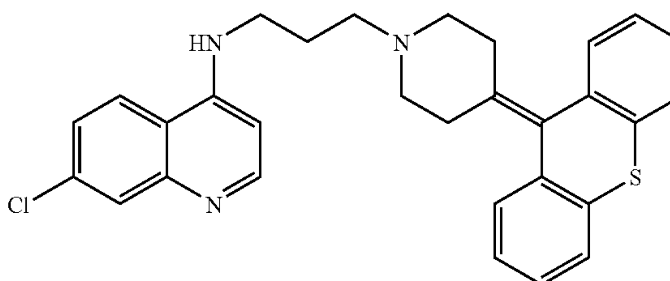
RCQ_115 4-thioxanthen-9-ylidene-piperidin-1-yl derivative
