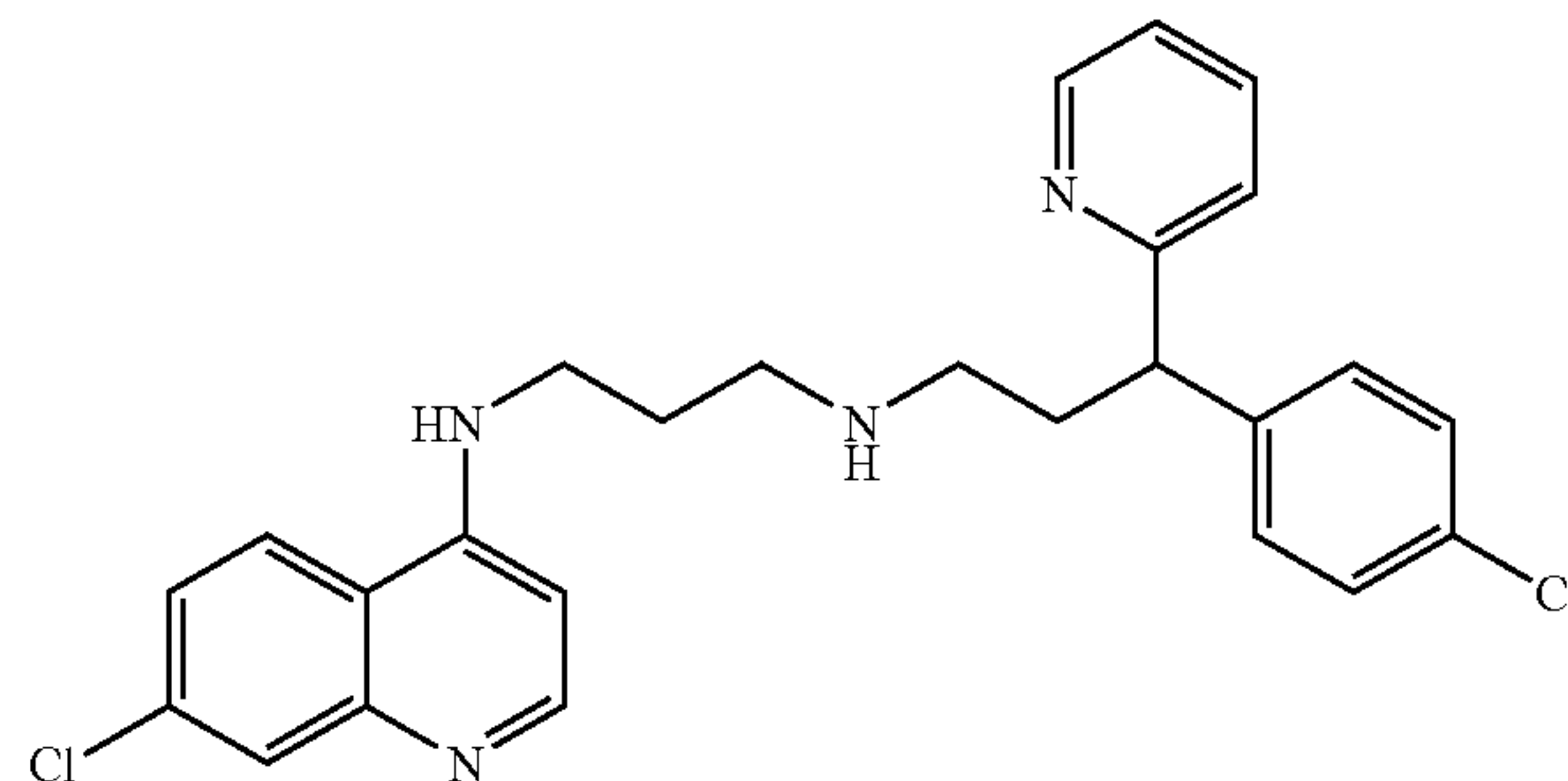
RCQ_101 (a chlorpheniramine derivative)
