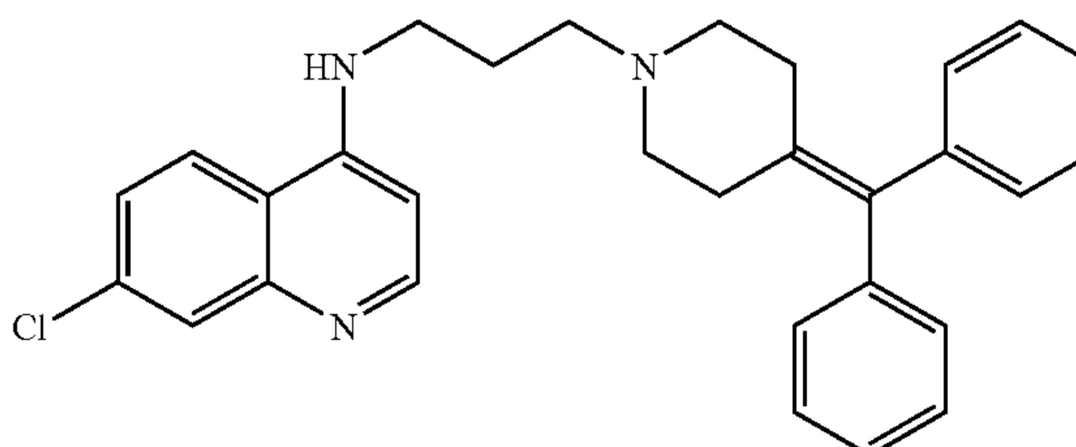
RCQ_116 4-Benzhydrylidene derivative
