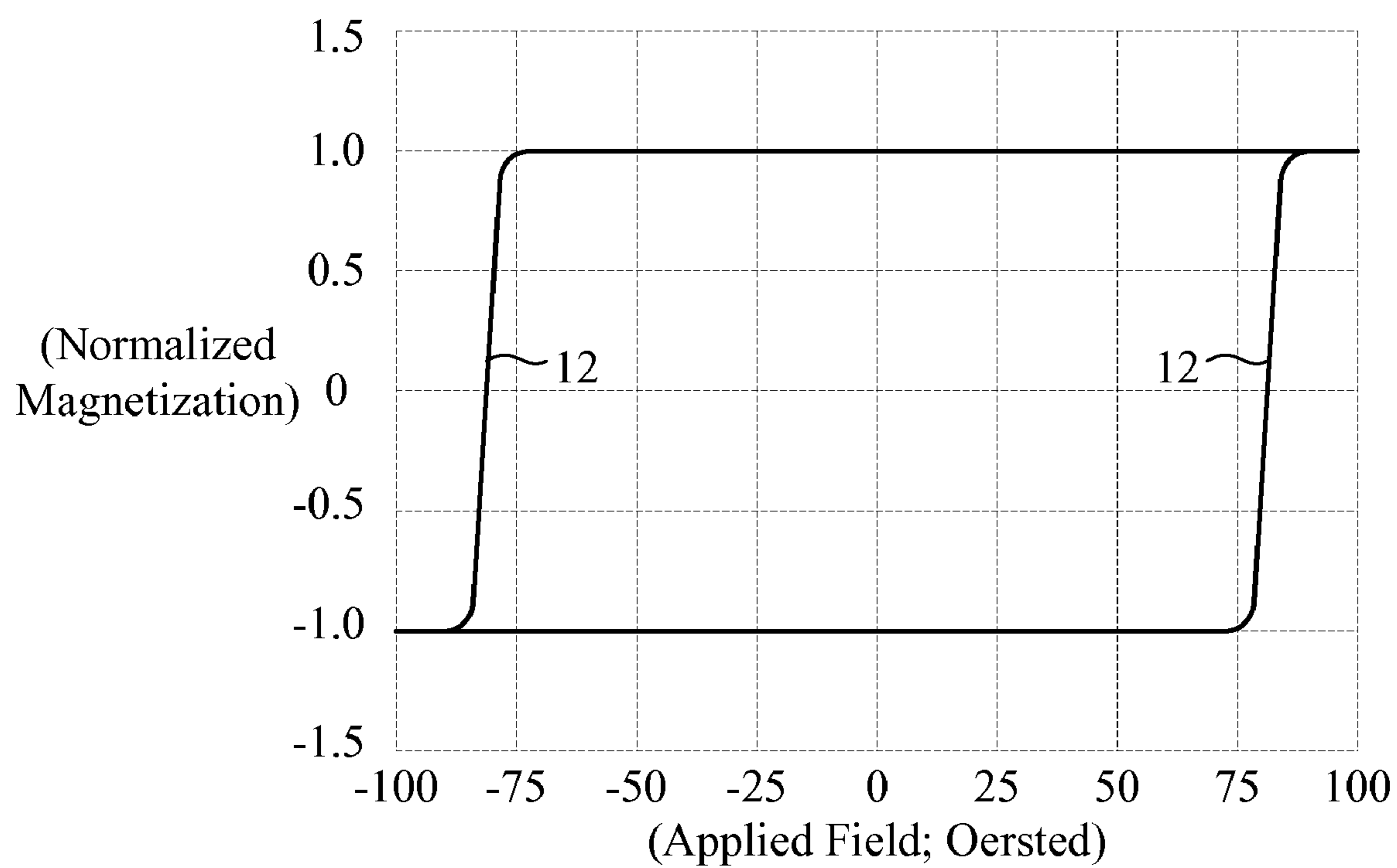
FIG. 7 ( Prior Art )
