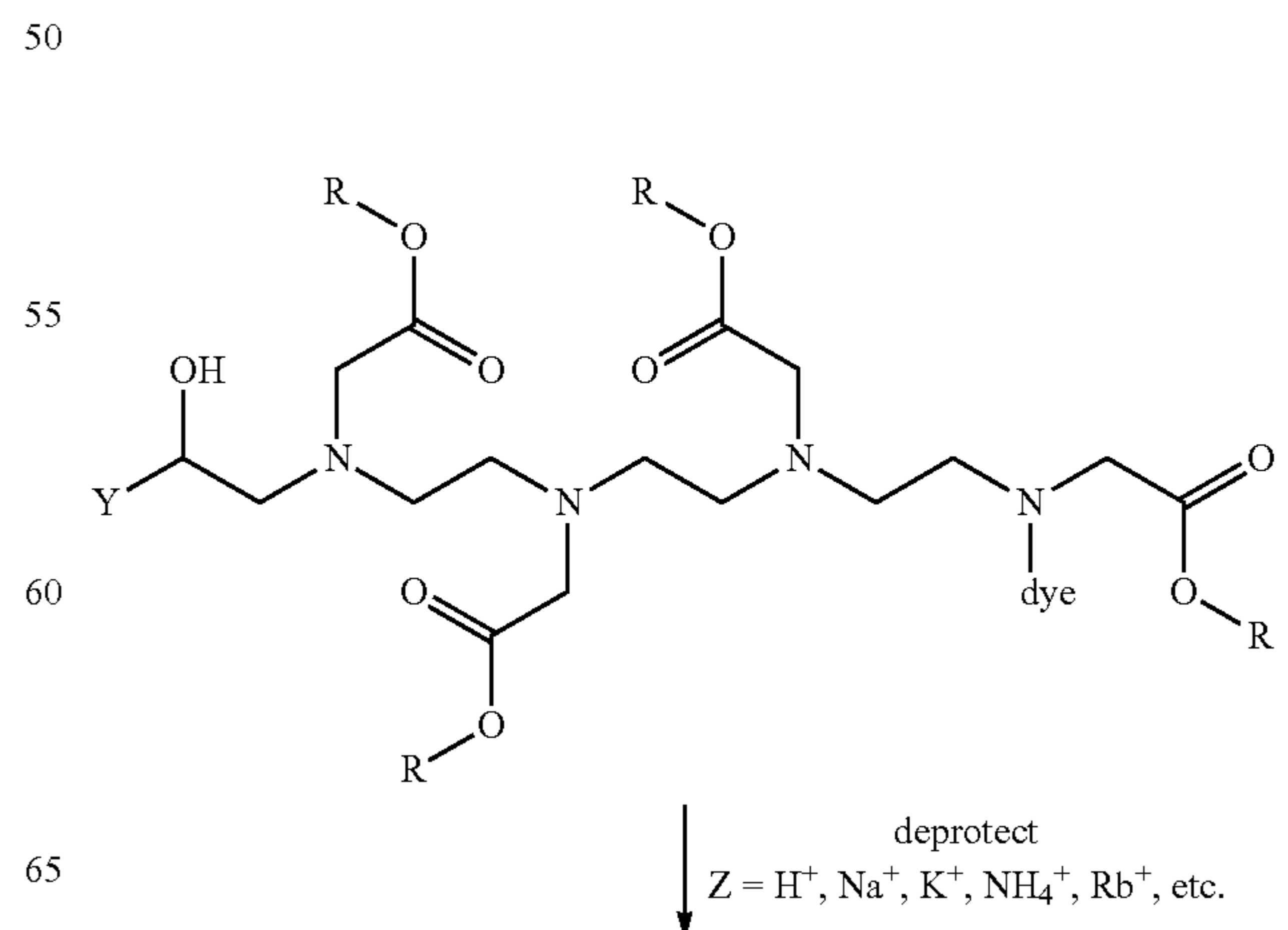
Reaction Scheme 4:
