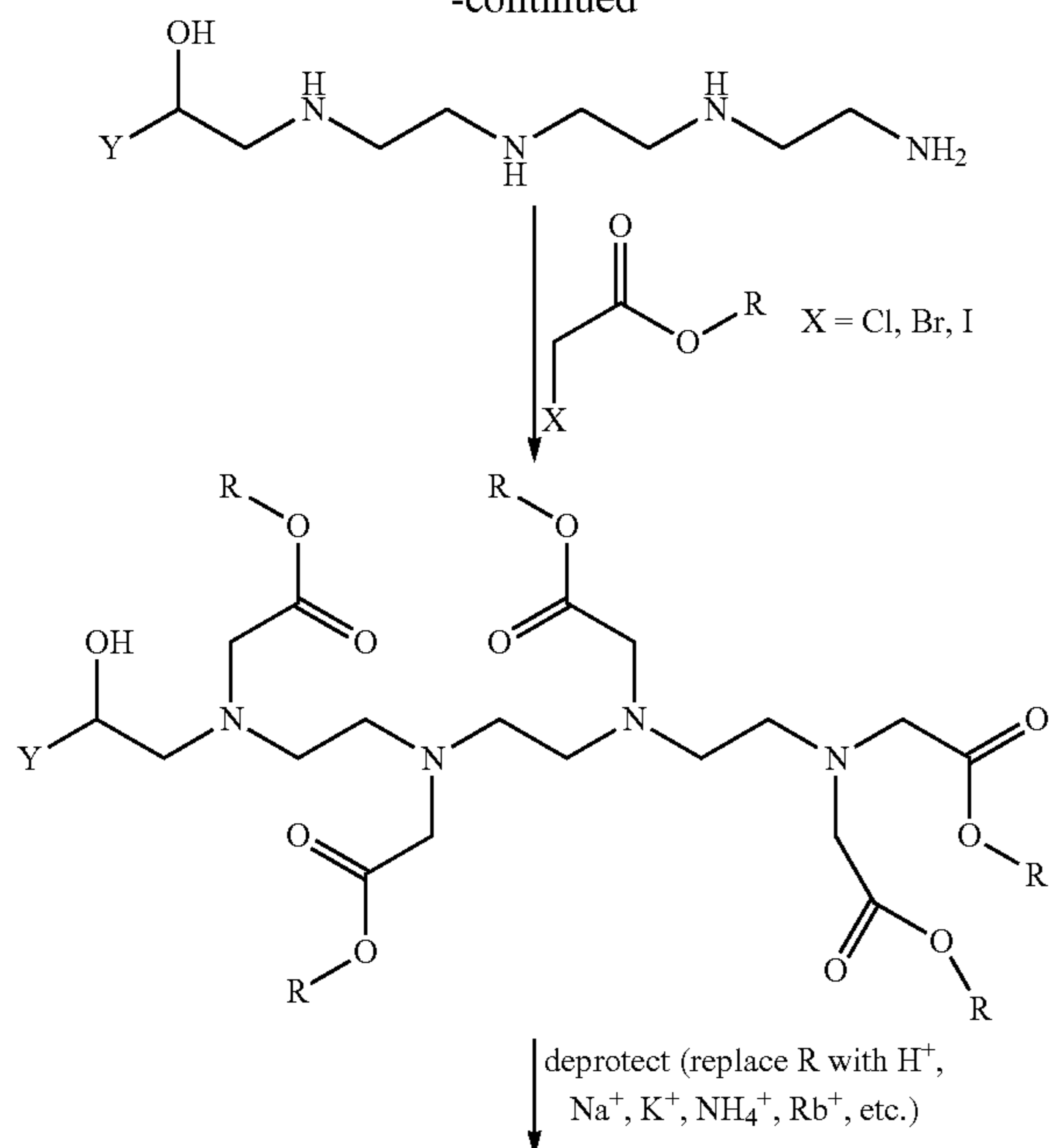
Reaction Scheme 11:
