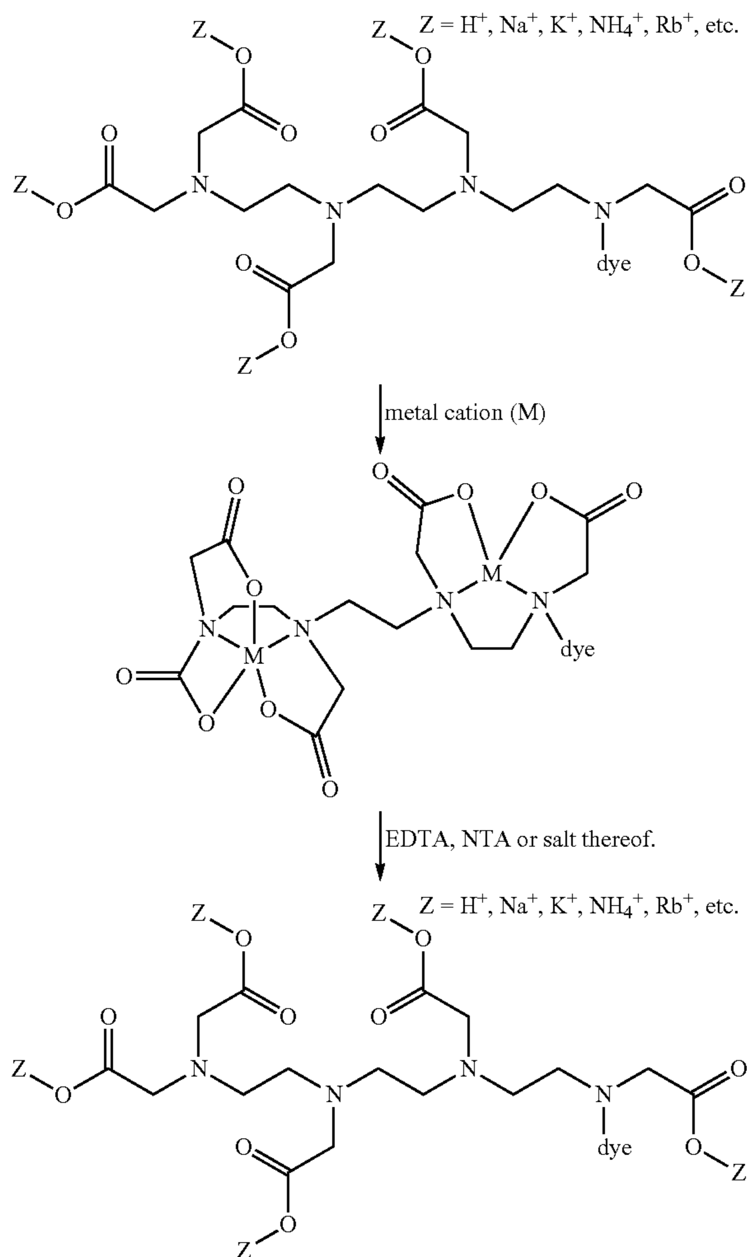
Reaction Scheme 2:
