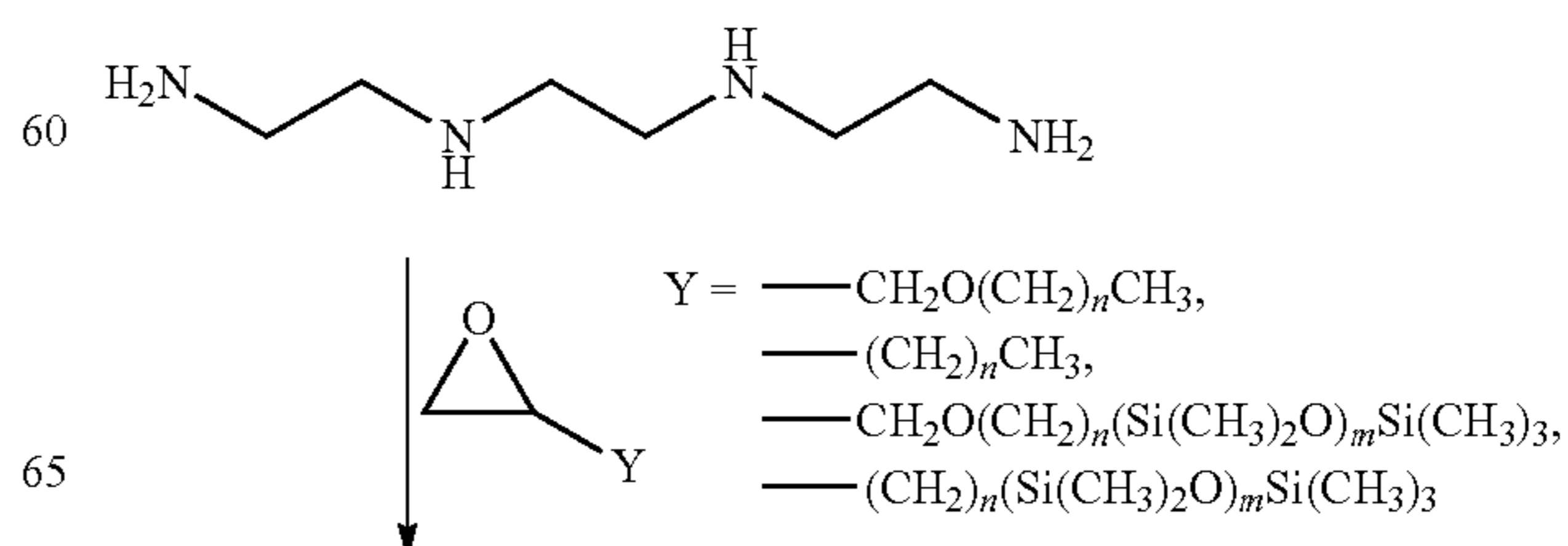
Reaction Scheme 9:
