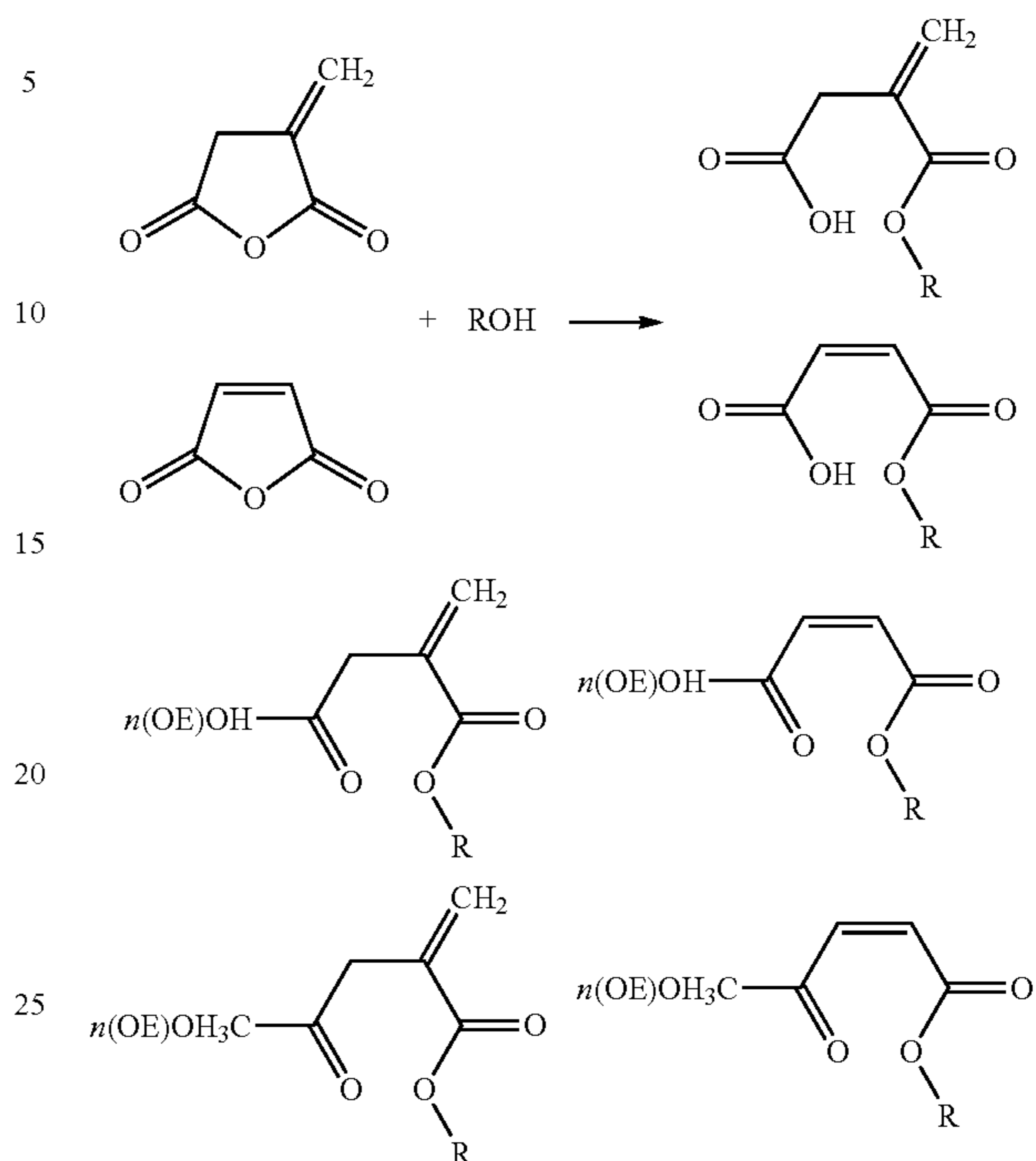
Reaction Scheme 8:
