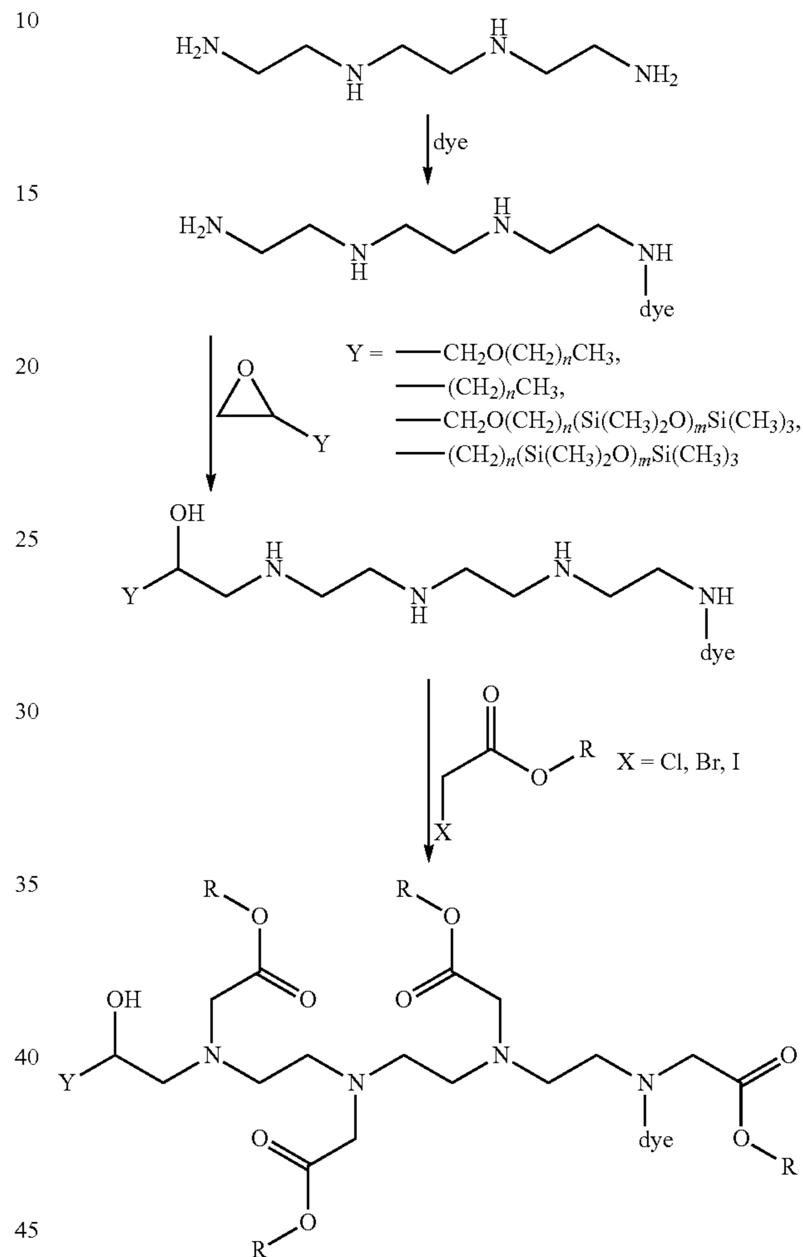
Reaction Scheme 3:
