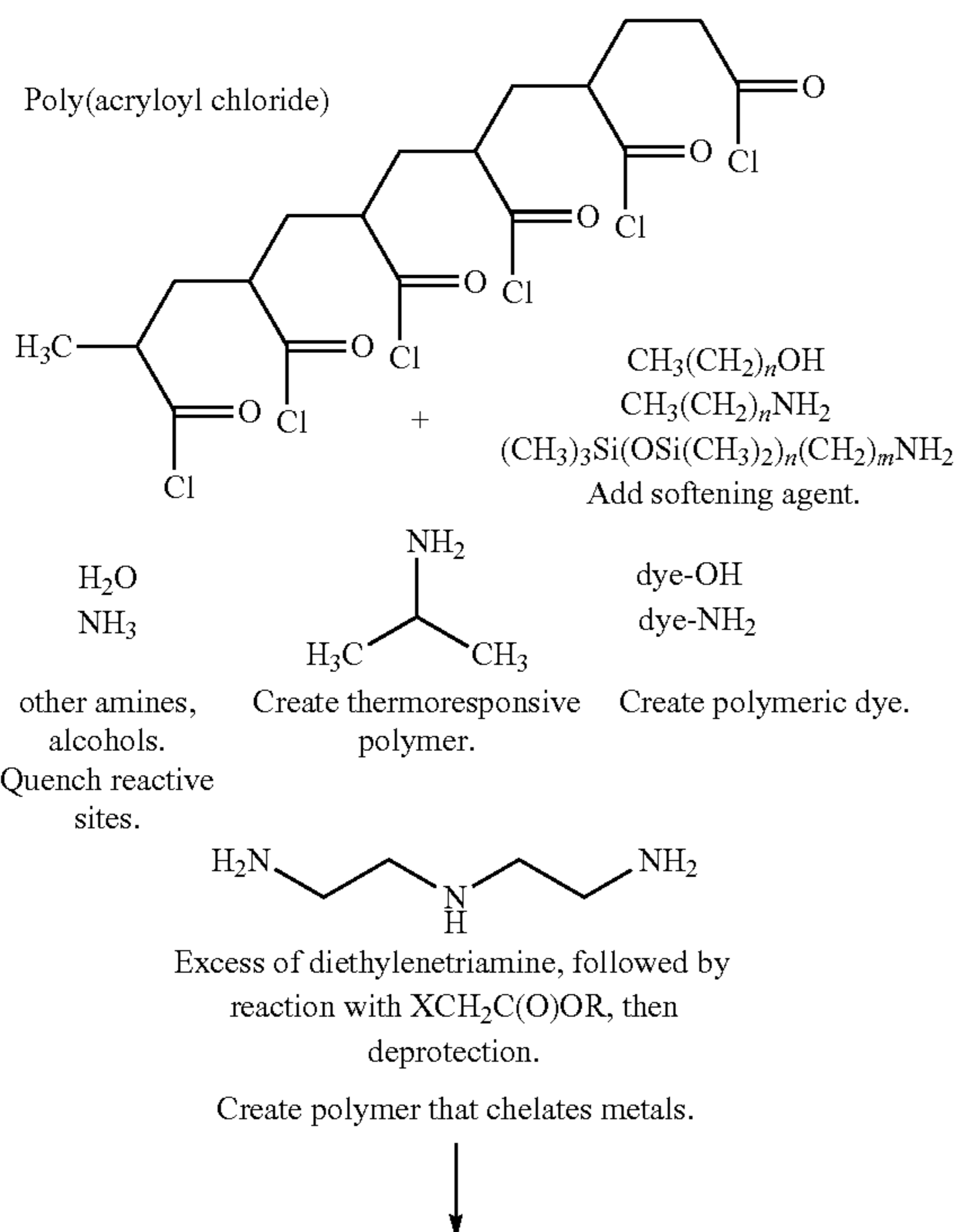
Reaction Scheme 10:
