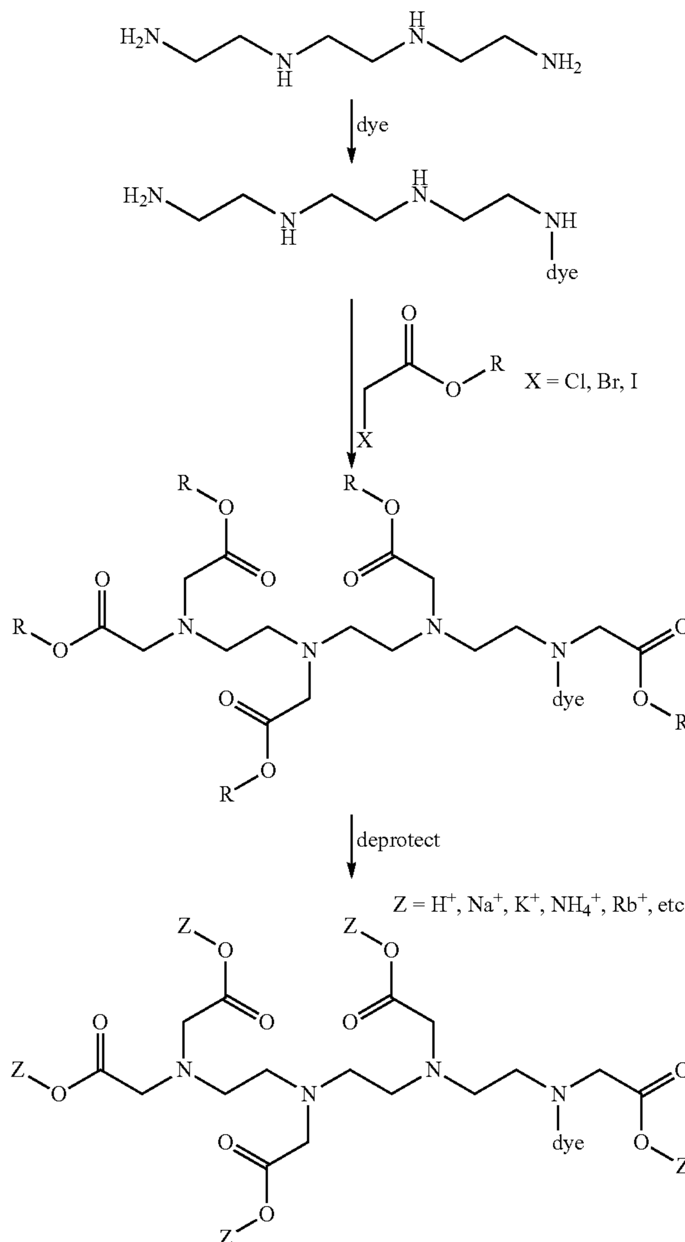
Reaction Scheme 1:
