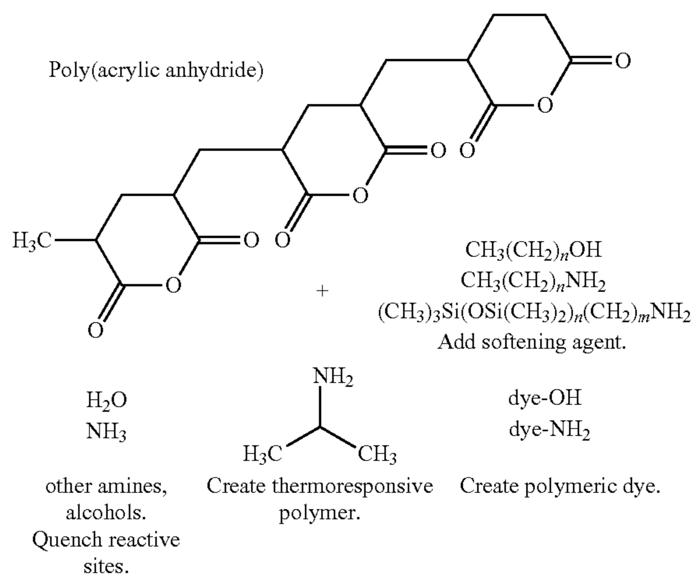
Reaction Scheme 11:
