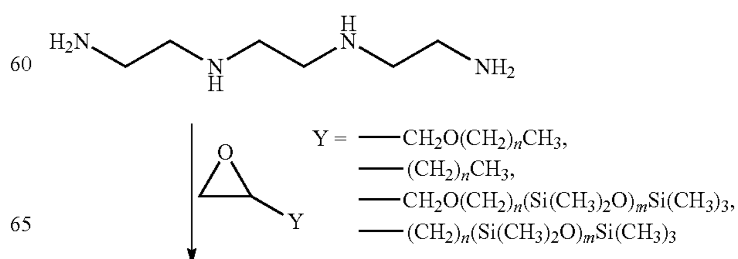
Reaction Scheme 9:
