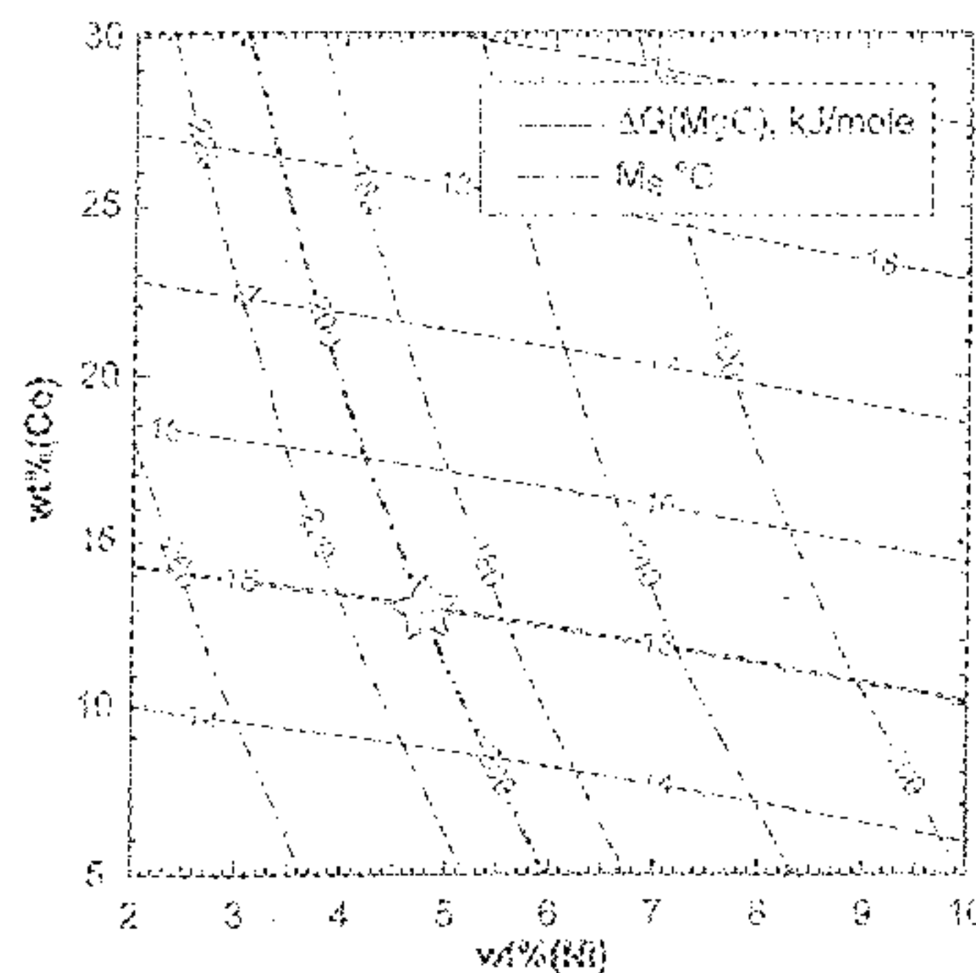
CONTOURS OF M_s TEMPERATURE AND M_2C DRIVING FORCE ( \Delta G ) FOR VARYING COBALT (CO) AND NICKEL (NI) CONTENTS. WHERE TEMPERATURE HAS BEEN SET TO +820^\circ C , AND OTHER ALLOYING ELEMENT AMOUNTS HAVE BEEN SET TO, BY WEIGHT: 0.14% C, 9% Cr, 1.5% Nb, AND 0.5% V.
