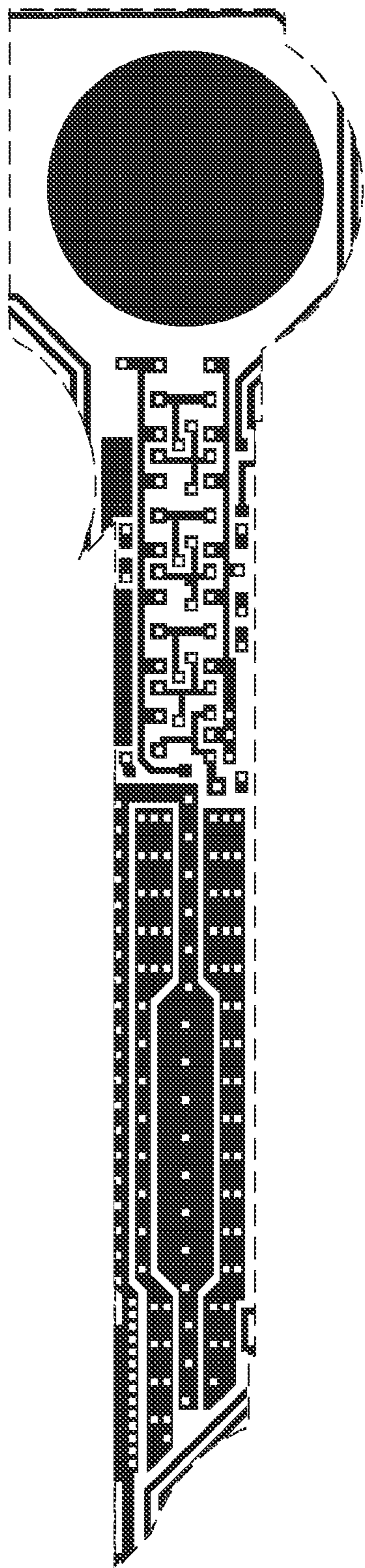
Metal 1 mask
