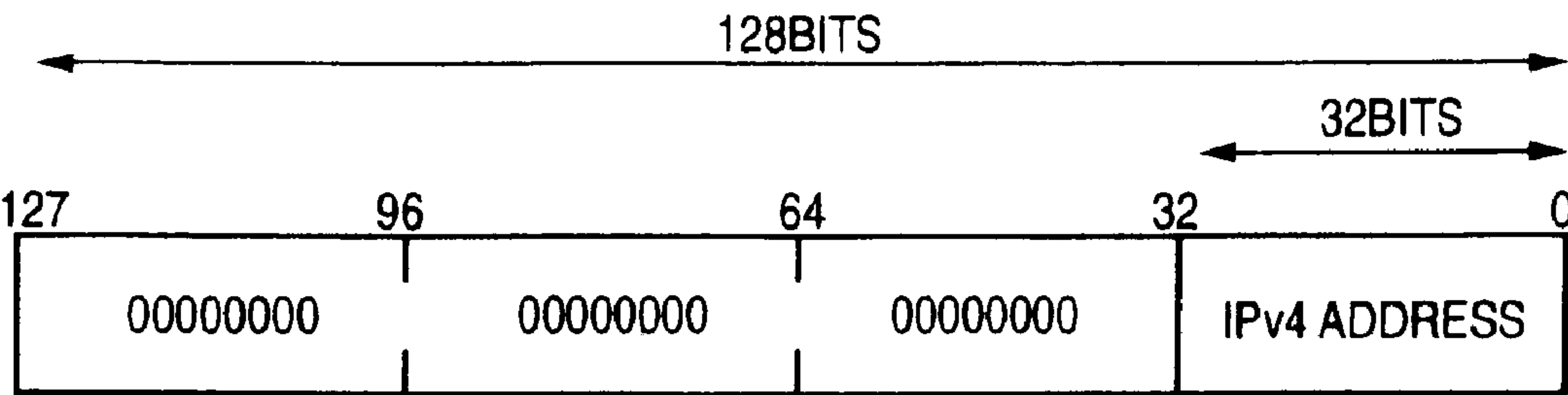
FIG. 12A IPv6 ADDRESS FOR INTERCONNECTION BETWEEN V6 NODE AND V4 NODE IPv4-compatible IPv6 ADDRESS
