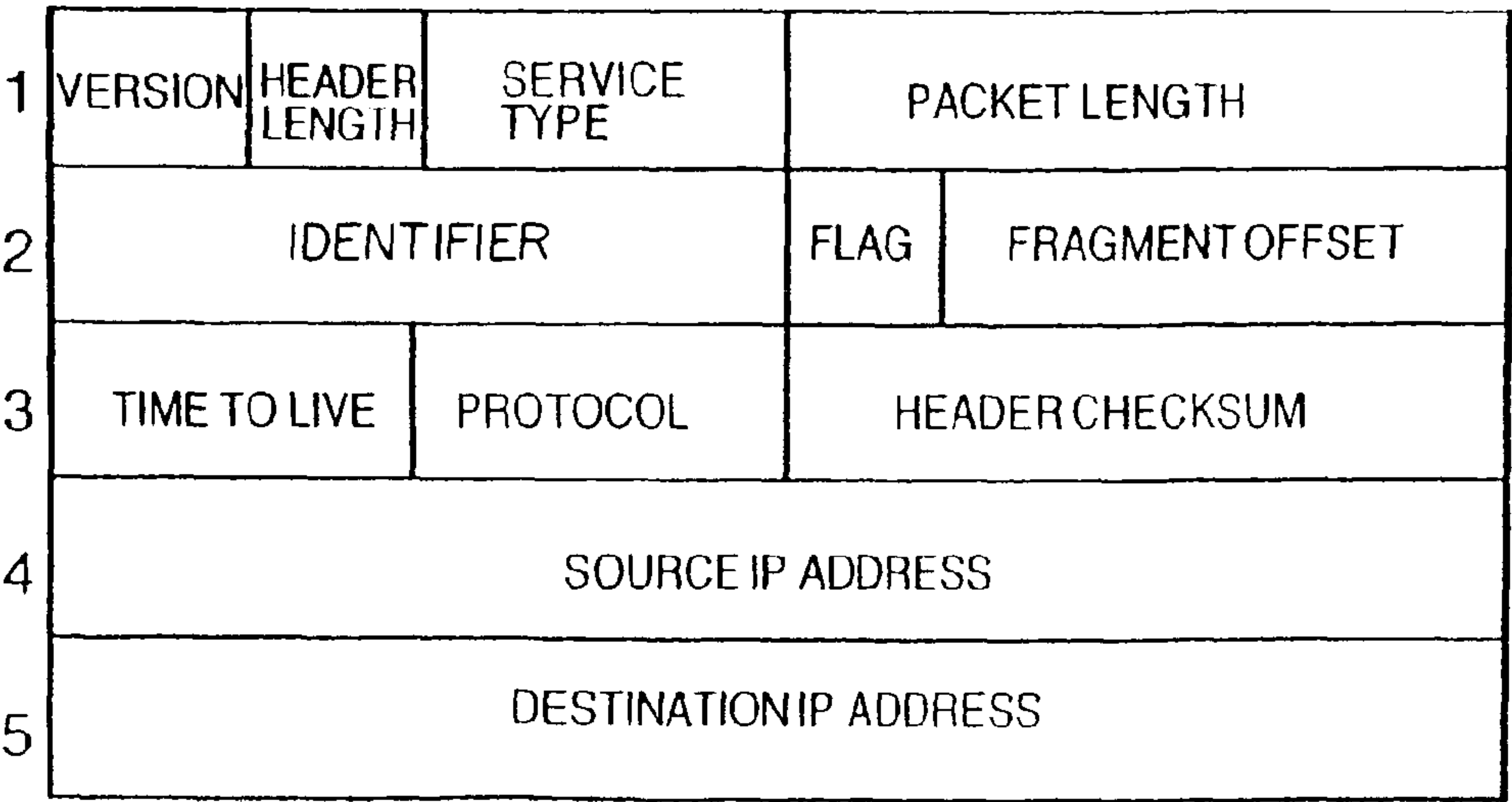
IPv4 HEADER FORMAT
