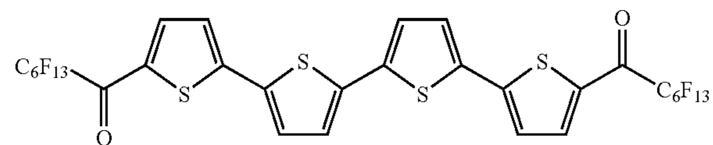
Ib (DHCO-4T)
