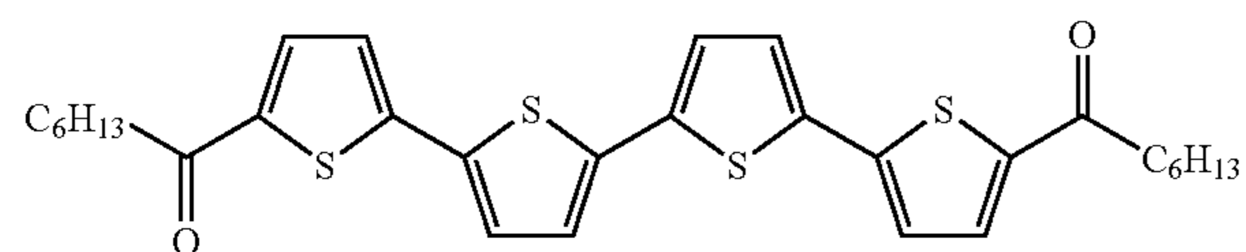
Ia (DFHCO-4T)
