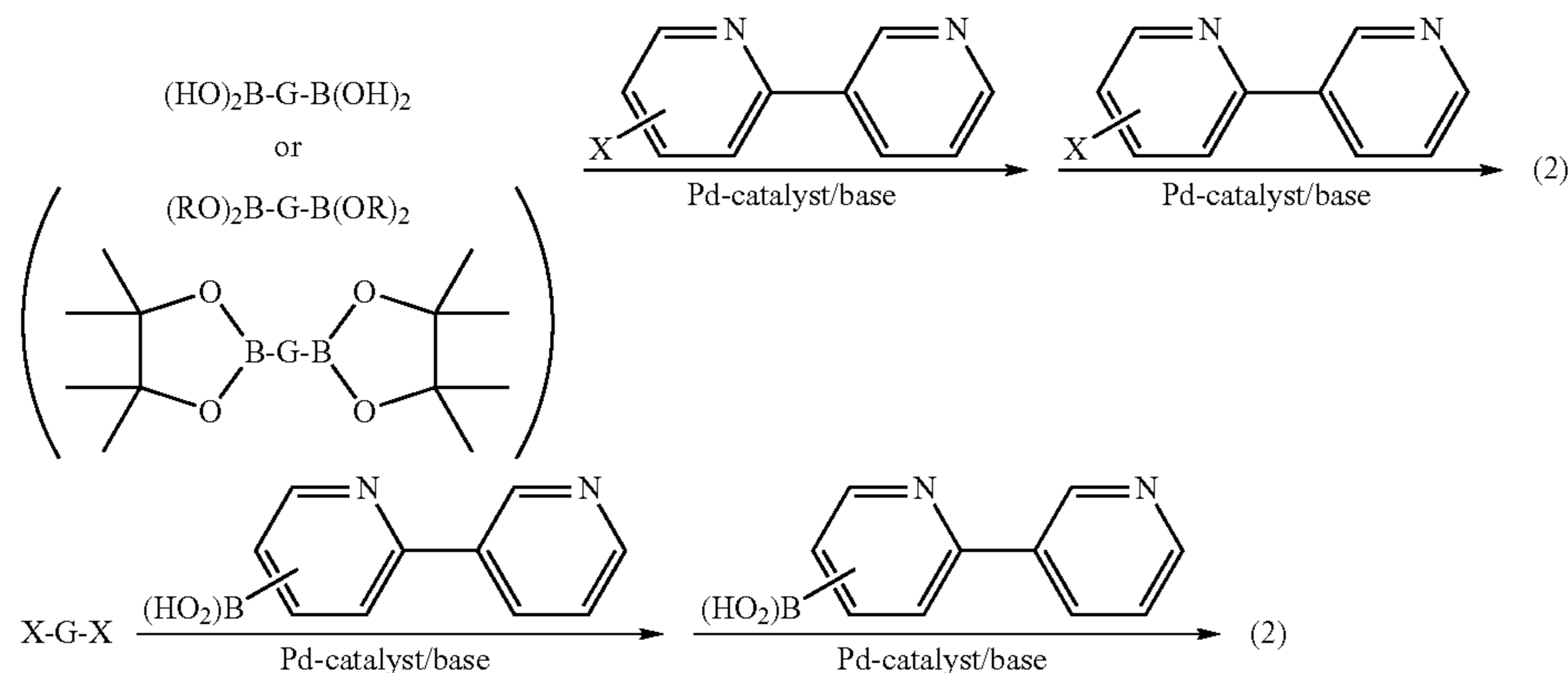
Scheme 1: Suzuki coupling
