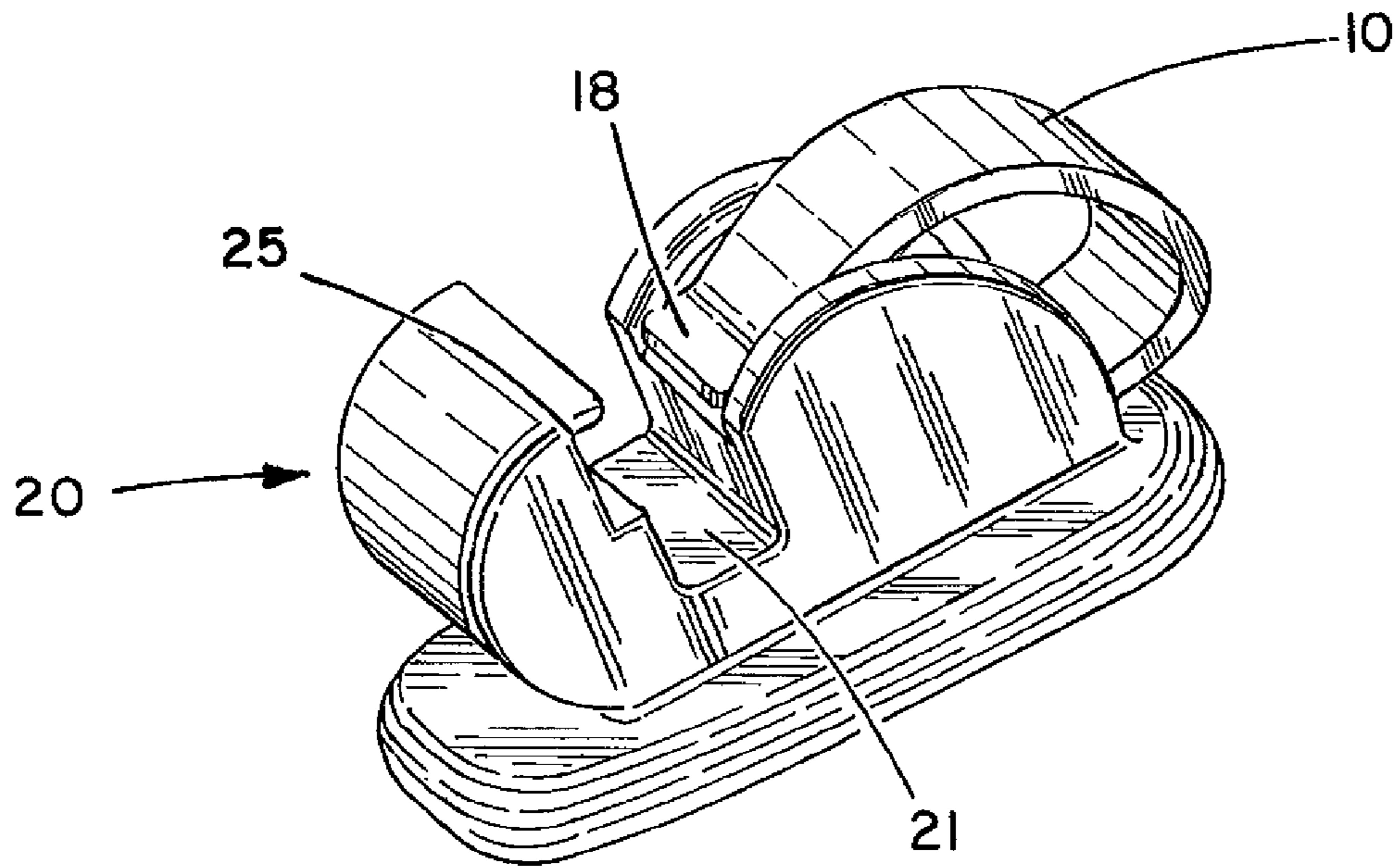
Fig. 3 (Prior Art)
