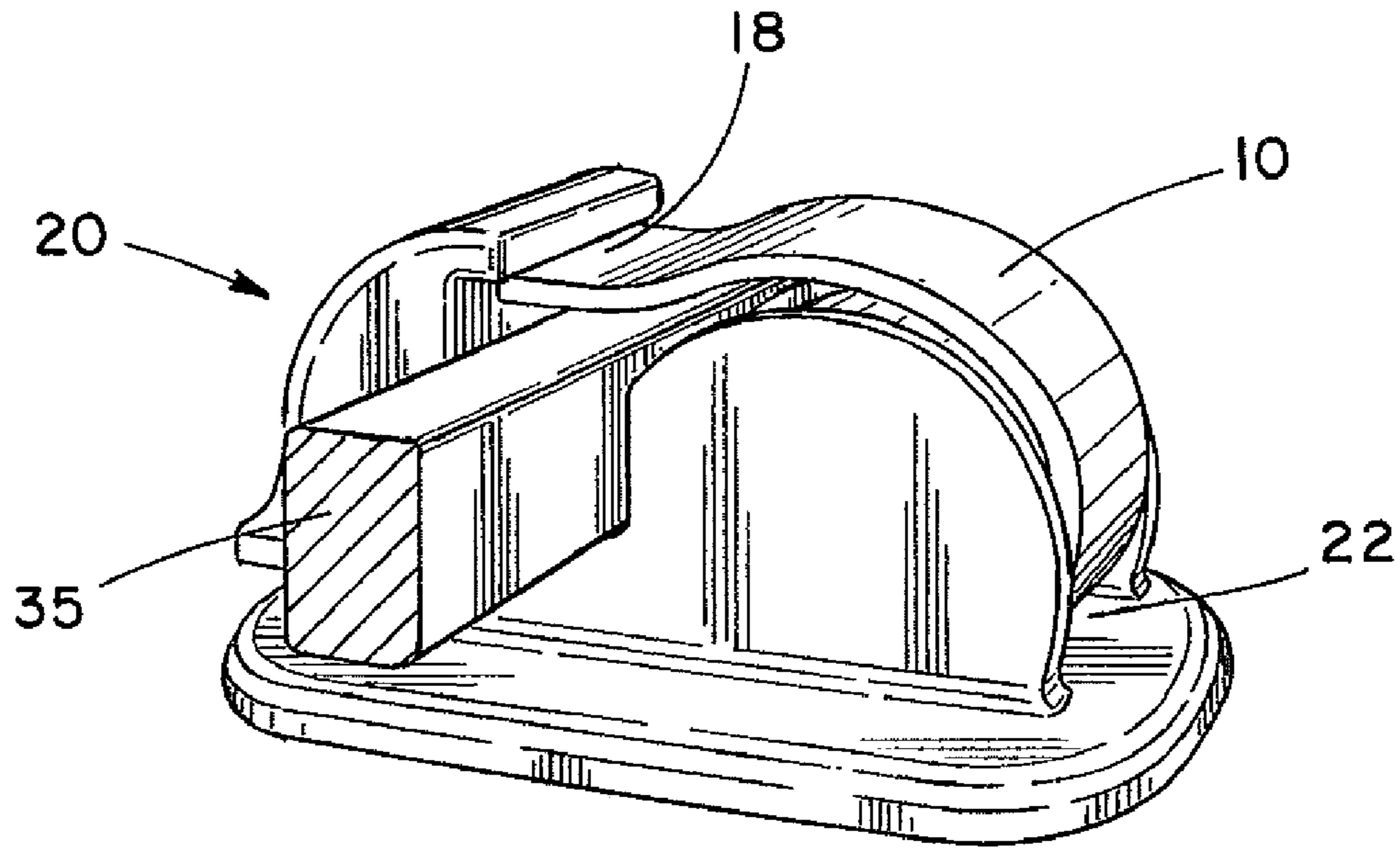
Fig. 7 (Prior Art)
