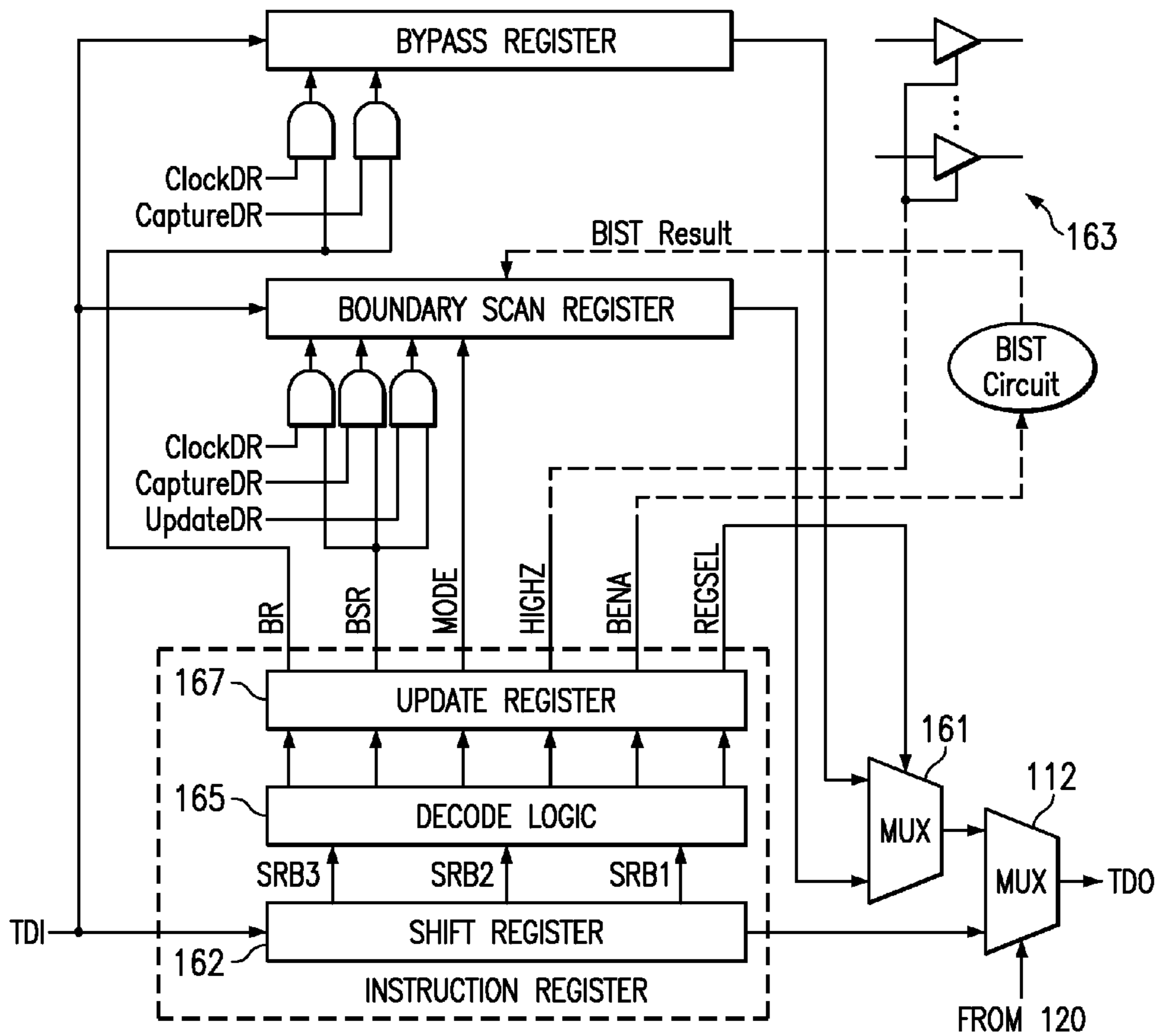
FIG. 16 (PRIOR ART)
