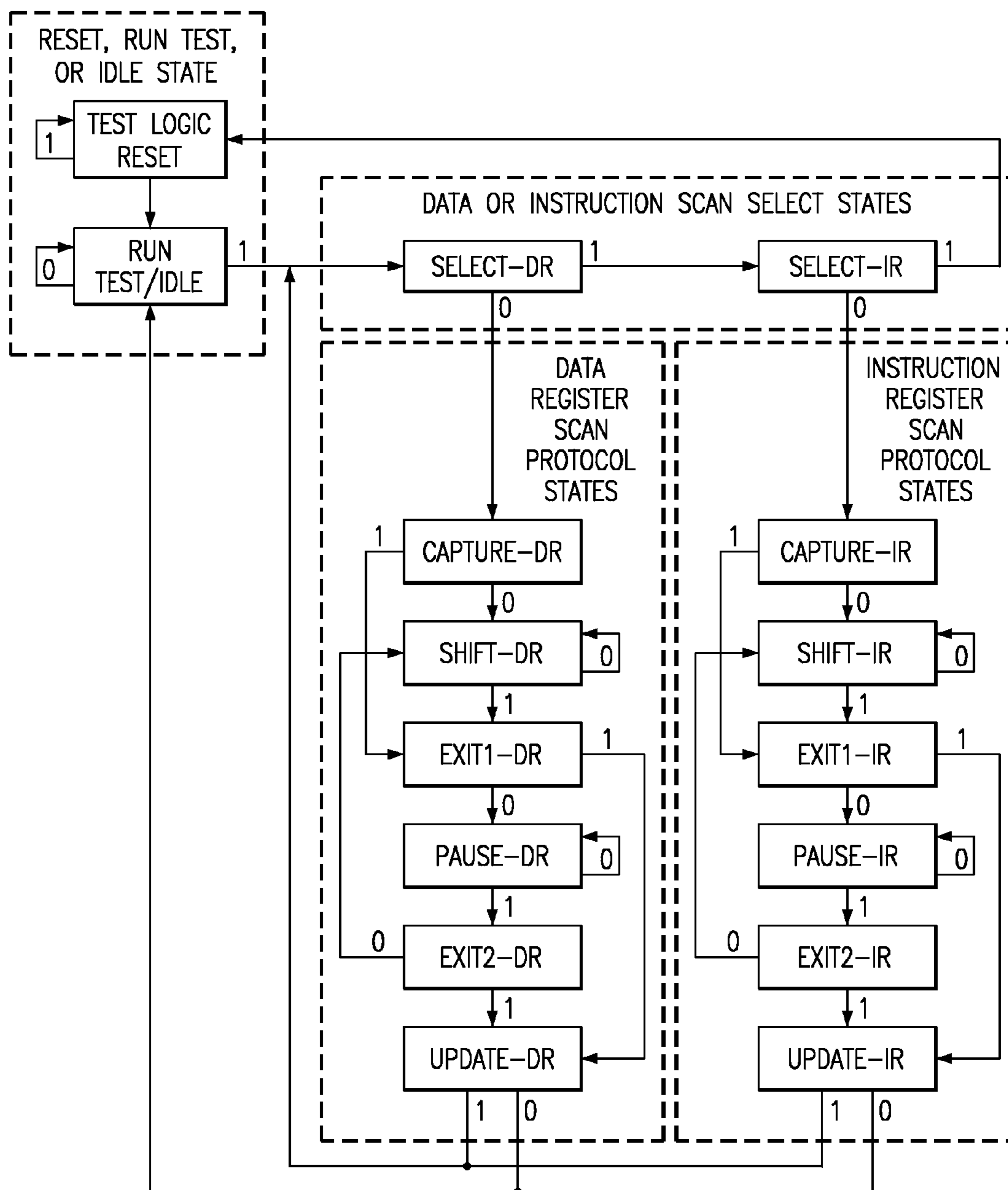
FIG. 2 (PRIOR ART)
