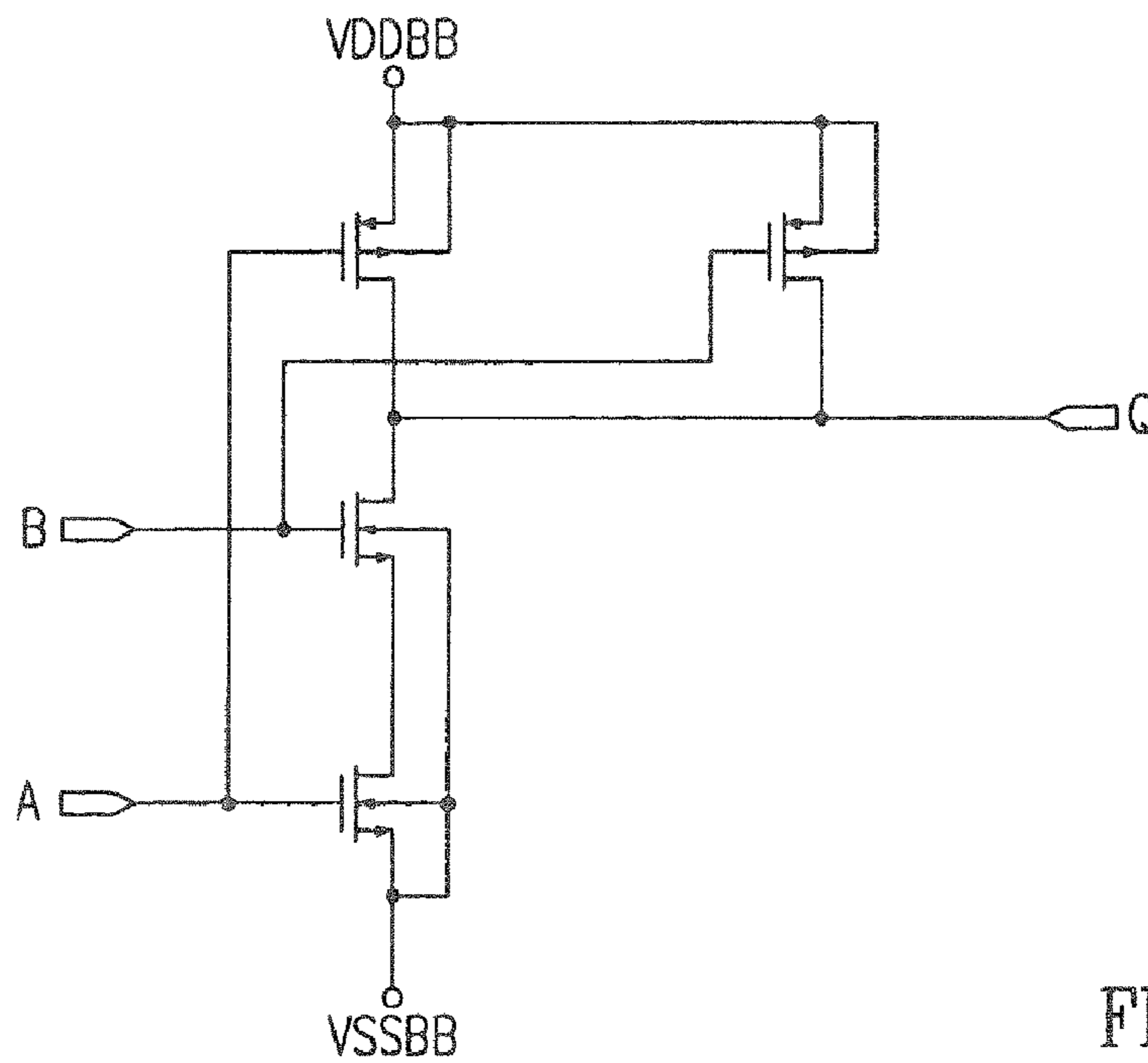
NAND2
