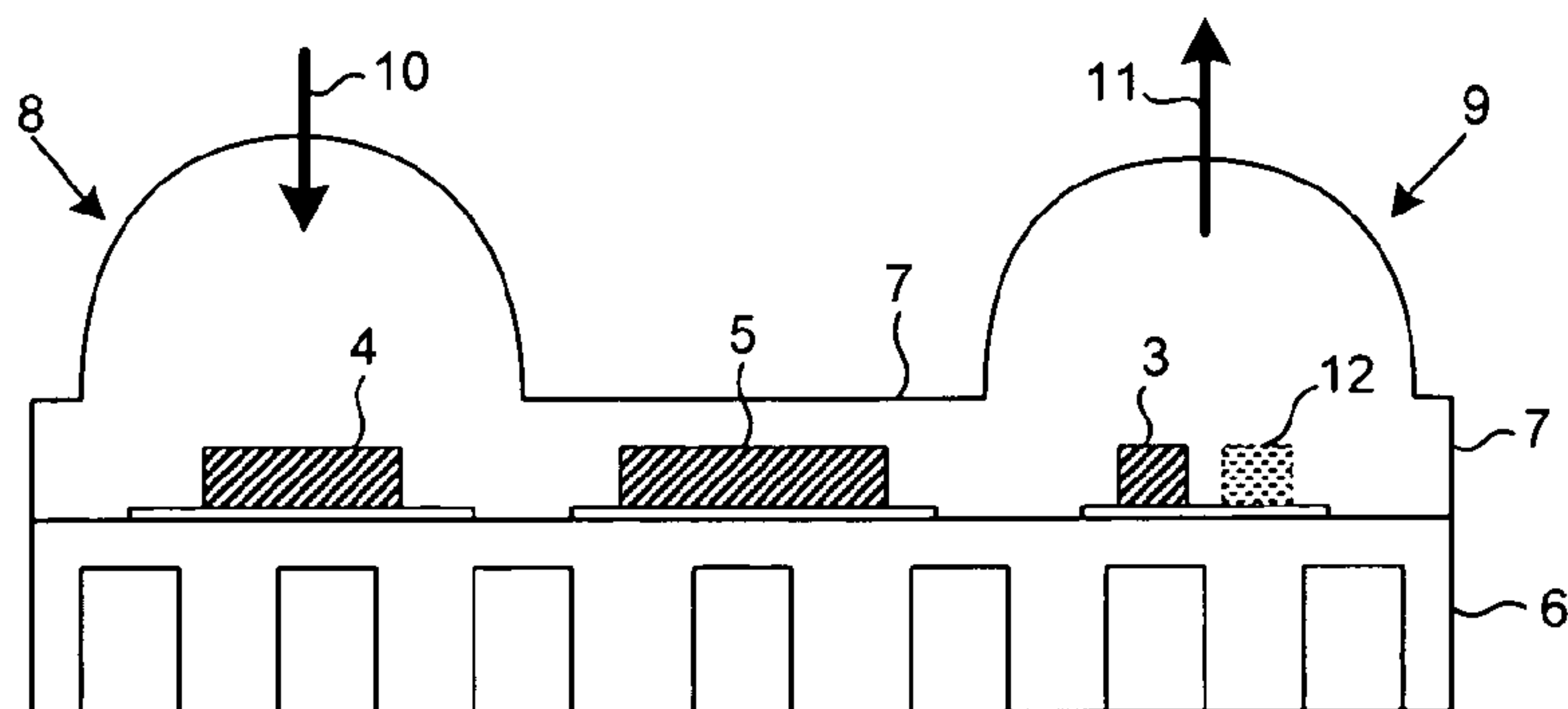
FIG. 2 (PRIOR ART)
