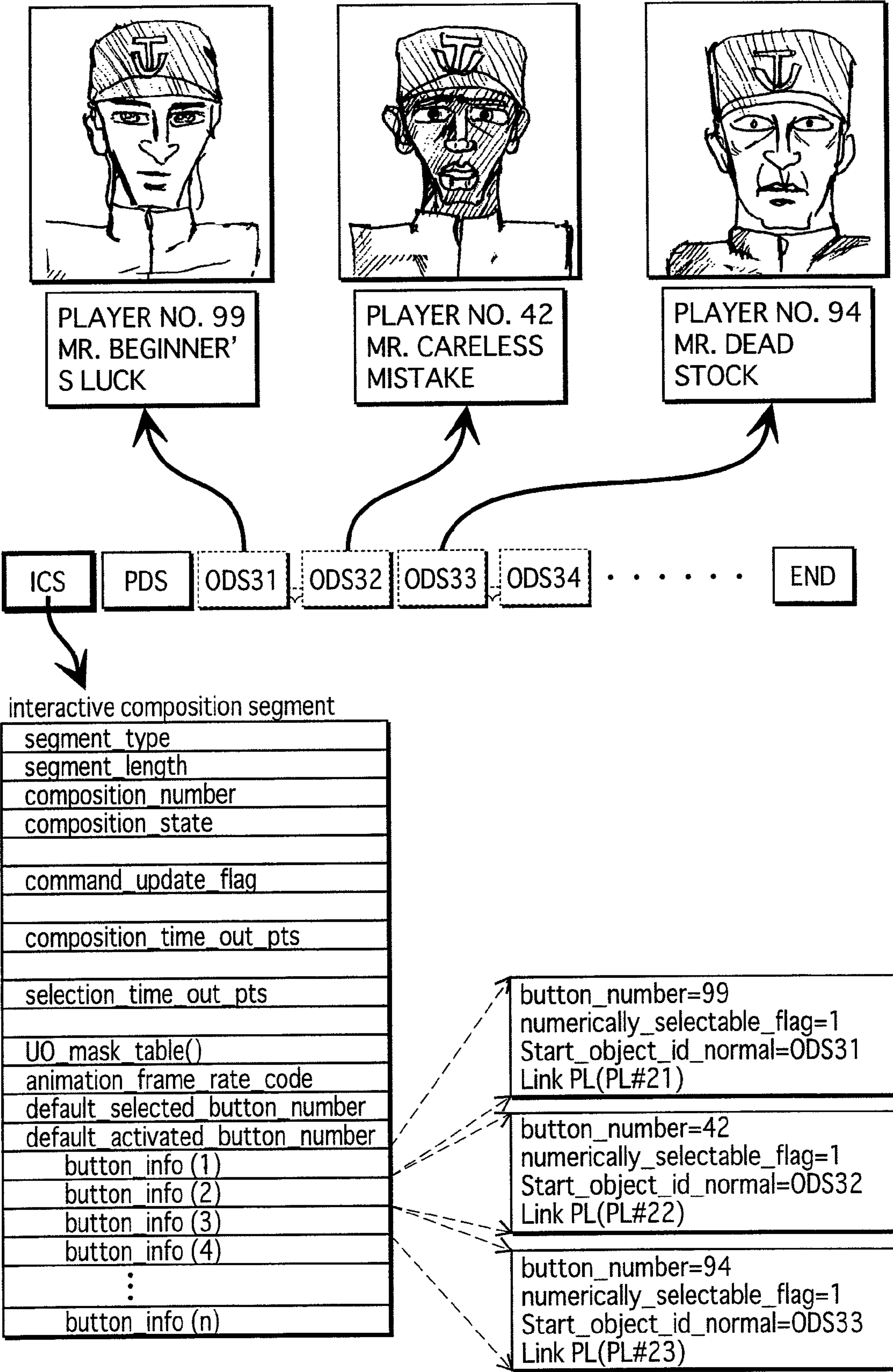
FIG. 18 PLAYERS LIST
