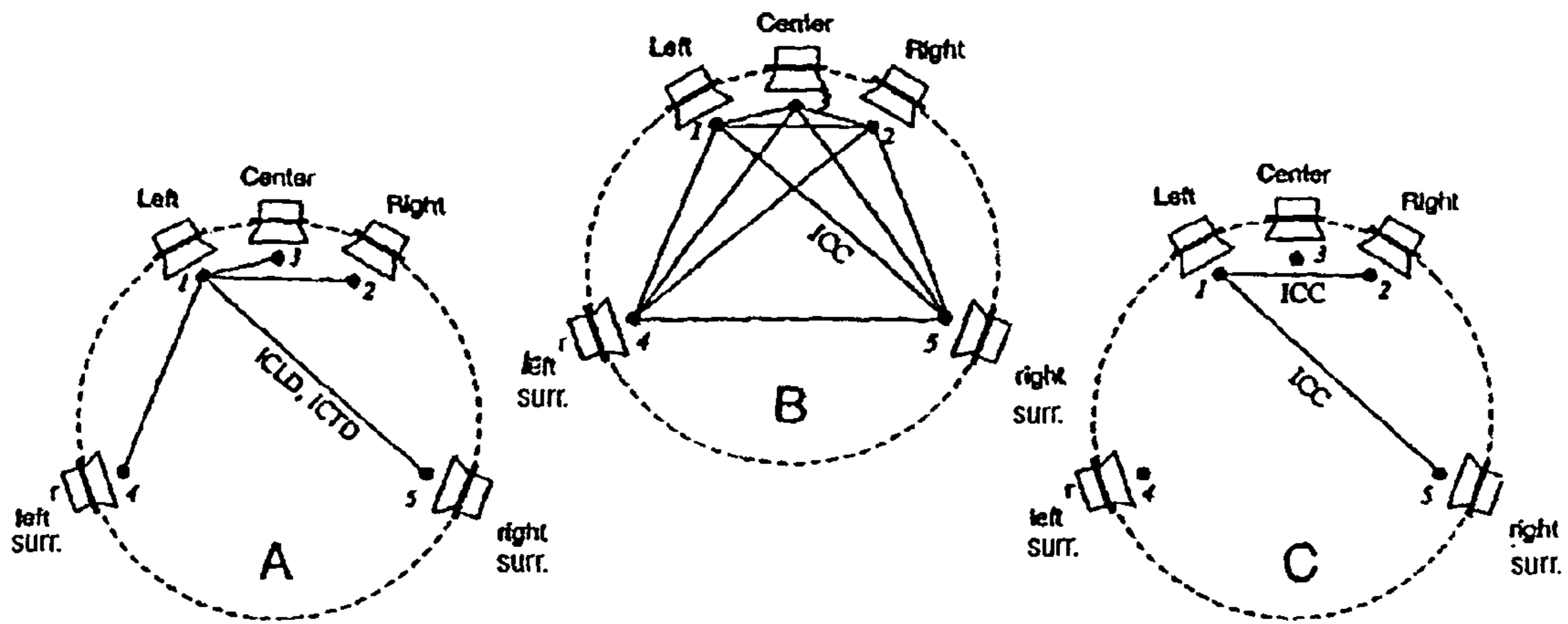
FIG 14 (Prior Art)
