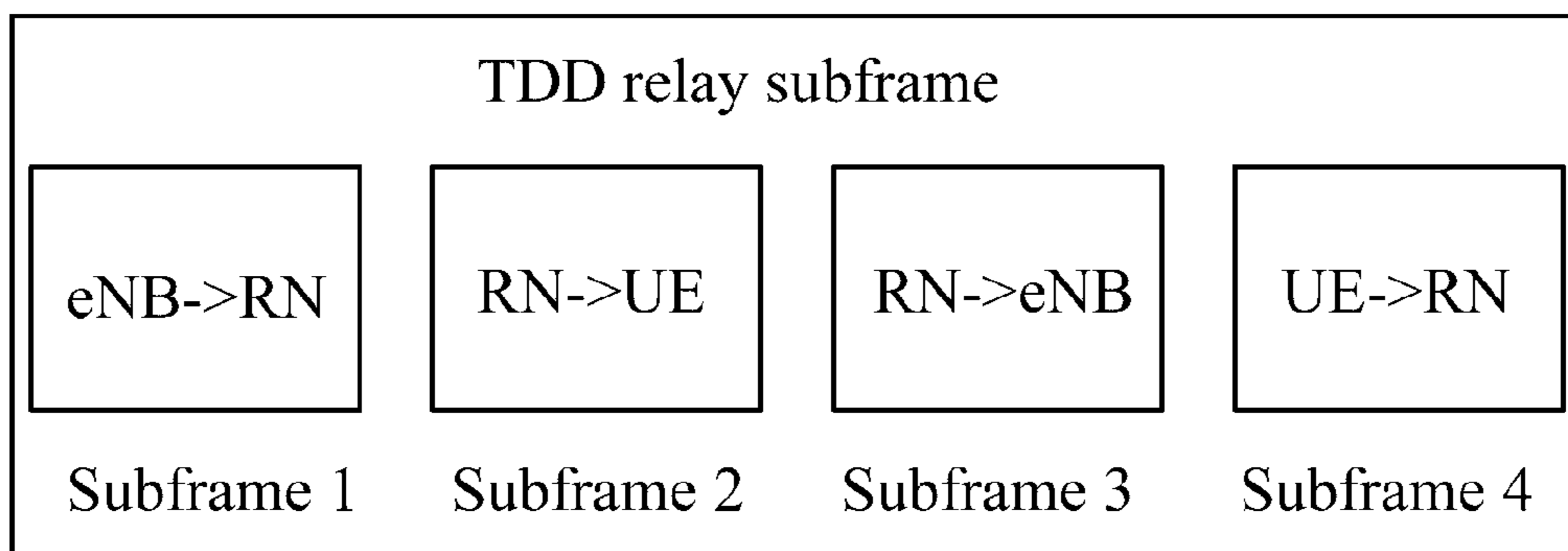
FIG. 1 (Prior Art)
