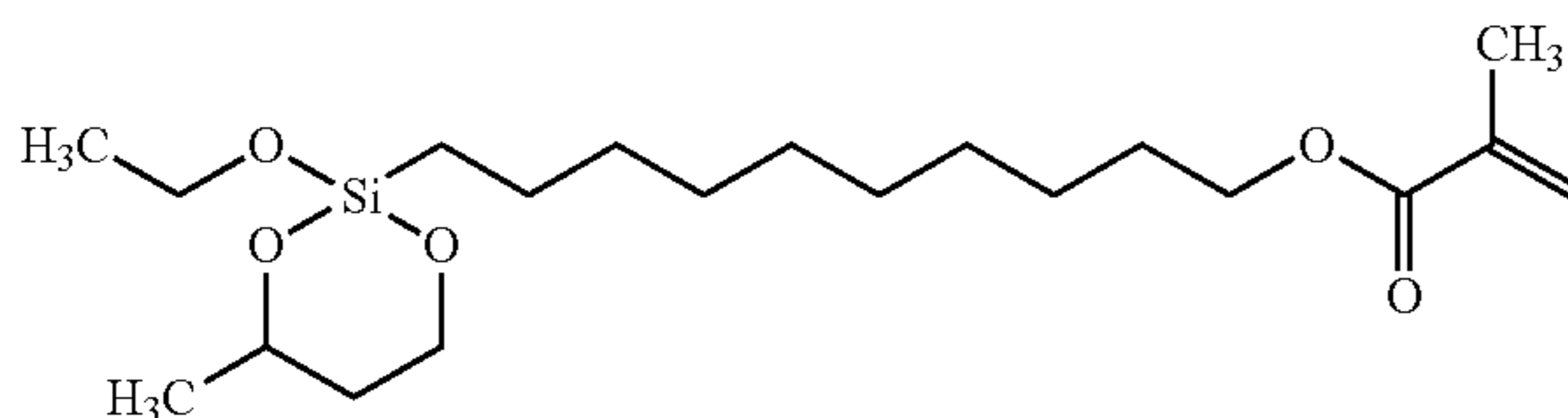
10-(1,3-butanedi-alkoxyethoxysilyl)-1-decyl methacrylate; and
