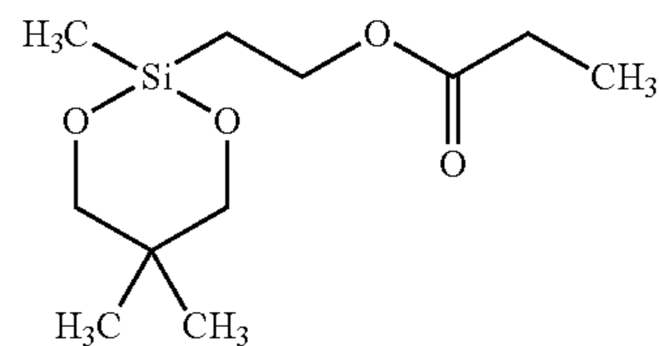
2-(neopentylglycoxy methylsilyl)-1-ethyl propionate;
