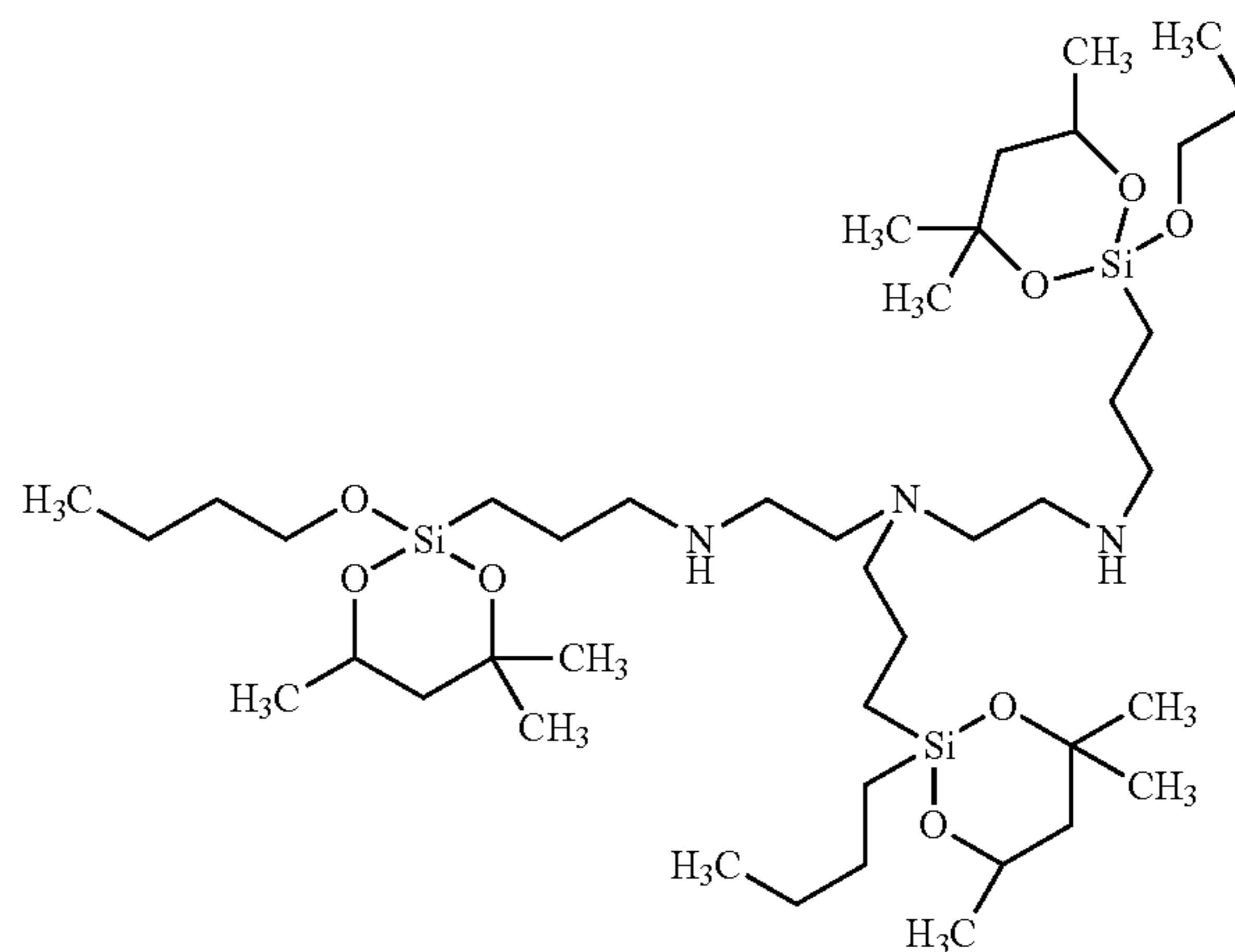
tris-N,N',N''-[3-(2-methyl-2,4-pentanedialkoxybutoxysilyl)-1-propyl] diethylene triamine;
