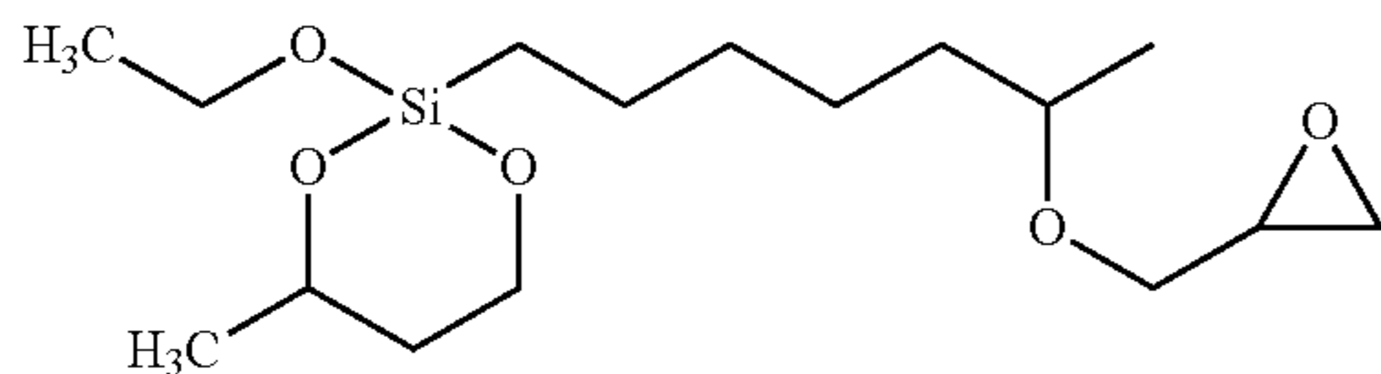
1-(1,3-butanedi-alkoxyethoxysilyl)-5-hexyl glycidyl ether;
