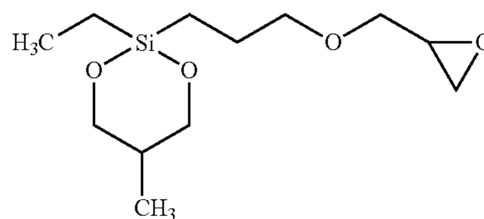
3-(2-methyl-1,3-propanedioxyethylsilyl)-1-propyl glycidyl ether;
