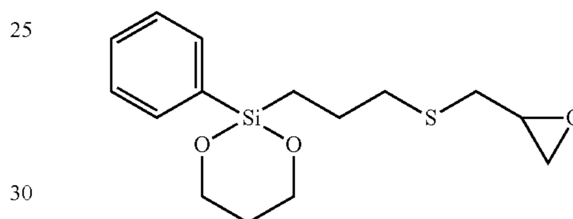
3-(1,3-propanedioldialkoxyphenylsilyl)-1-propyl glycidyl thioether;
