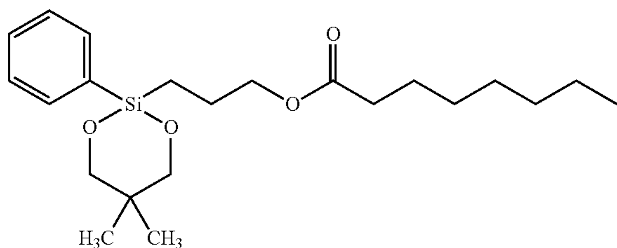
3-(neopentyl glycoxyphenylsilyl)-1-propyl octanoate;
