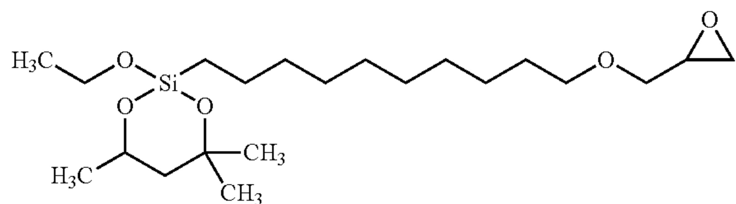
10-(2-methyl-2,4-pentanedialkoxyethoxysilyl)-1-decyl glycidyl ether;
