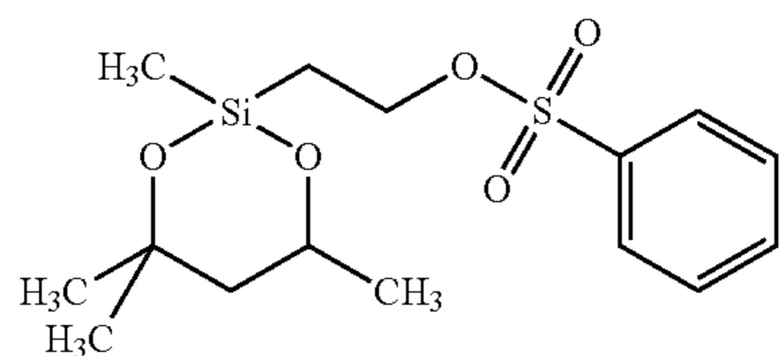
2-(2-methyl-2,4-pentanedialkoxy methylsilyl)-1-ethyl benzenesulfonate;
