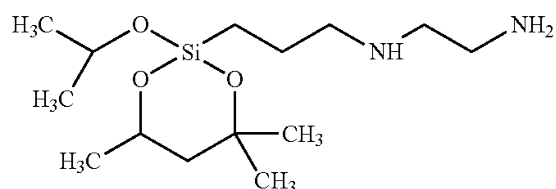
N-[3-(2-methyl-2,4-pentanedialkoxyisopropoxysilyl)-1-propyl] ethylene diamine;
