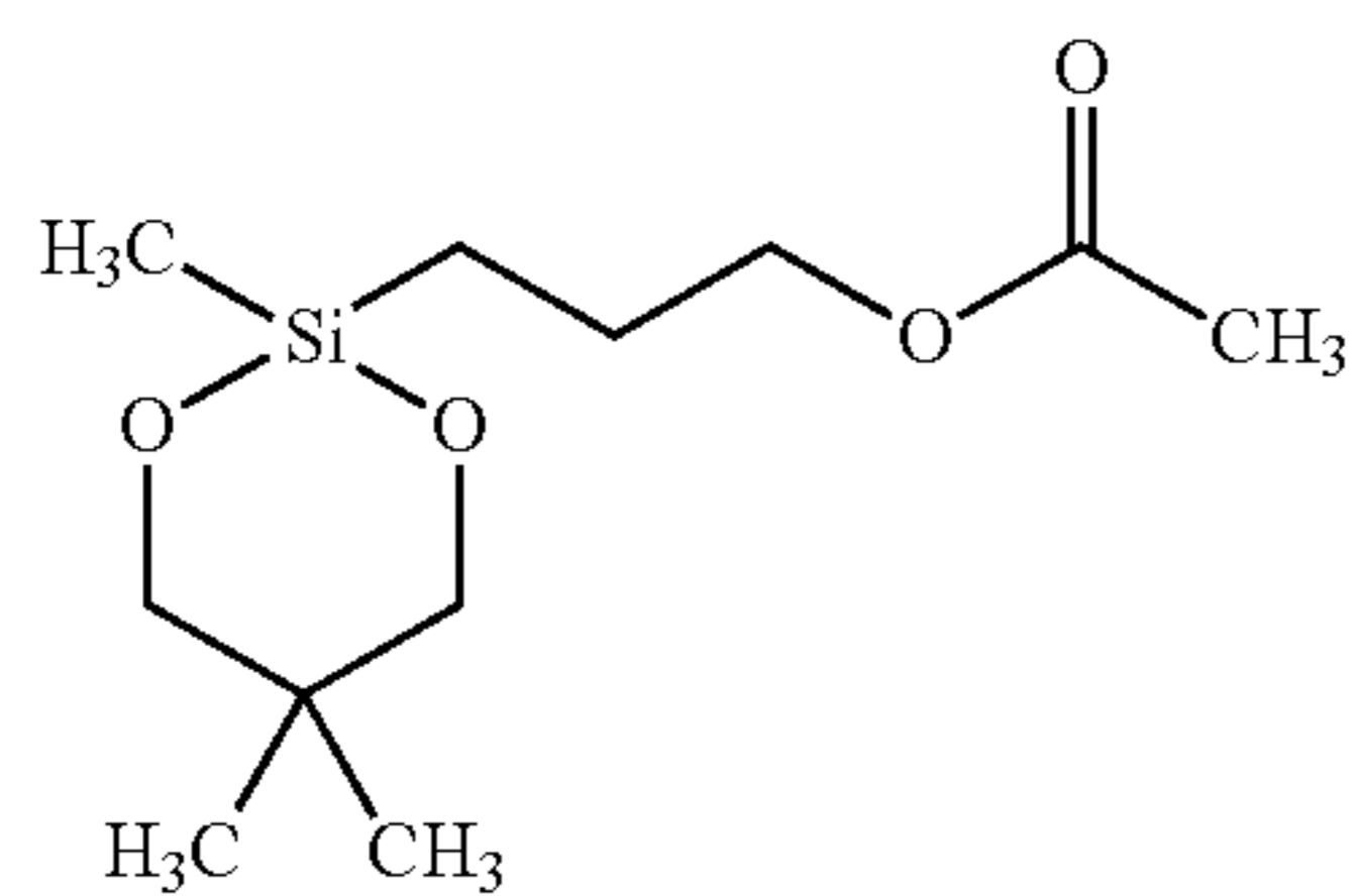
3-(neopentyl glycoxymethylsilyl)-1-propyl acetate;
