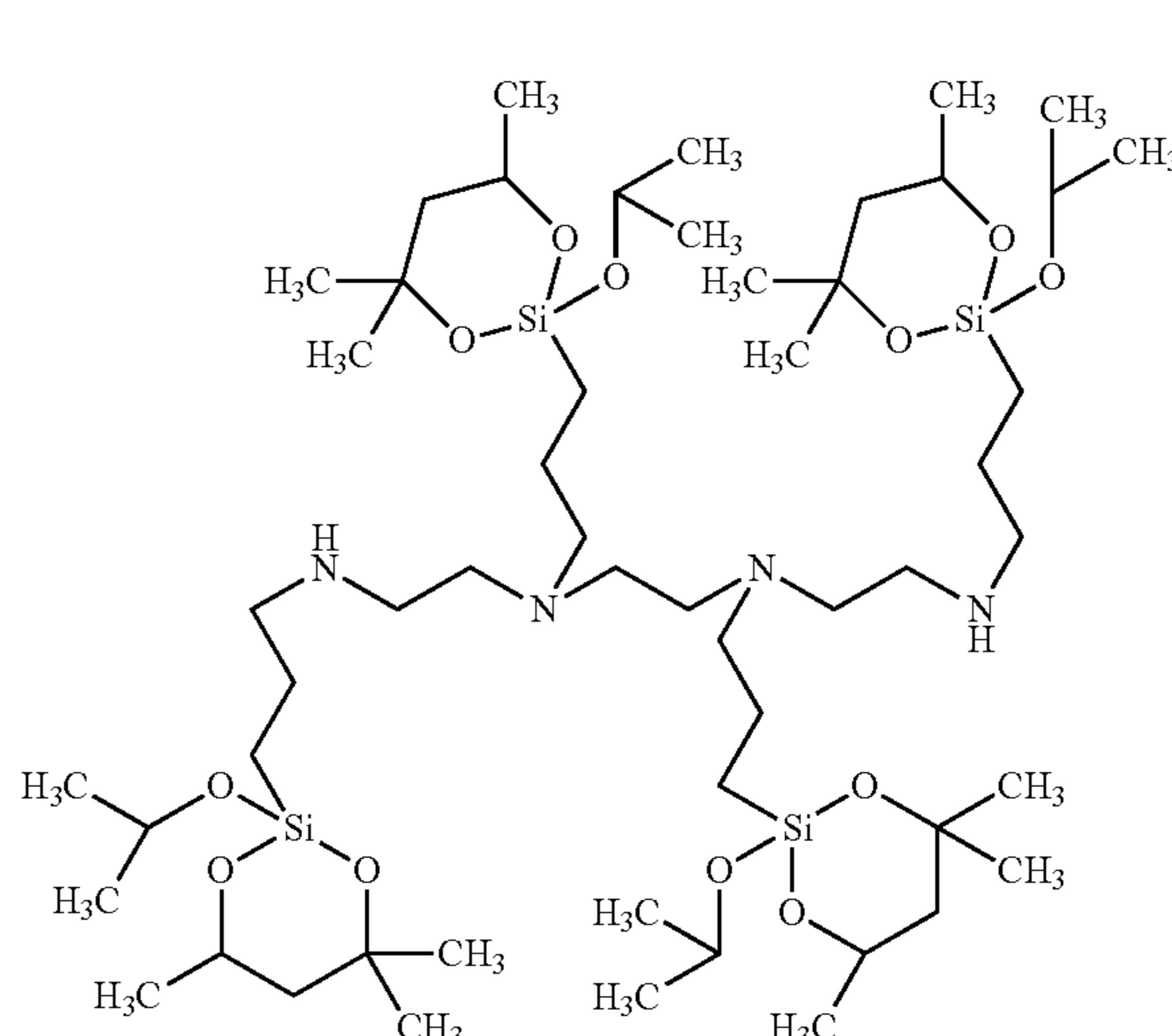
tetrakis-N,N',N'',N'''-[3-(2-methyl-2,4-pentanedialkoxyisopropoxysilyl)-1-propyl] triethylene tetramine;
