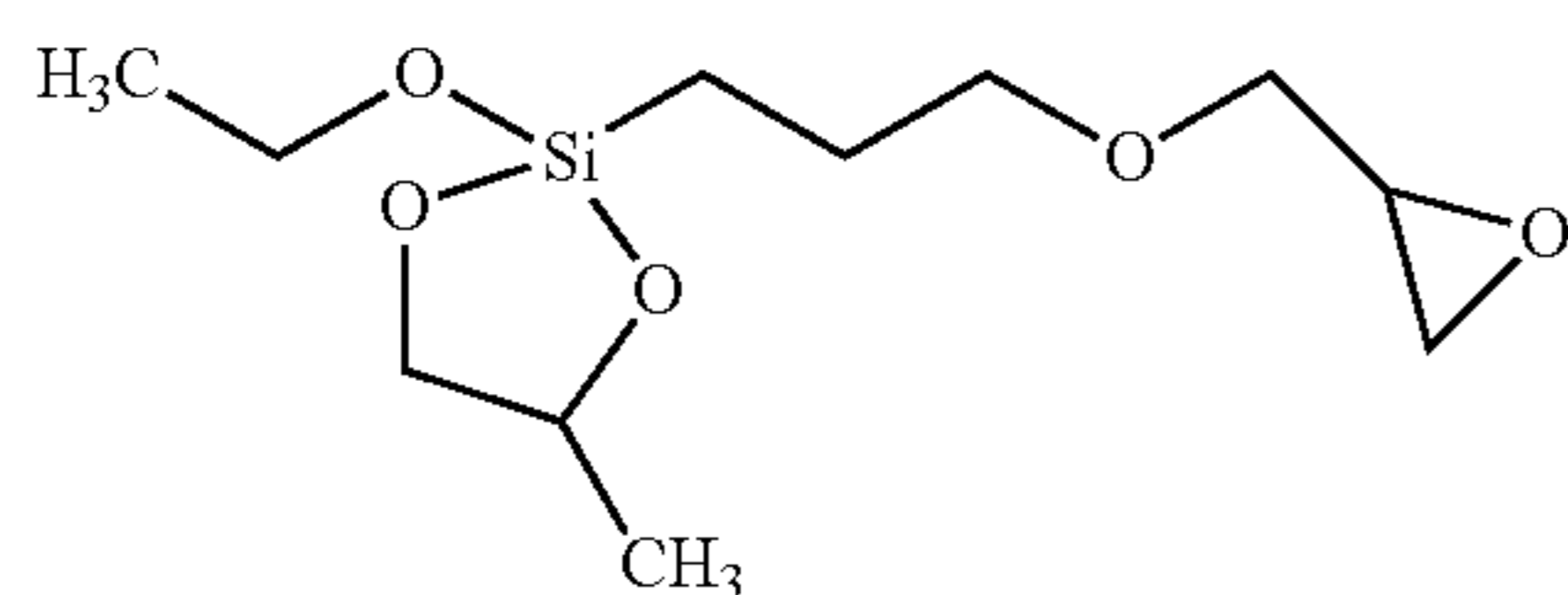
3-(1,2-propanedialkoxyethoxysilyl)-1-propyl glycidyl ether;
