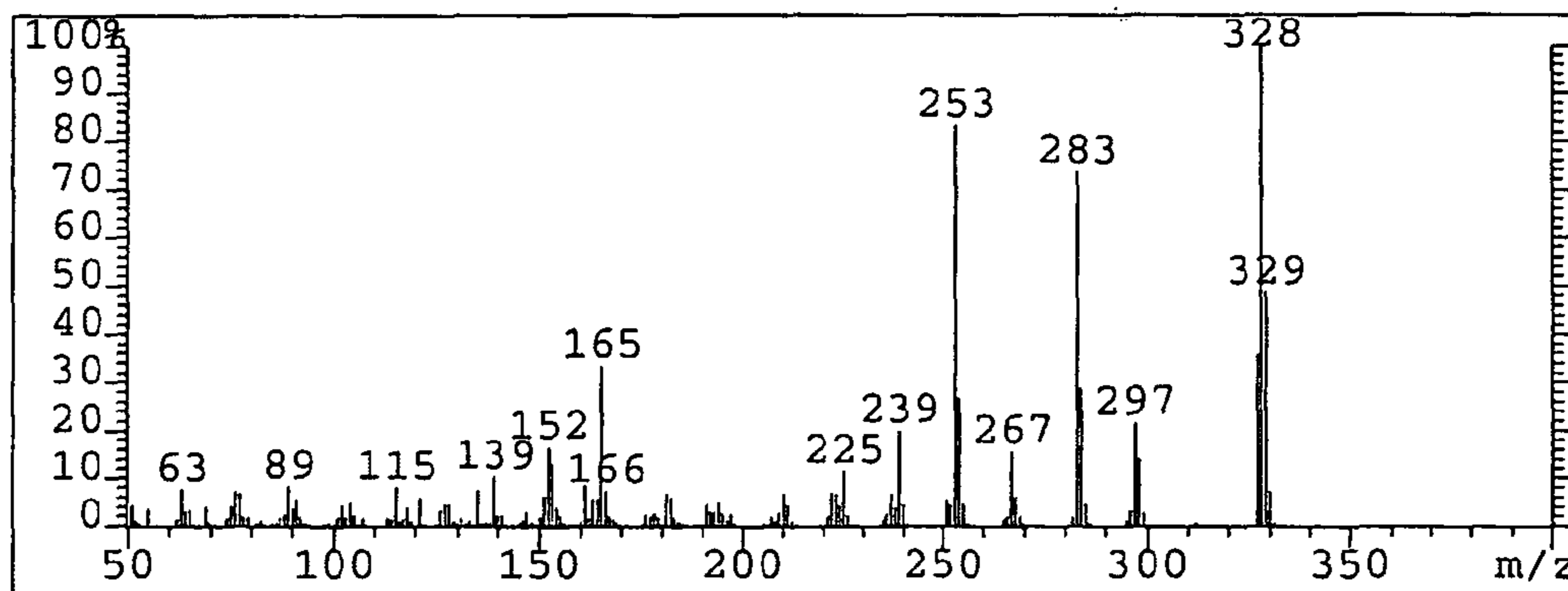
Spectrum - bis-MOM-dehydroequisol
