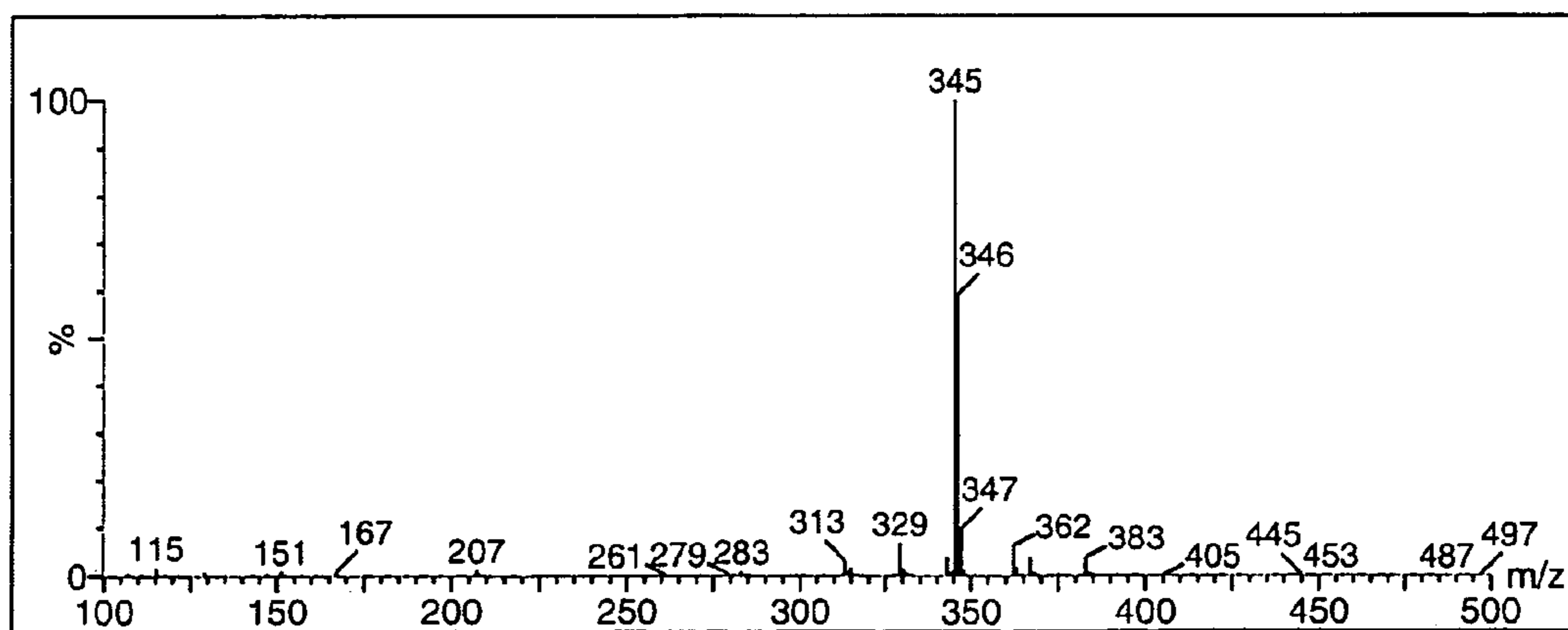
Spectrum - chroman-4-one
