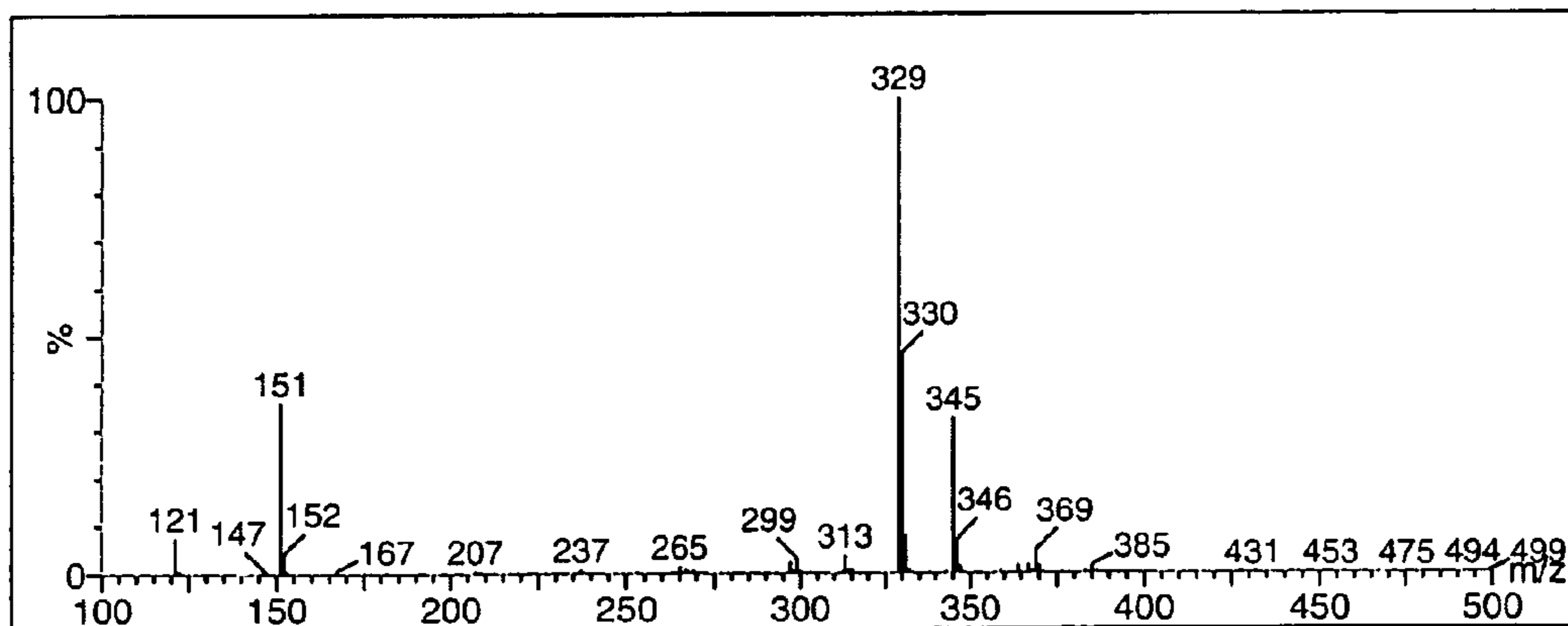
Spectrum - chroman-ol
