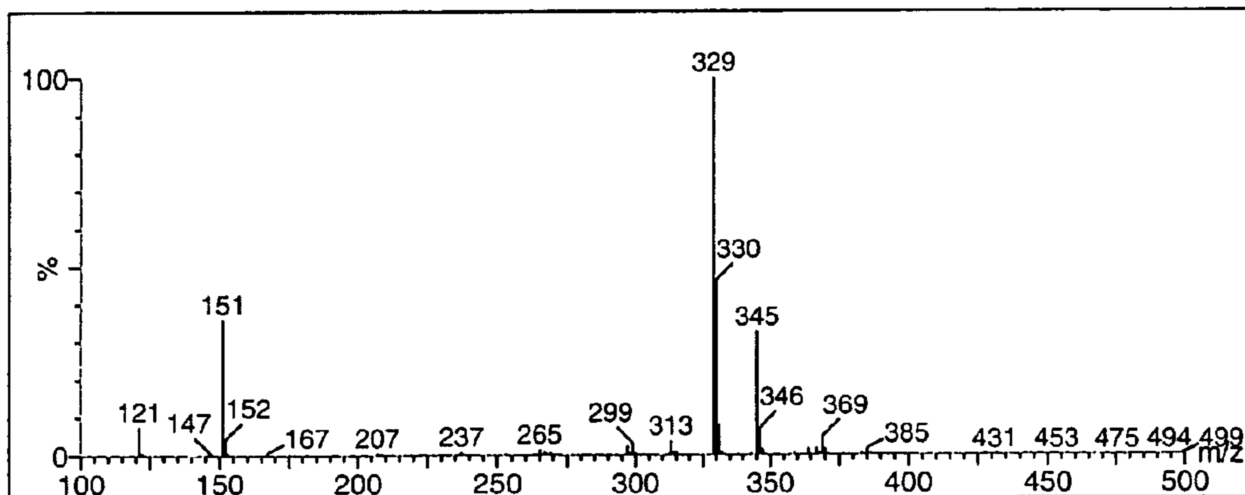
Spectrum - chroman-ol
