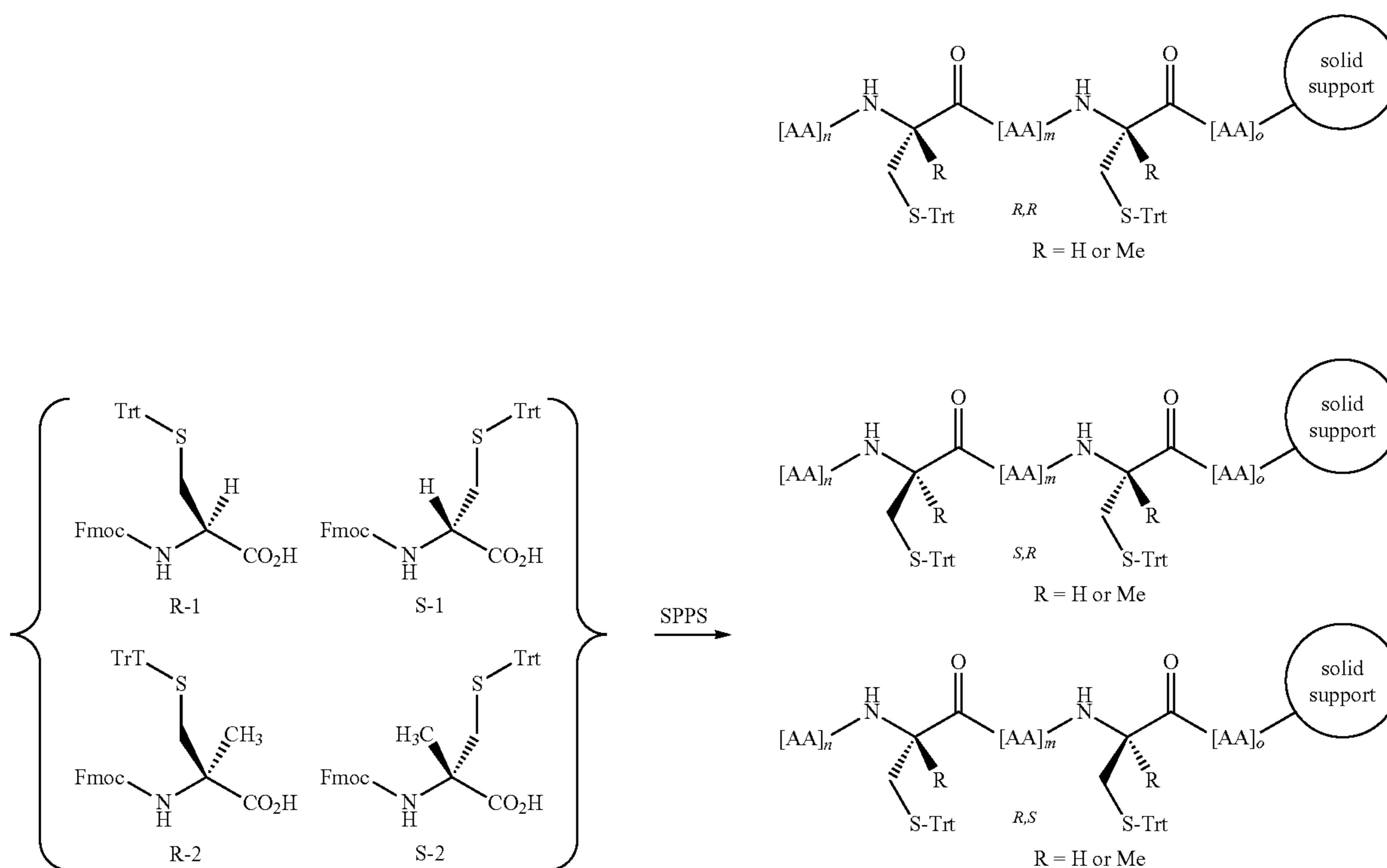
Synthetic Scheme 1:
