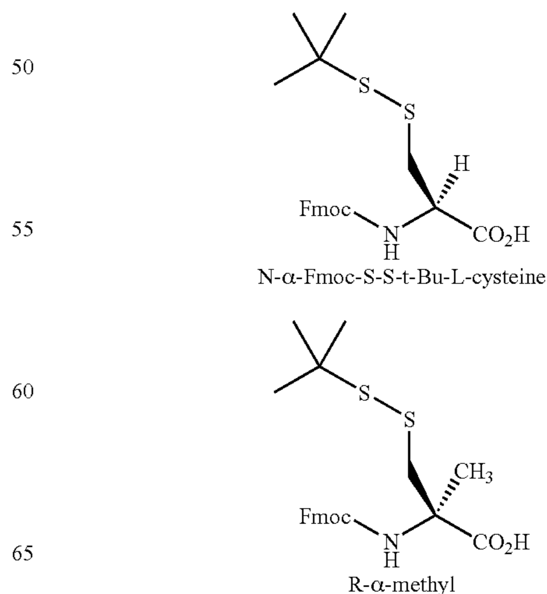
(Formula IIa)
