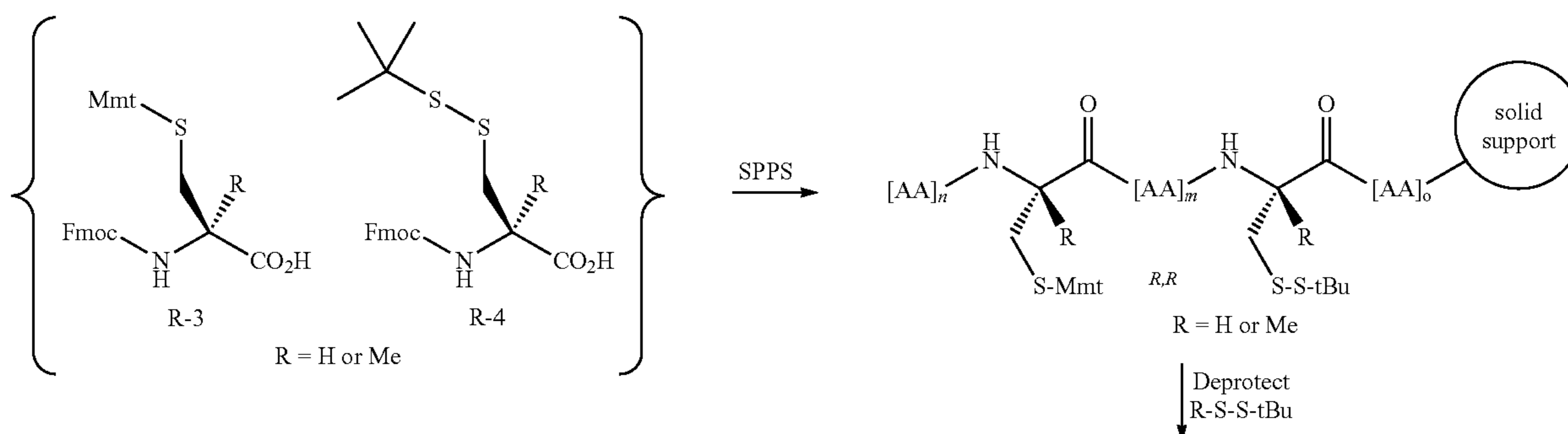
Synthetic Scheme 3:
