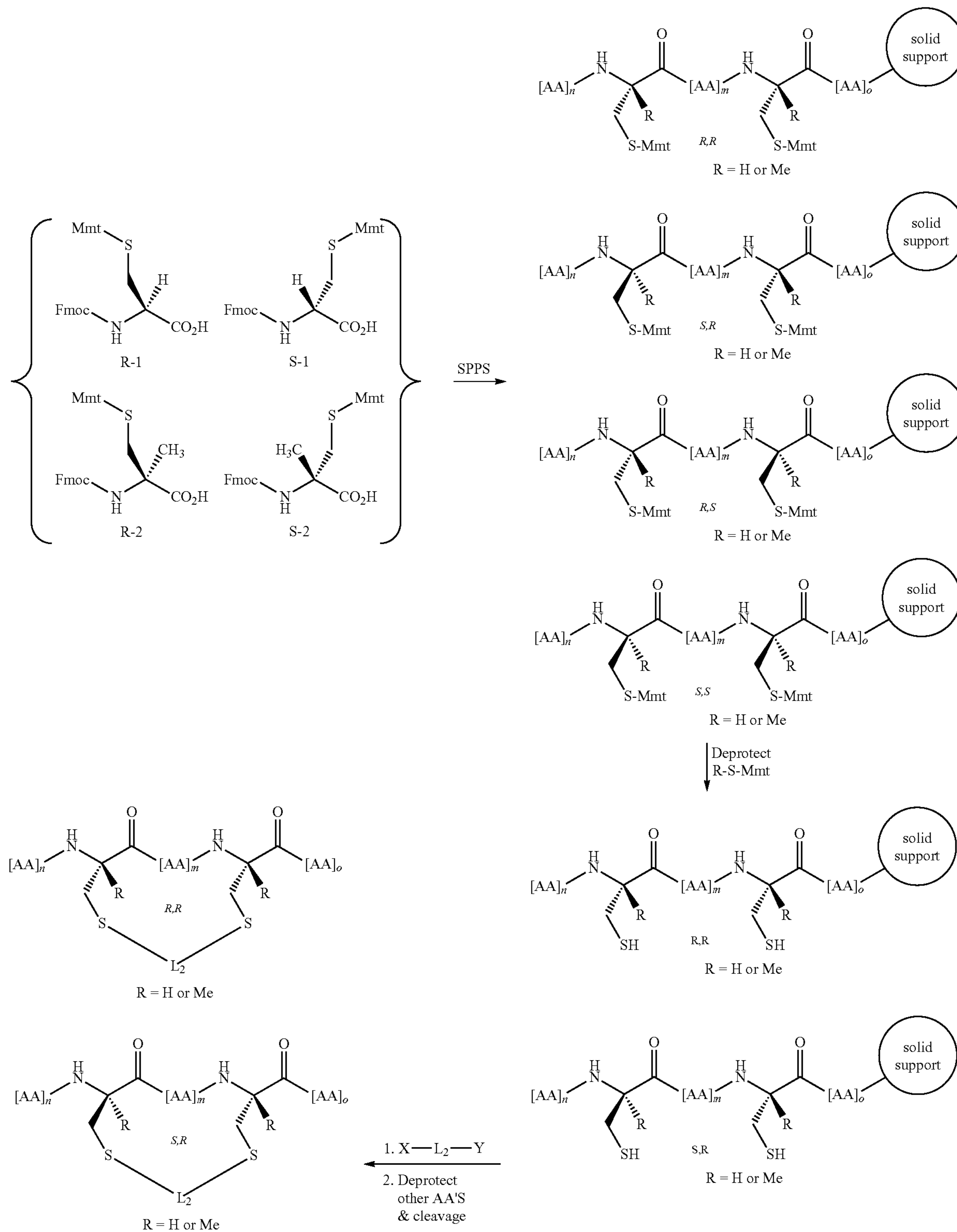
Synthetic Scheme 2:
