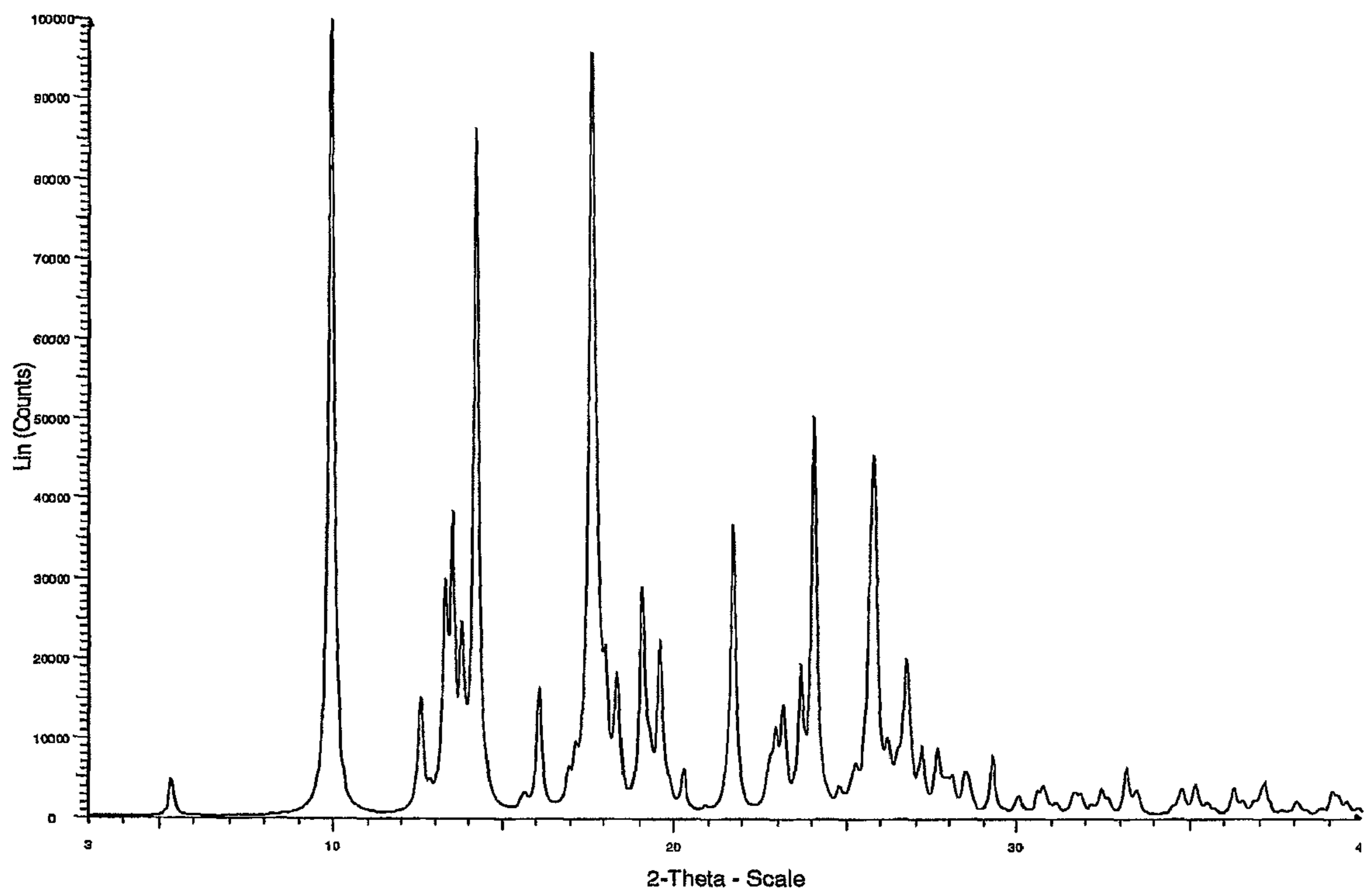
Form A calculated PXRD
