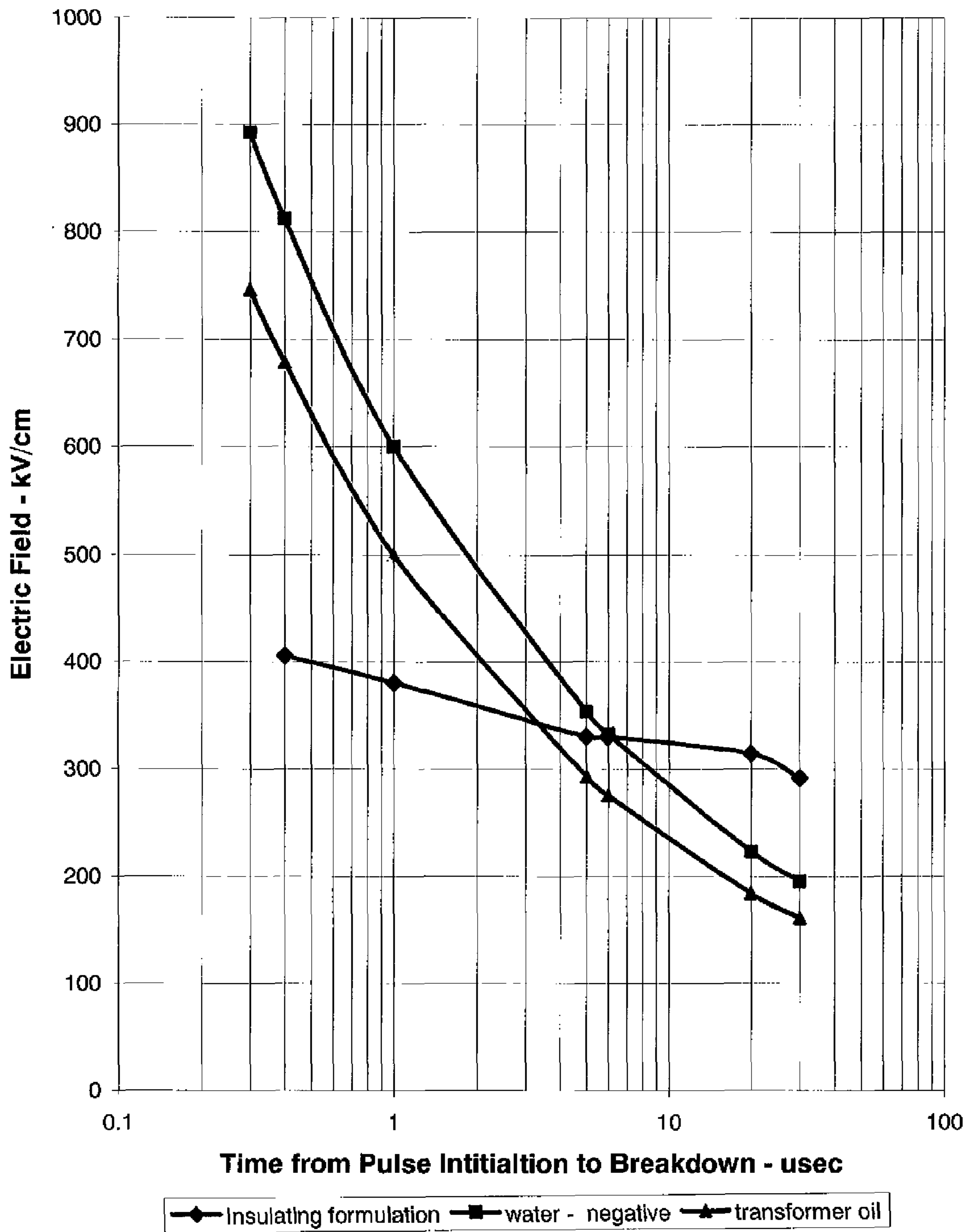
Dielectric Strength vs. Delay To Breakdown Figure 32
