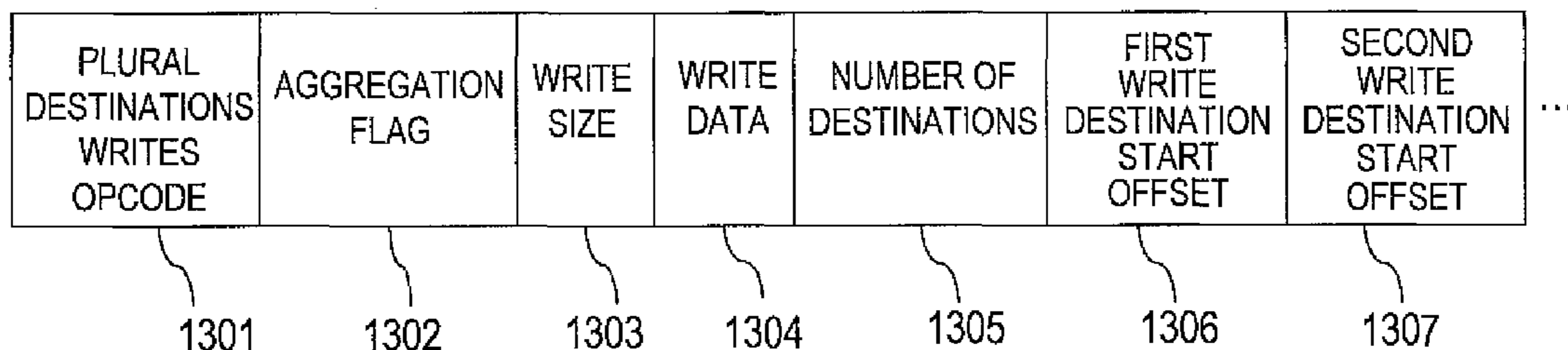
FORMAT OF PLURAL DESTINATIONS WRITE COMMAND 1300
