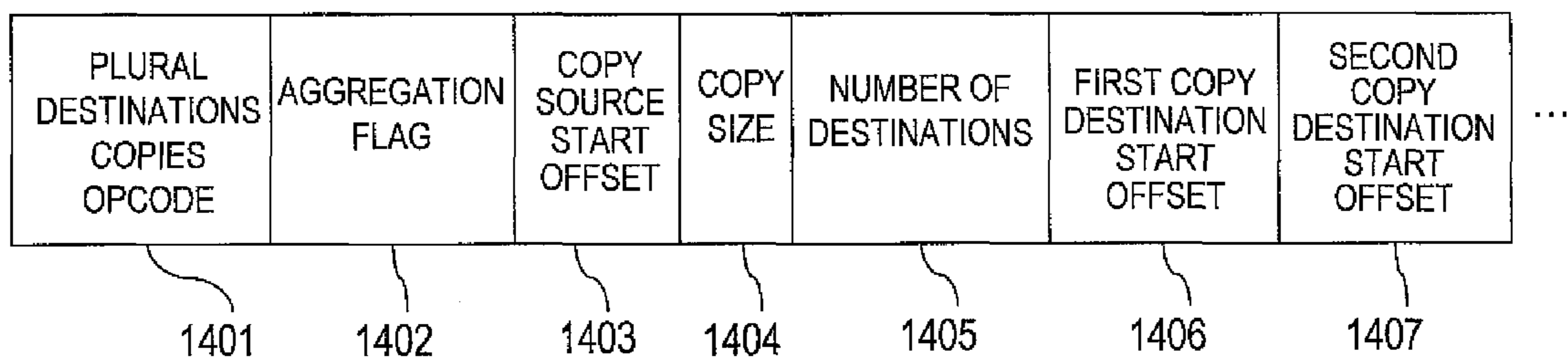
FORMAT OF PLURAL DESTINATIONS EXPANSION COPY COMMAND 1400
