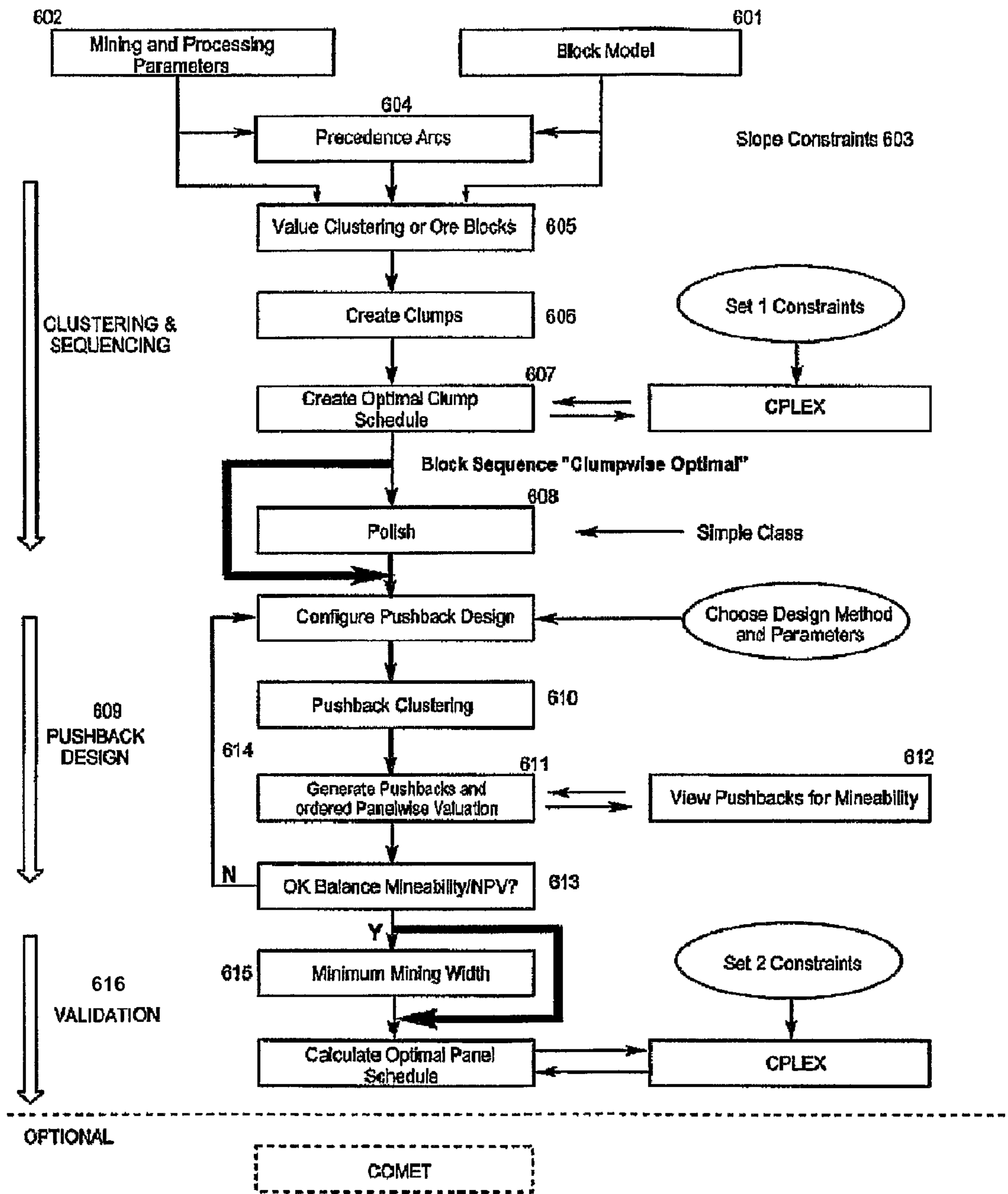
Figure 6 KlumpKing Top-Level Flow Chart
