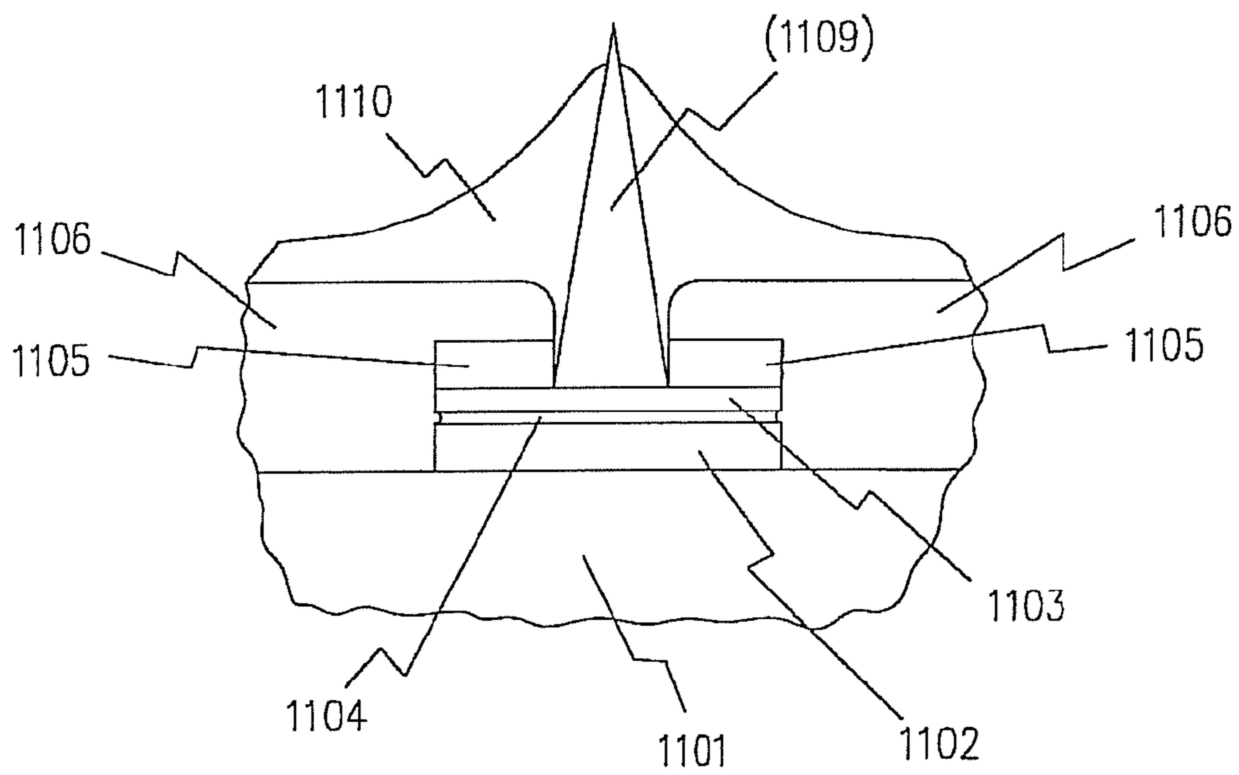
FIGURE 11b ELECTRODES
