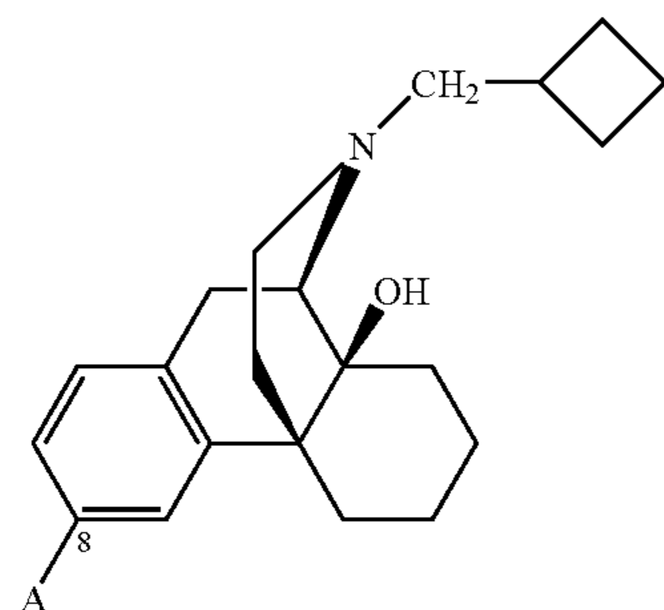
Butorphanol core
