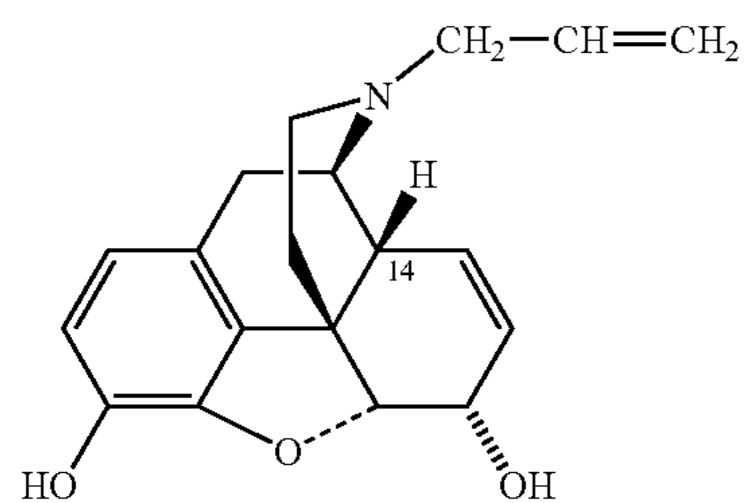
Nalorphine
