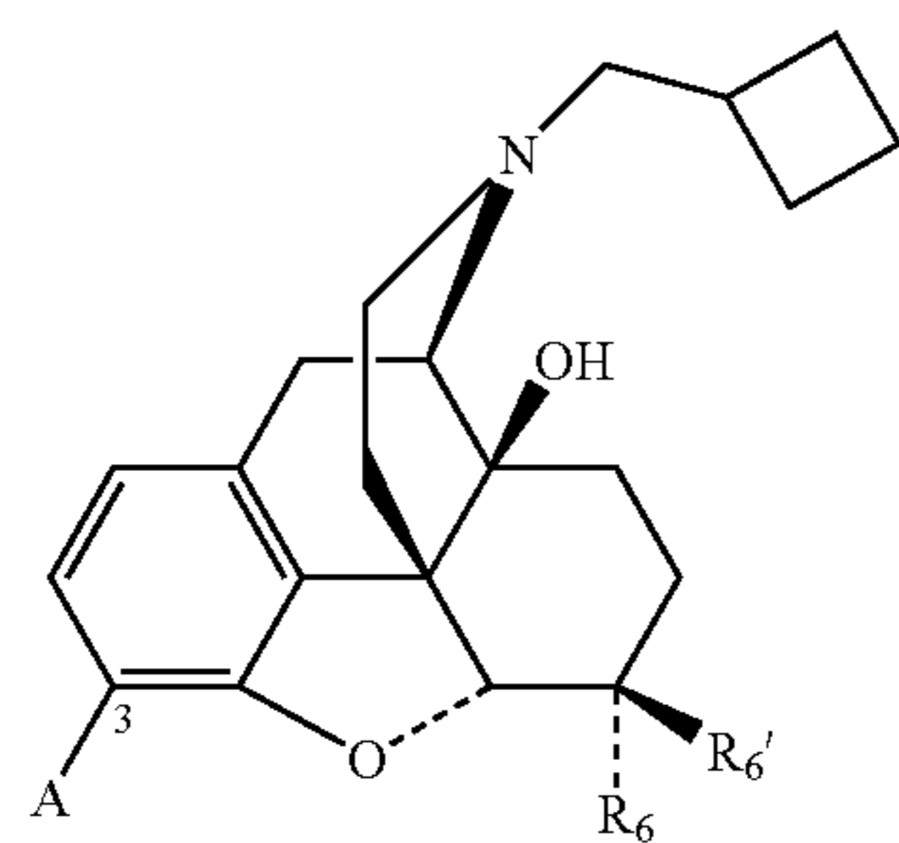
Nalbuphine core
