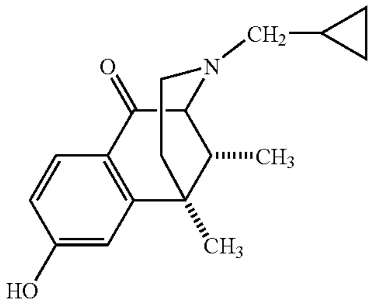
Ketocyclazocine
