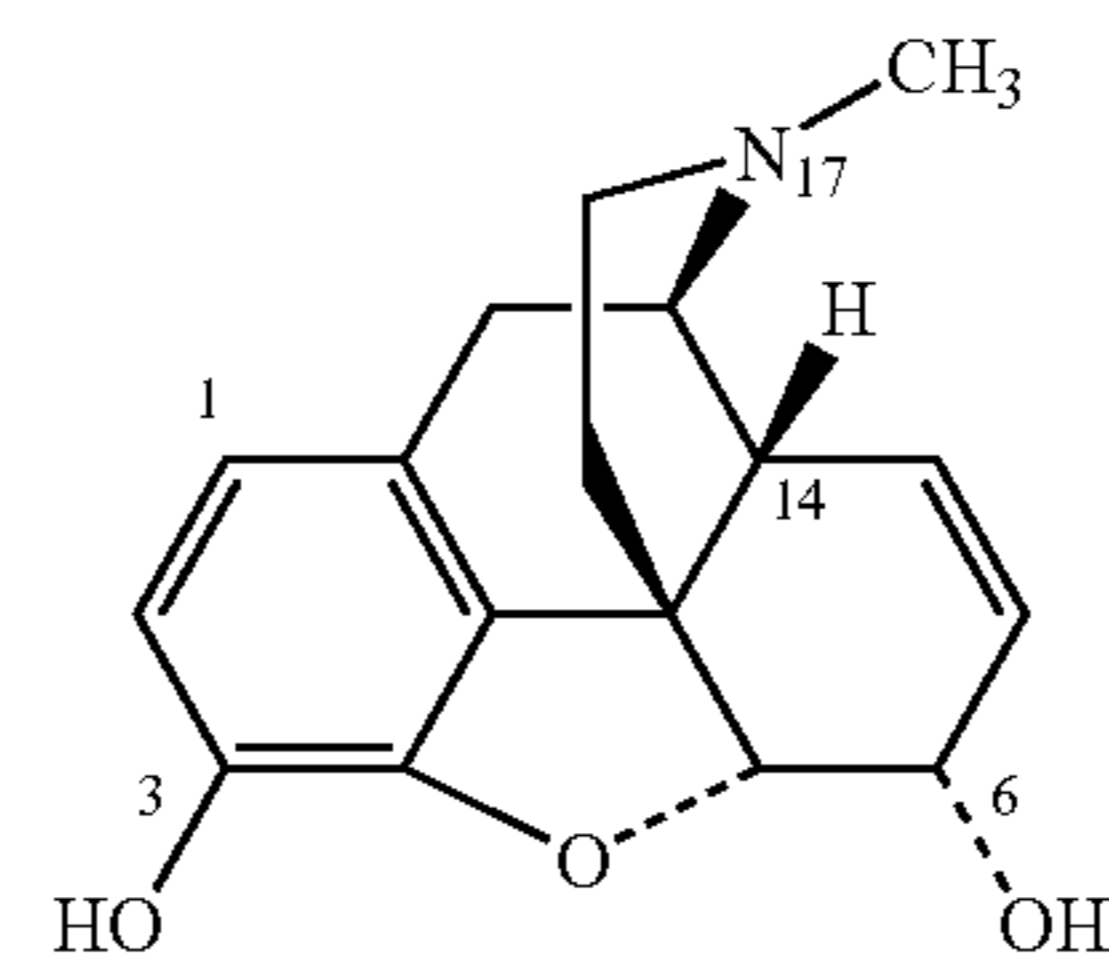
Morphine
