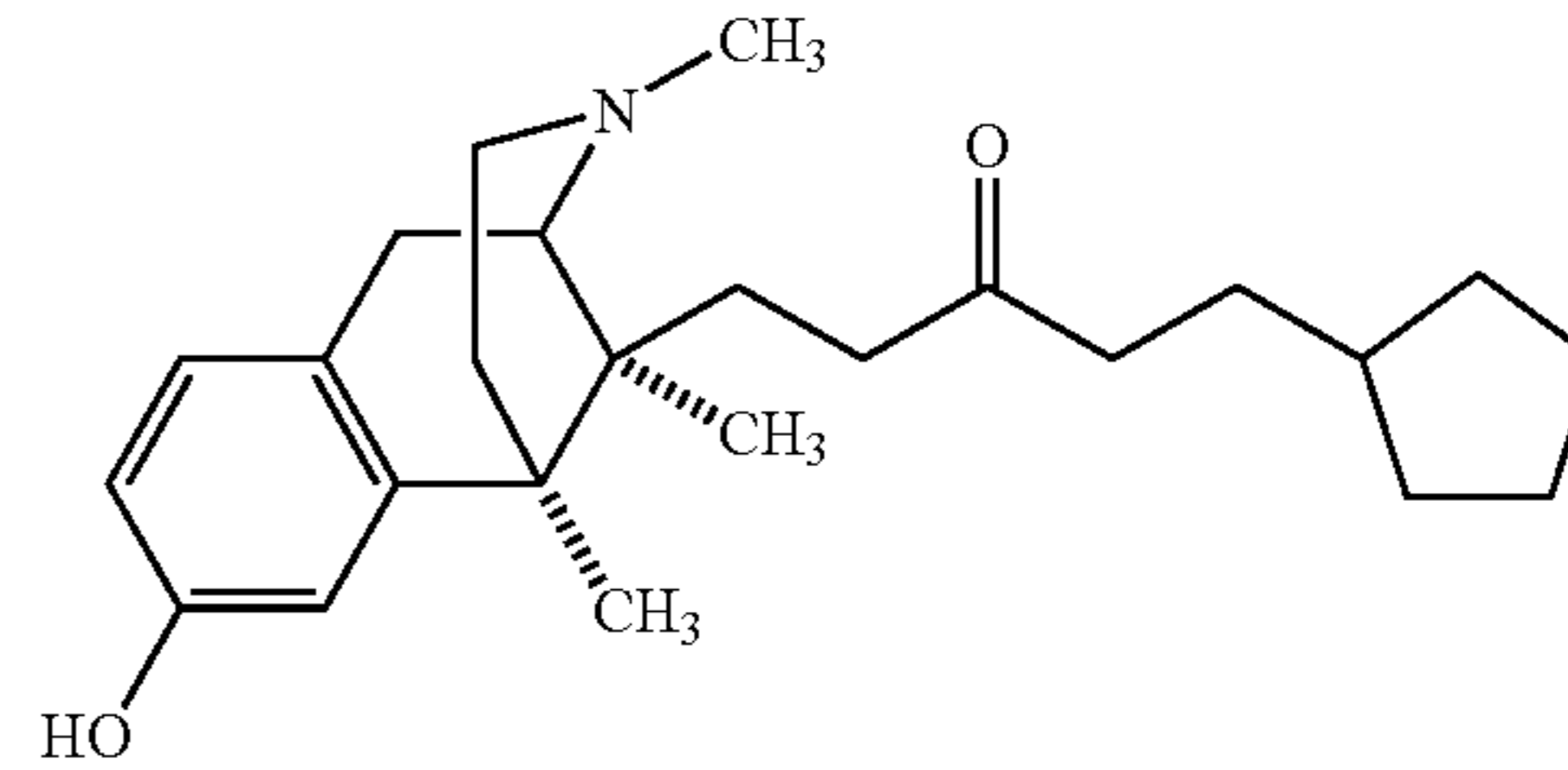
WIN 44,441
