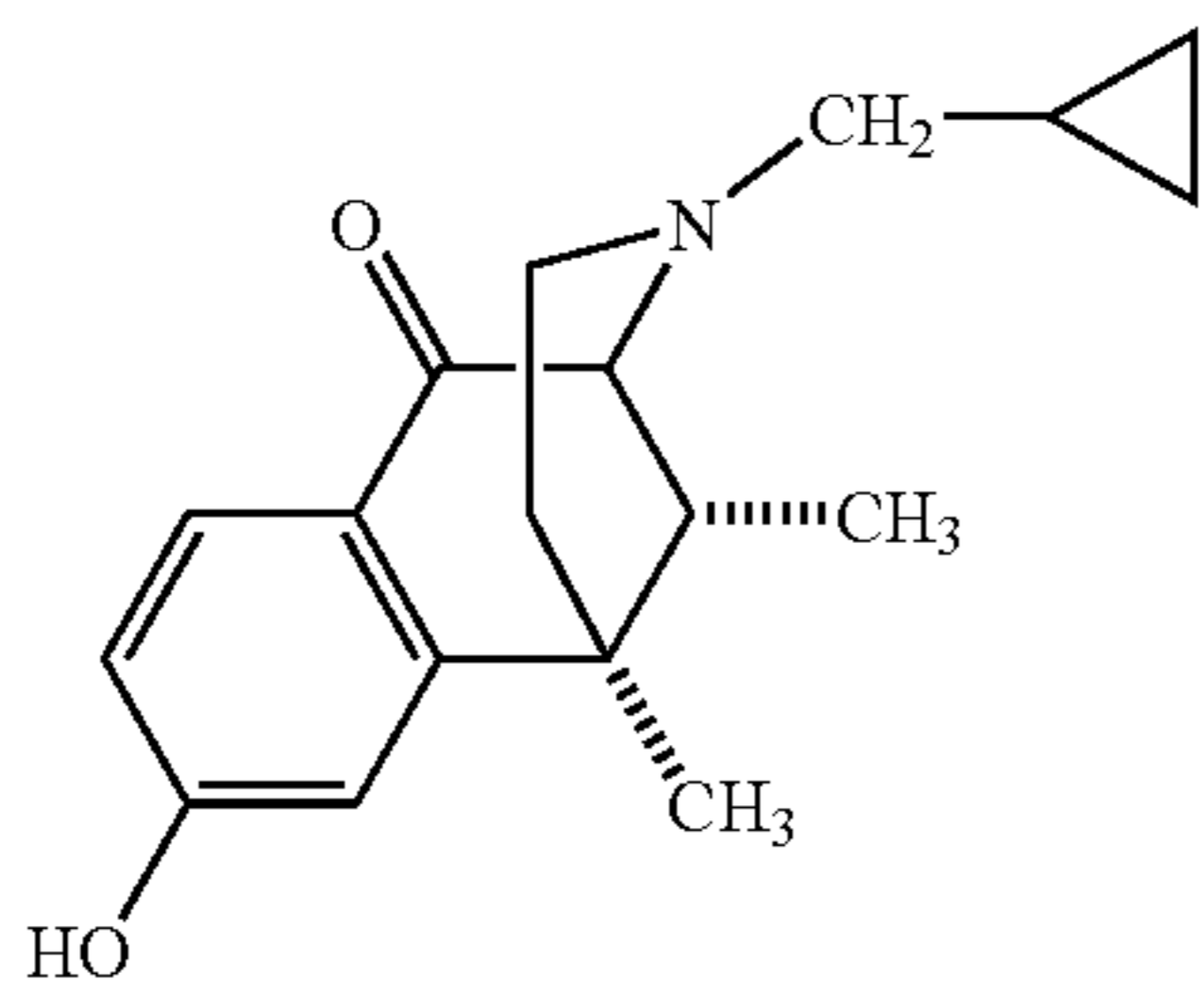
Ketocyclazocine
