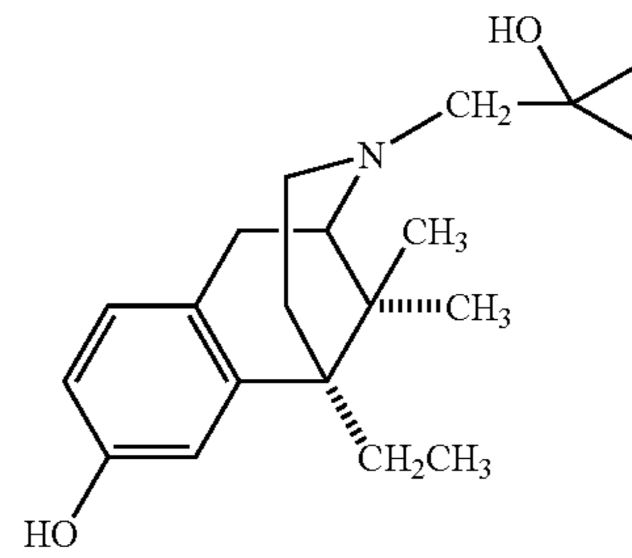
Bremazocine
