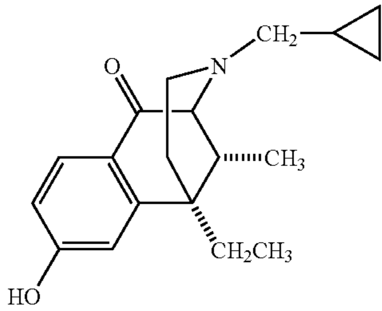
Ketocyclazocine
