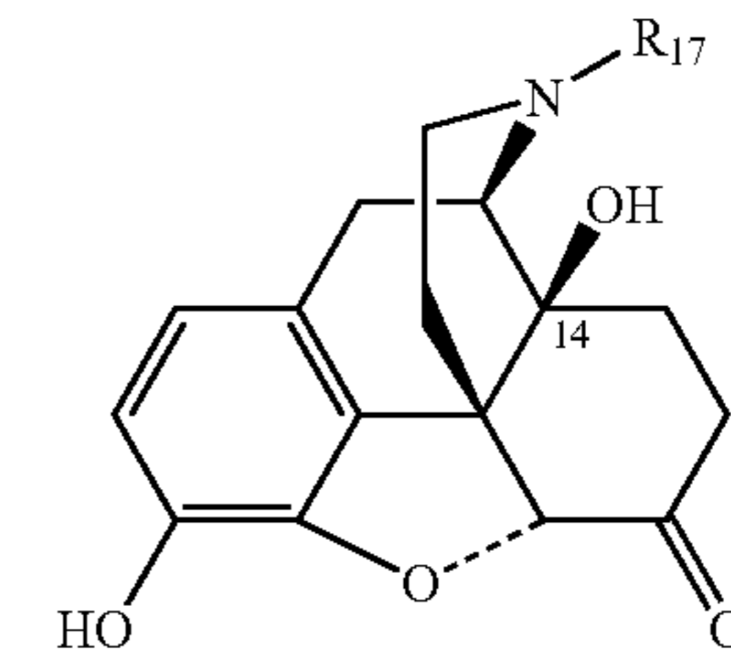
Morphine
