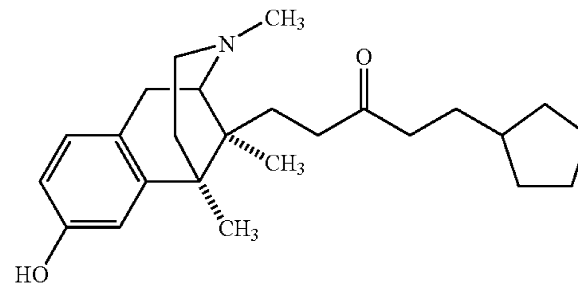
WIN 44,441
