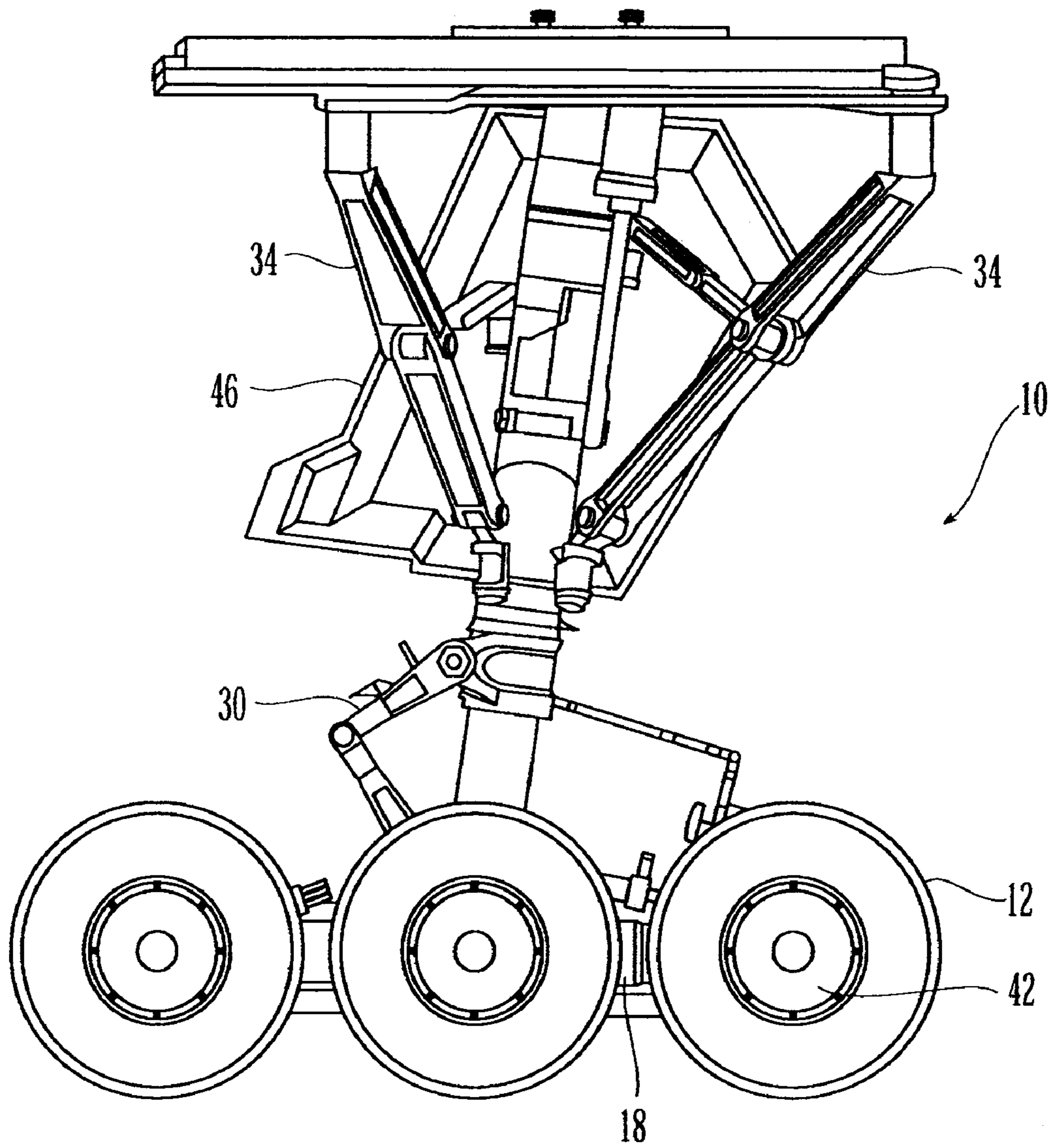
Fig. 1 (Prior Art)
