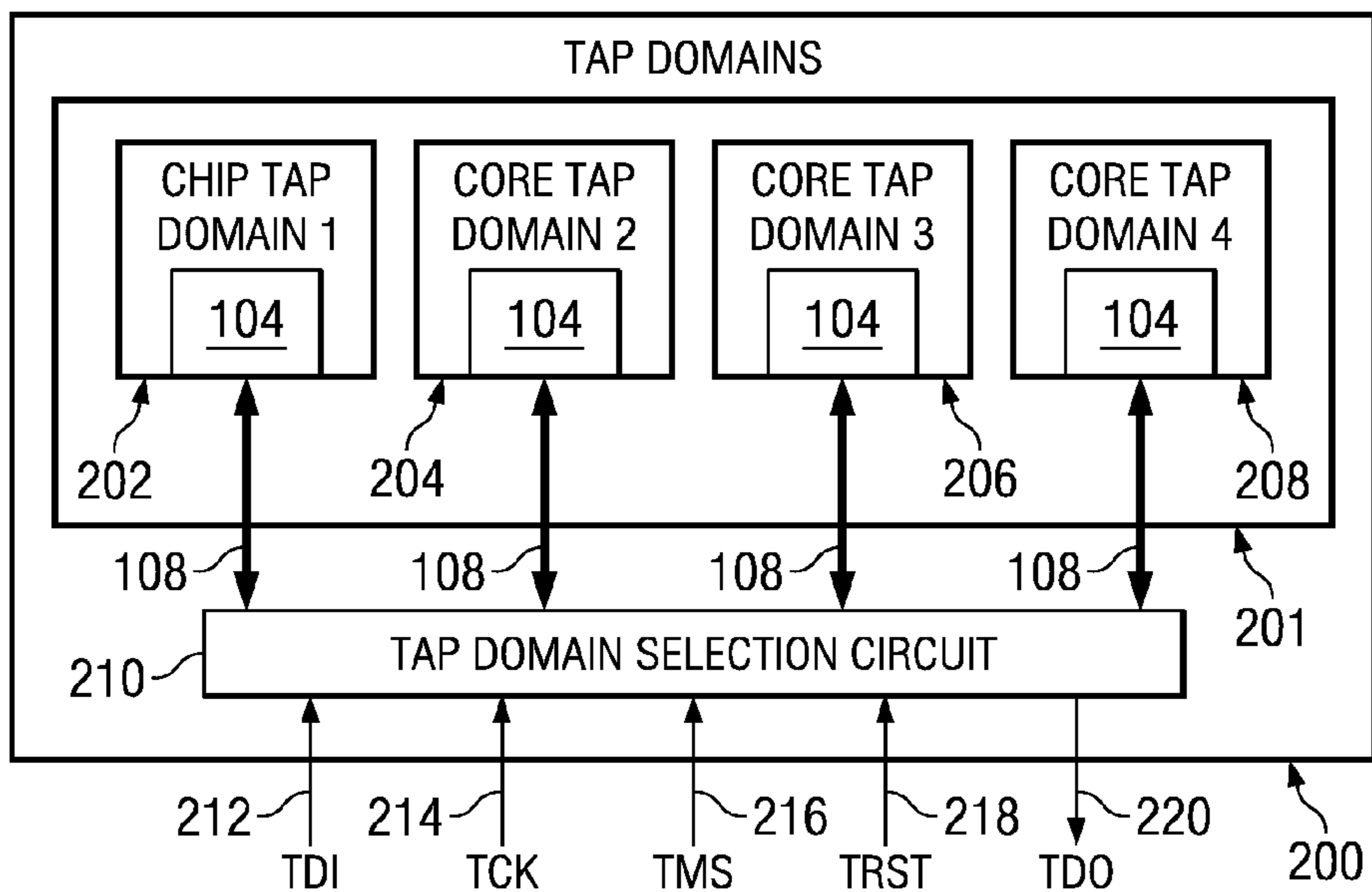
FIG. 2 (PRIOR ART)
