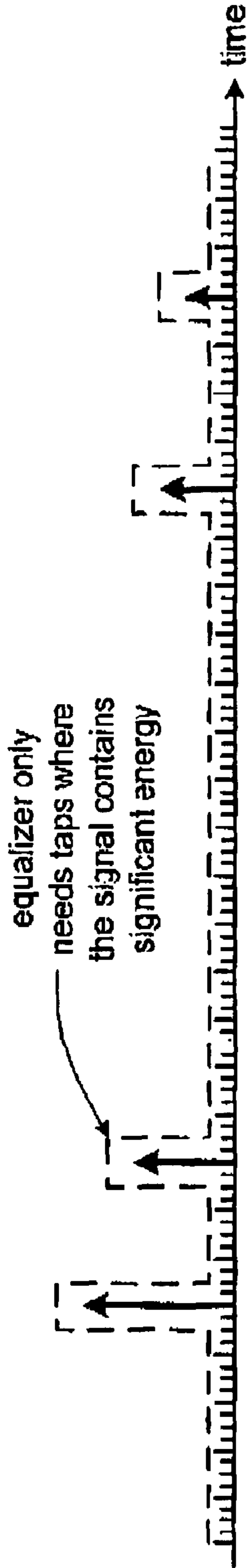
Figure 7 sparse channel
