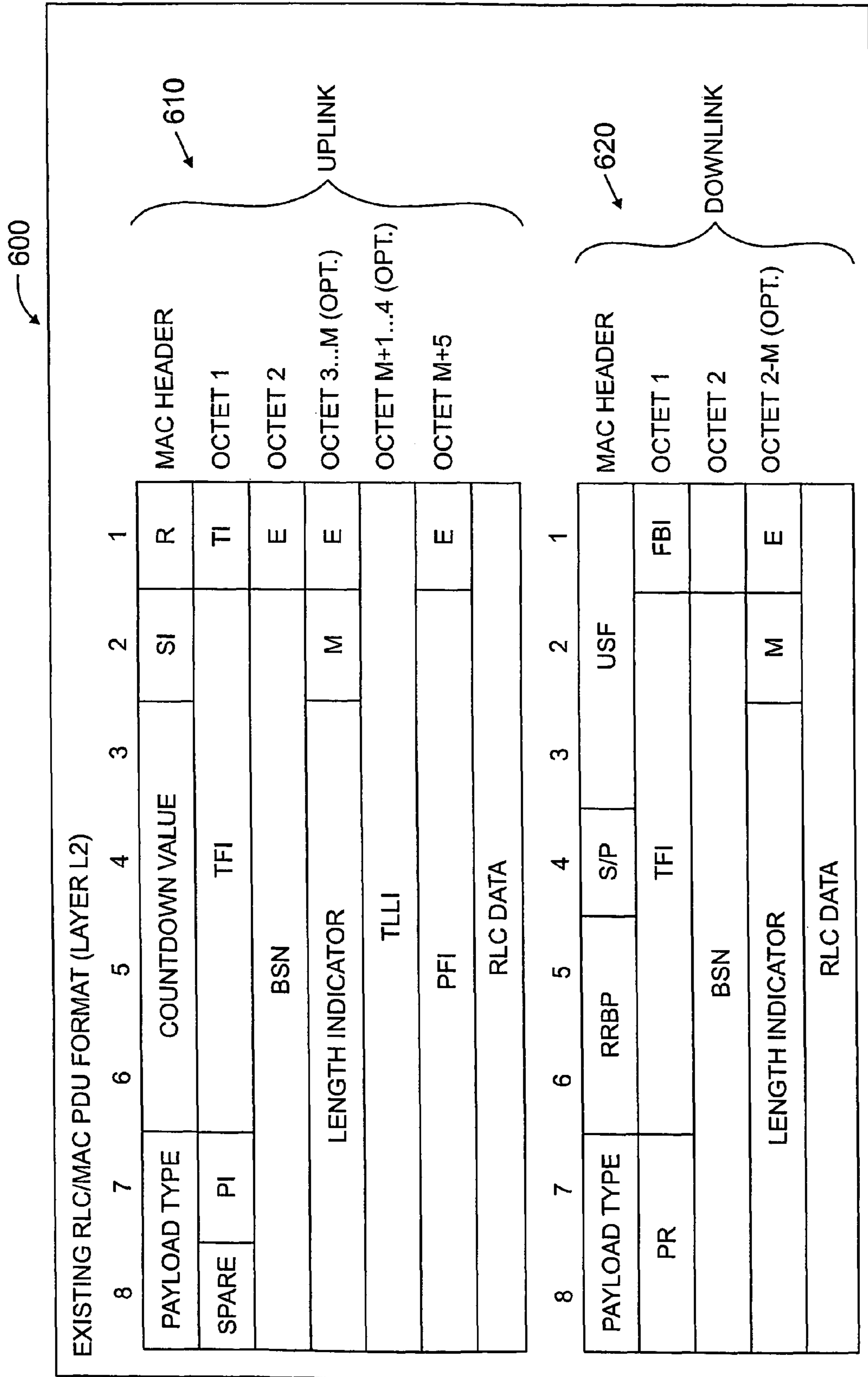
FIG. 6 (PRIOR ART)
