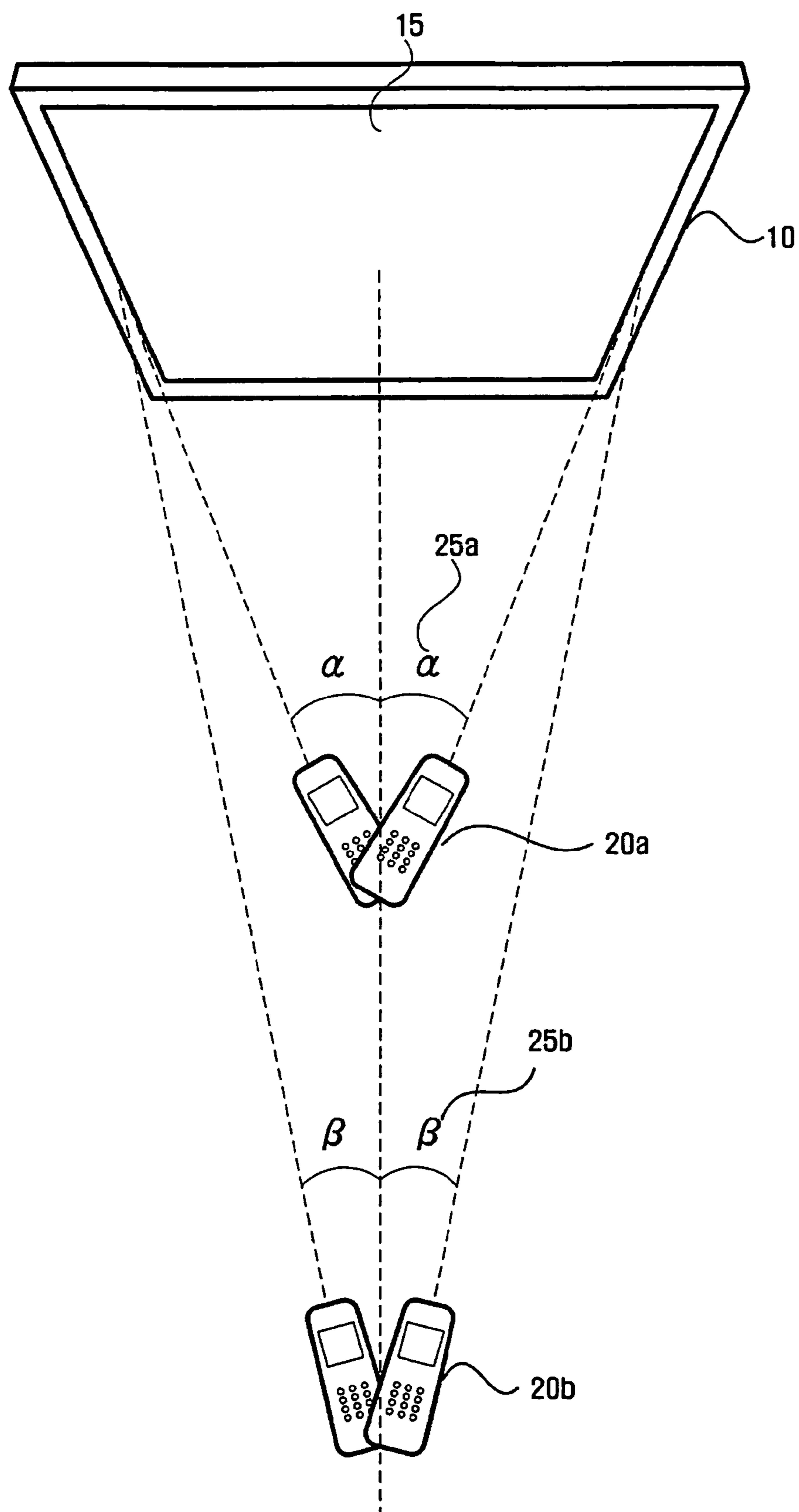
FIG. 1 (PRIOR ART)
