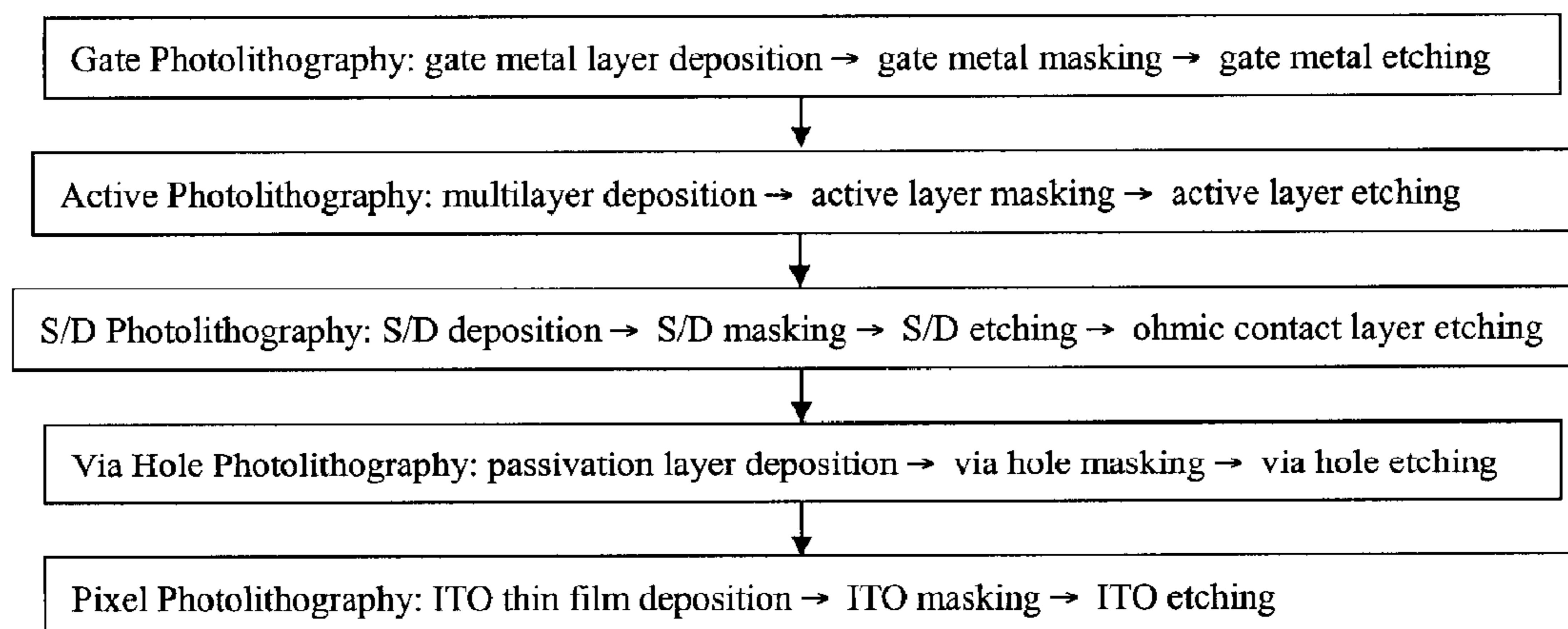
FIG. 2 (PRIOR ART)
