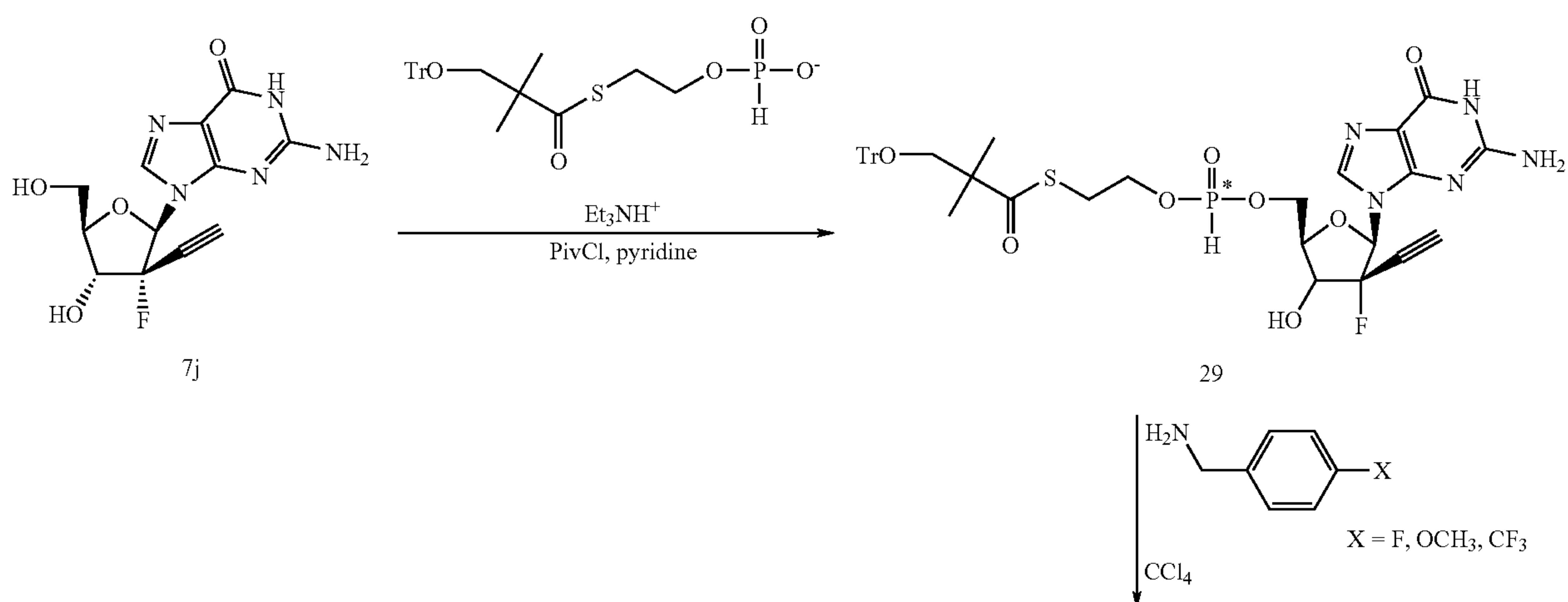
-Scheme 6-
