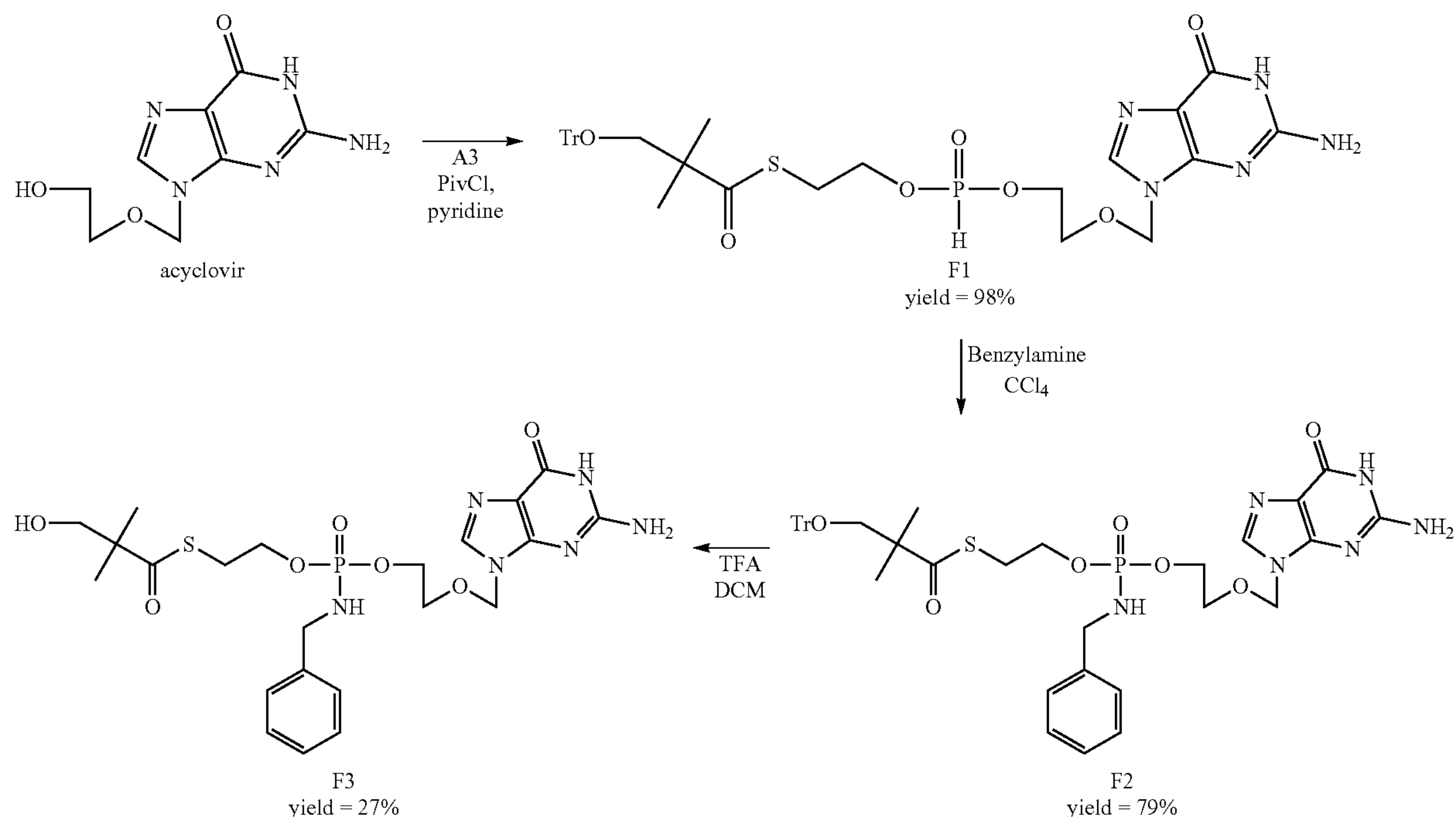
Scheme 1
