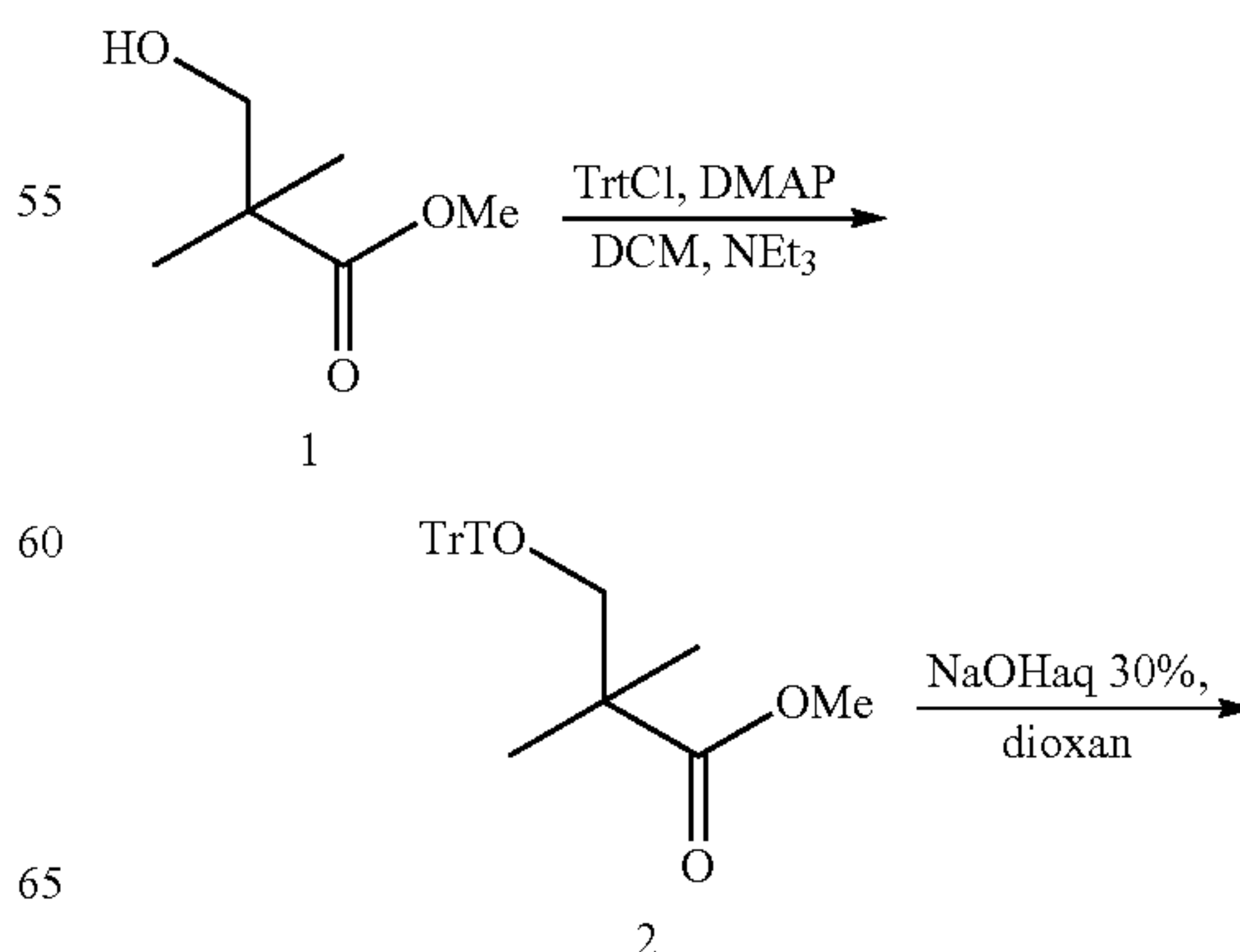
Scheme B1: Synthesis of the H-phosphonate monoester reagent
