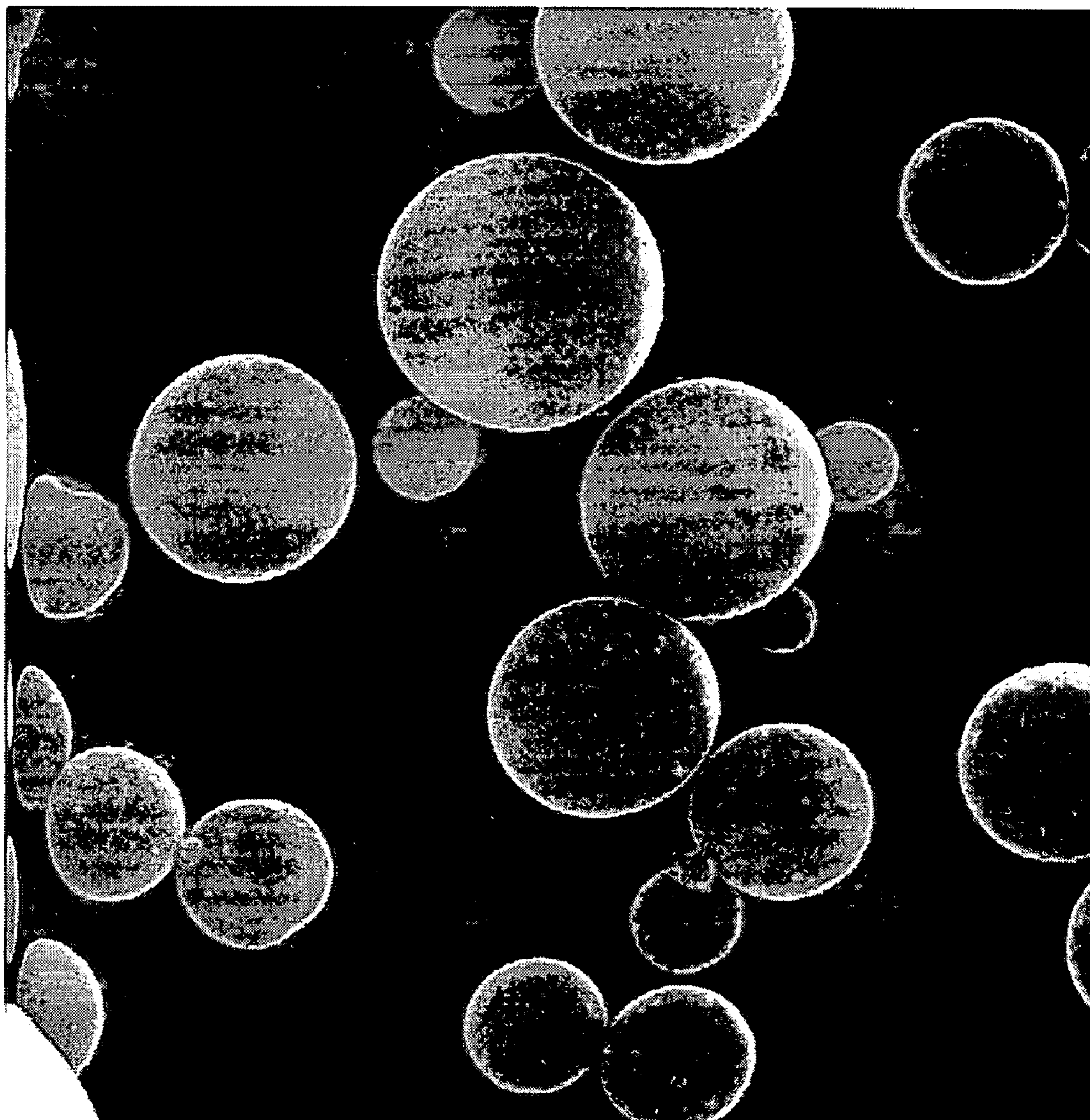
Figure 1. SEM Picture of Particles SP-5 taken under 5000x magnification.
