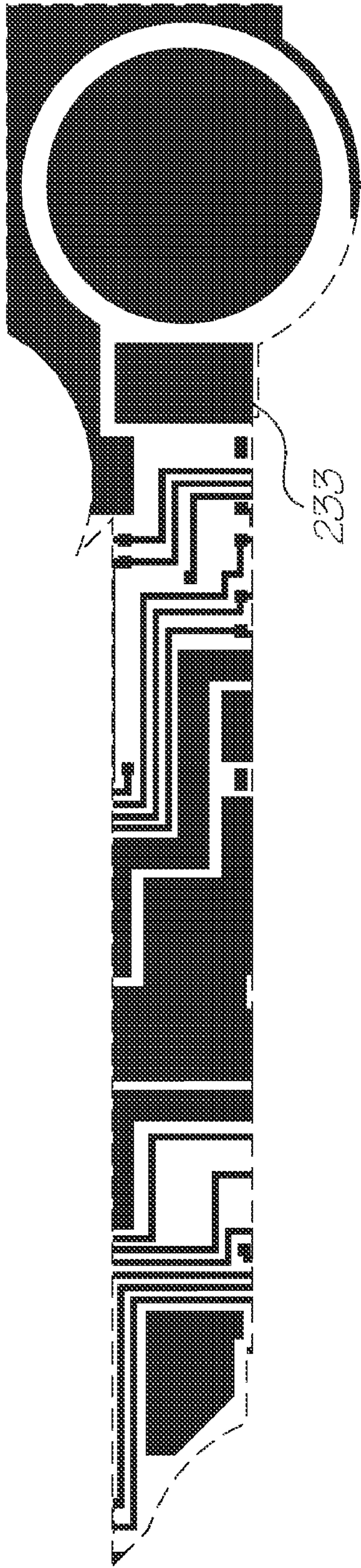
Metal 2 mask
