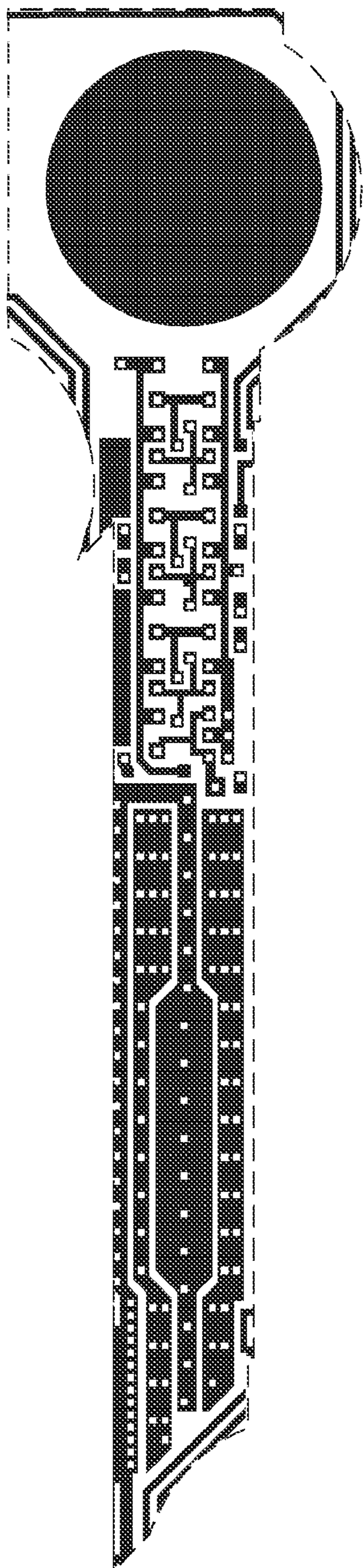
Metal 1 mask
