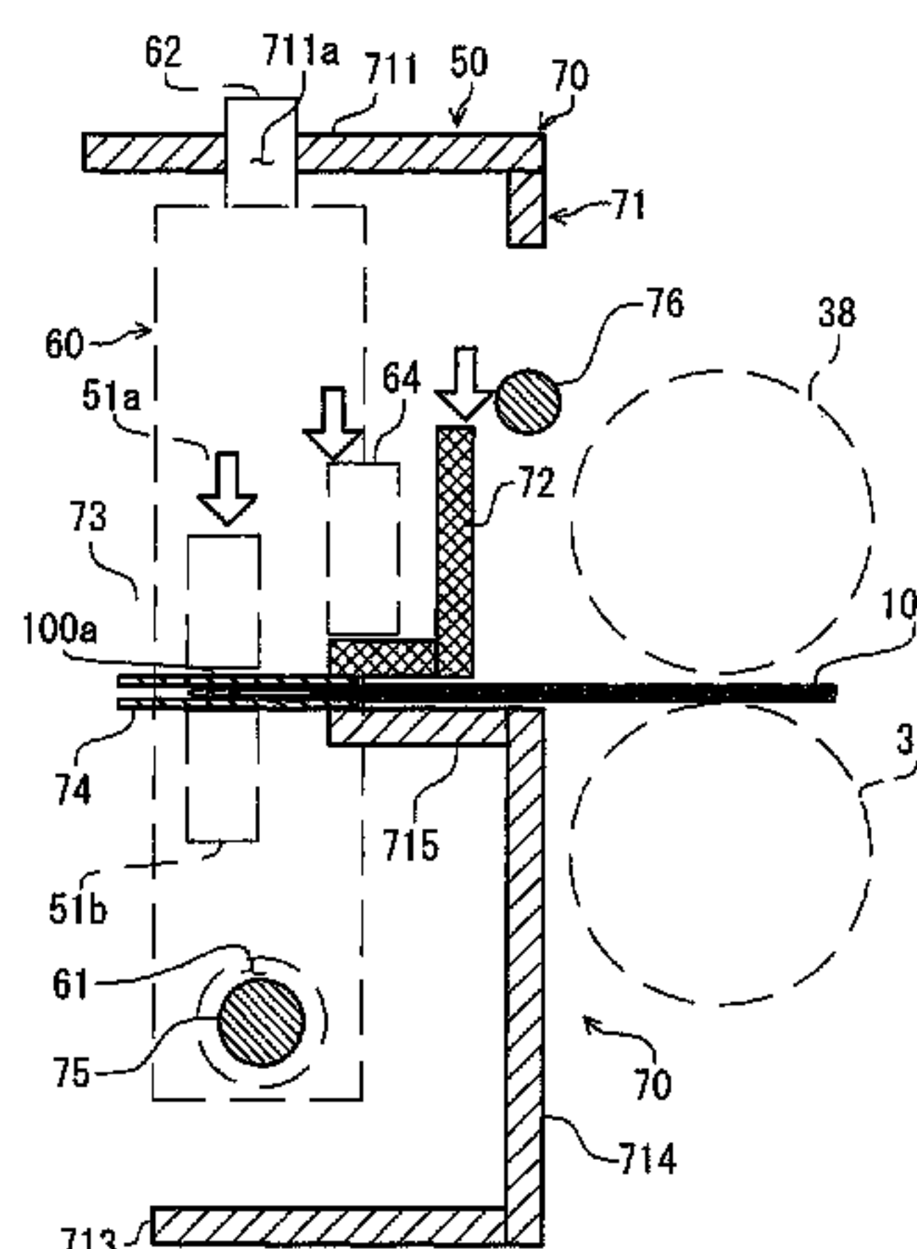
AT MOVEMENT OF ROLLER UNIT (AT FOLD LINE REINFORCING OPERATION)
